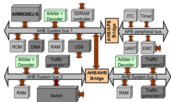
Figure 7. SoC platform
