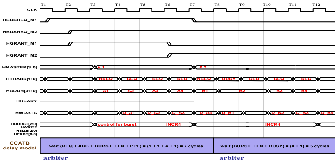
Figure 5. Reference AMBA2 call sequence
