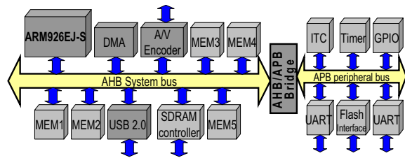
Figure 6. SoC Multimedia Subsystem
