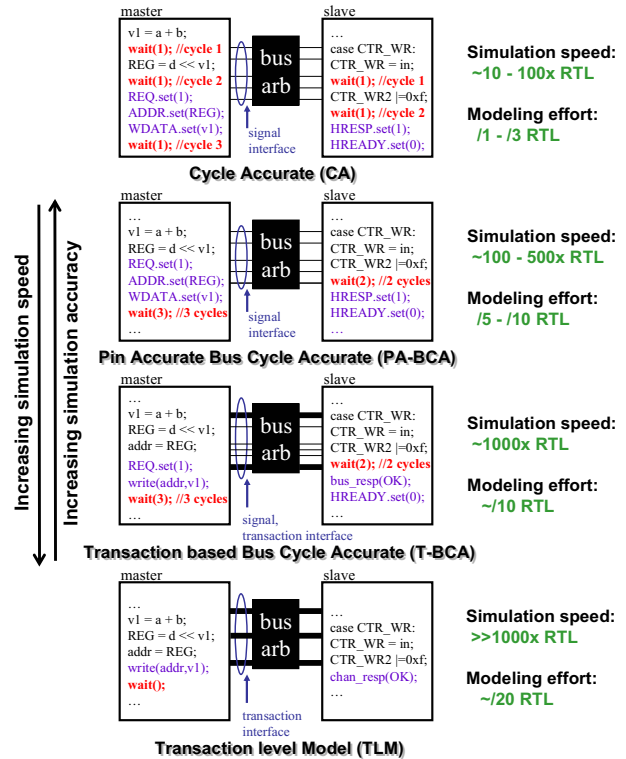
Figure 3. Modeling Abstractions for Communication Architecture Exploration
