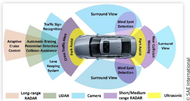
FIGURE 1 State-of-the-art ADAS and different sensors [24].
