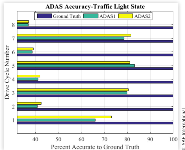
FIGURE 13 ADAS percent accurate to ground truth - traffic light state
