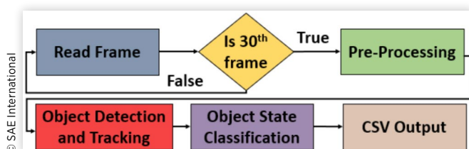
FIGURE 6 ADAS prediction pipeline
