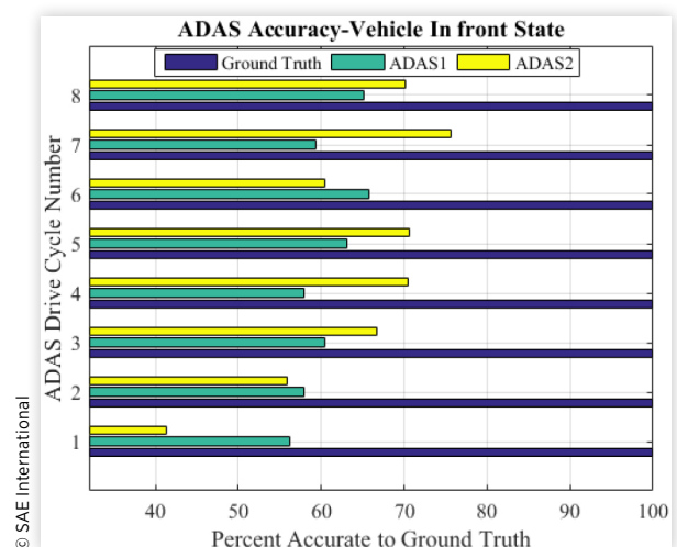
FIGURE 12 ADAS percent accurate to ground truth - vehicle in front state
