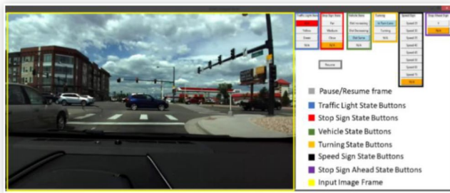
FIGURE 5 Ground Truth Development App
