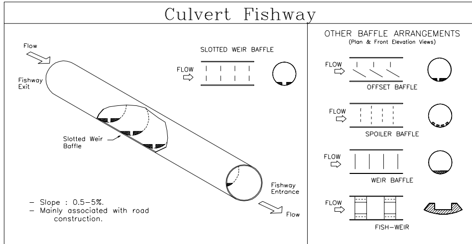
Figure 2.4b Culvert fishway.
