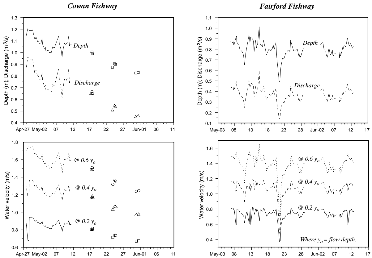
Figure 7.3 Depth, discharge and velocity profiles for Cowan (1985) and Fairford (1987) fishways.
