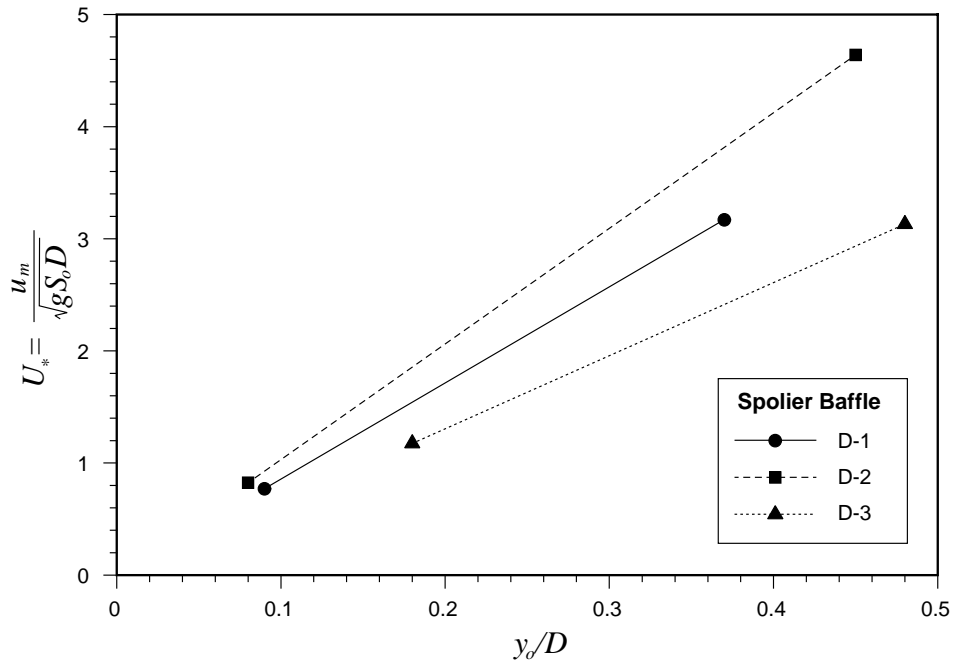
Figure 5.15 Spoiler baffle dimensionless velocity scales.
