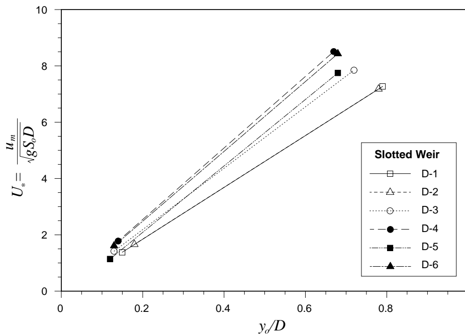
Figure 5.12 Slotted weir baffle dimensionless velocity scales.
