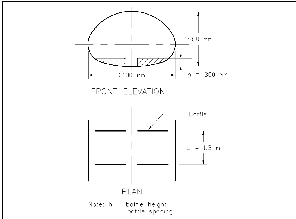
Figure 8.3 Slotted weir culvert fishway for Altrude Creek.
