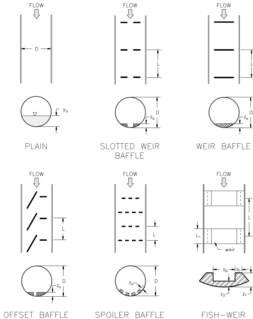
Figure 5.6 Culvert fishways - baffle and weir arrangements.
