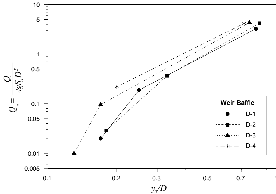
Figure 5.9 Weir baffle dimensionless discharge curves.
