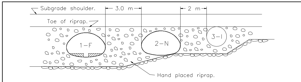
Figure 8.1 Altrude Creek culverts - end view.
