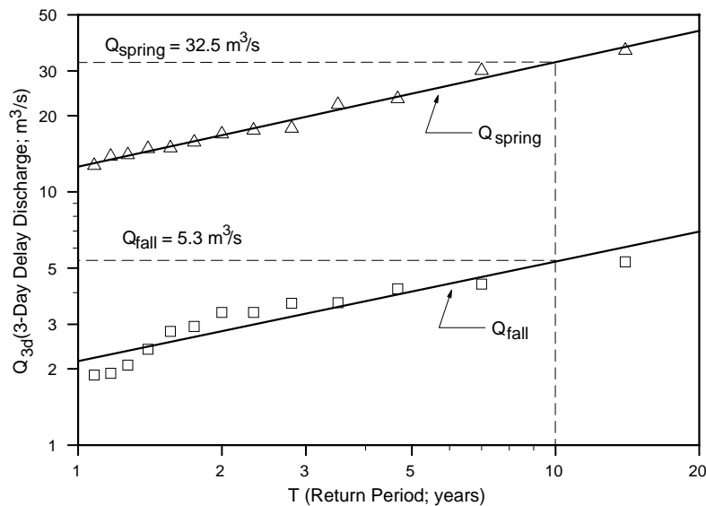
Figure 4.1 Redearth Creek frequency curves (1974-86)
