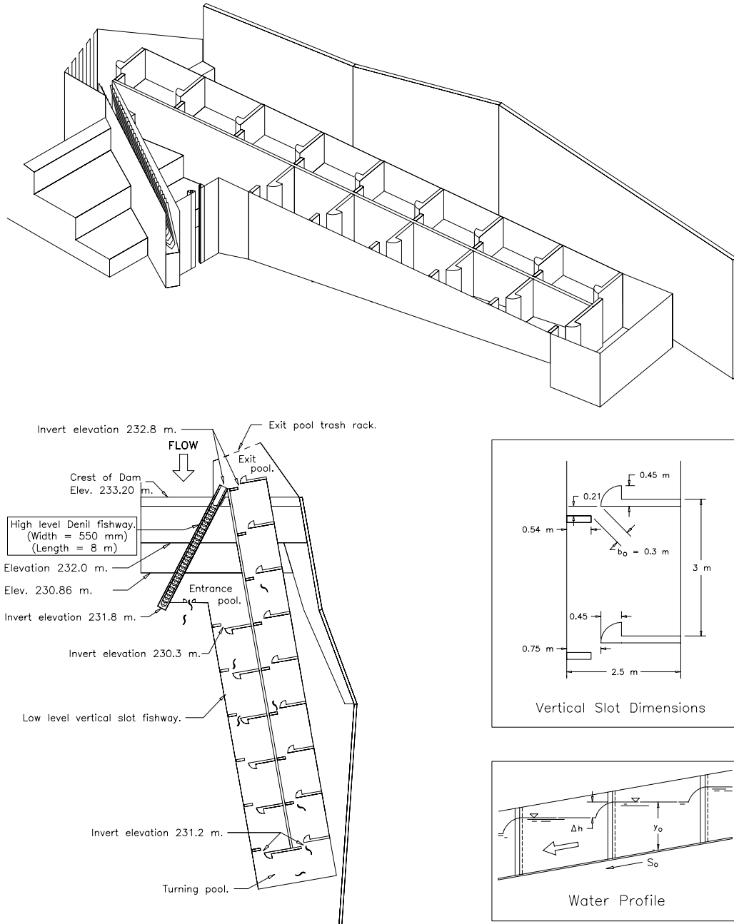
Figure 8.6. Isometric and plan view of the Hunt Dam fishways.
