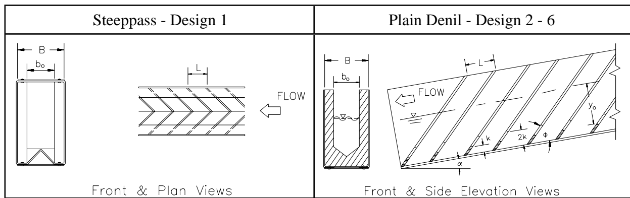
Figure 5.3 Denil fishway design layouts.
