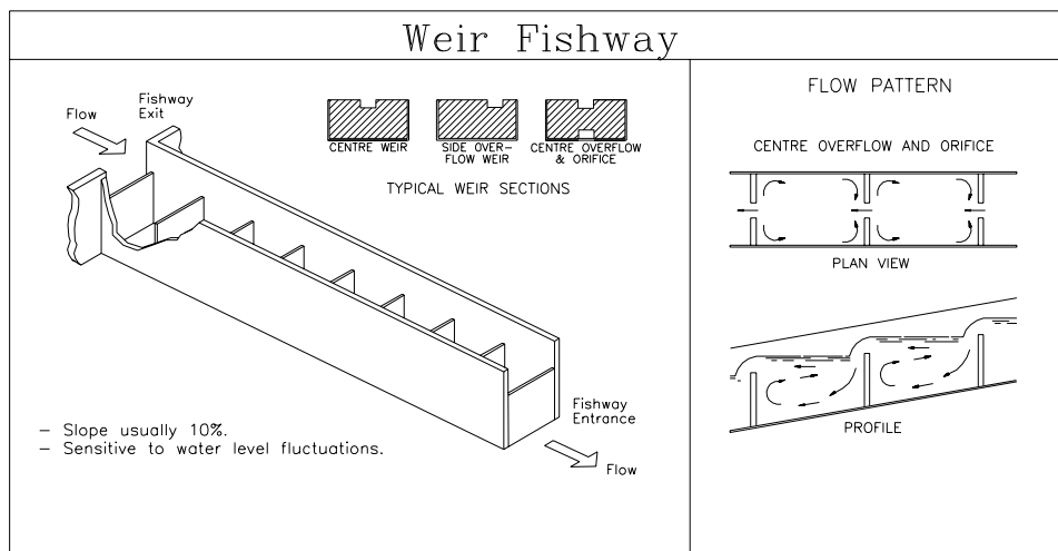
Figure 2.3 Weir Fishway
