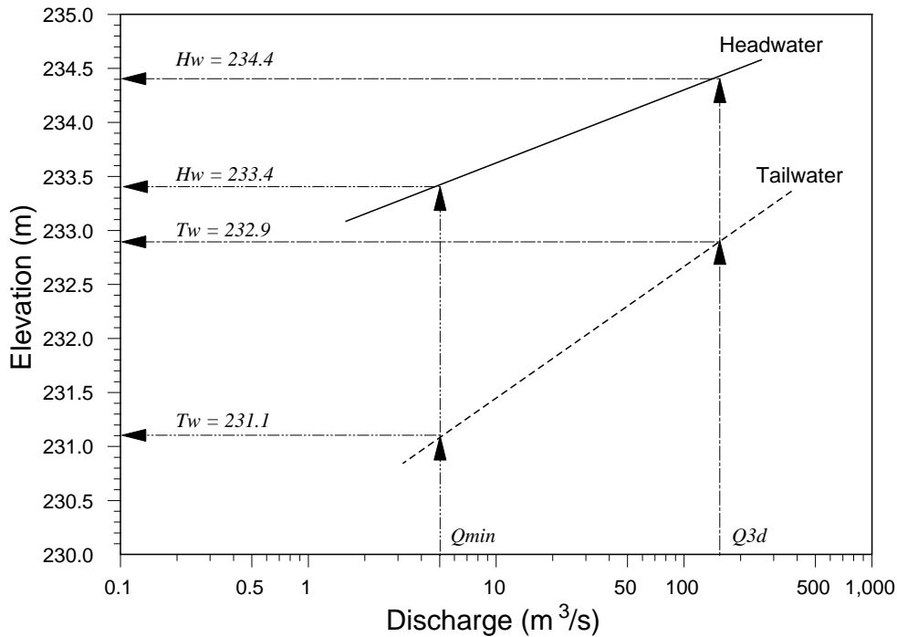
Figure 8.5 Hunt Dam discharge rating curves.
