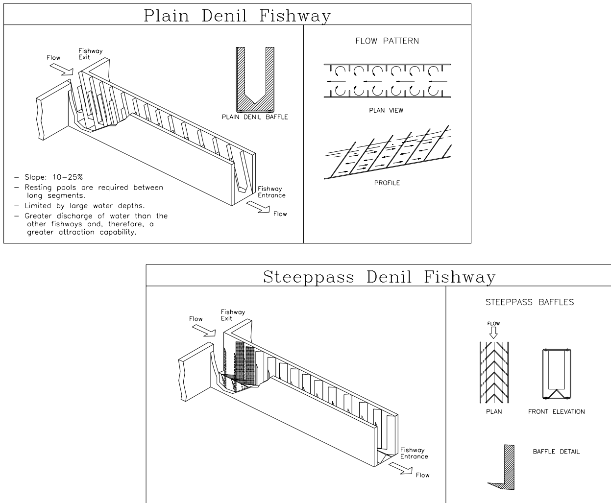
Figure 2.2 Denil Fishways
