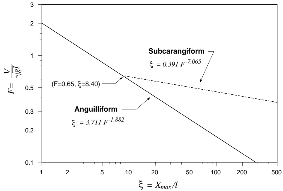
Figure 6.3 Dimensionless swimming distance curves.
