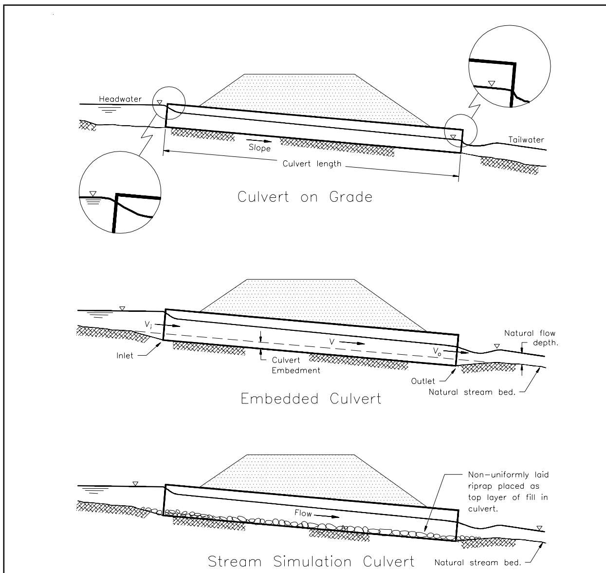
Figure 2.4a Culvert placement.
