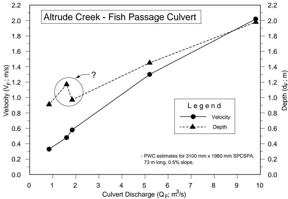
Figure 8.2 Depth and velocity vs discharge for fish passage culvert at Altrude Creek.
