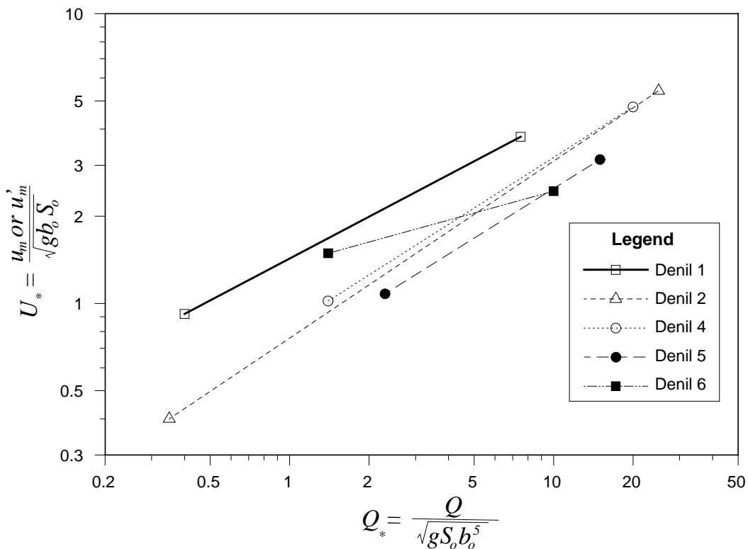
Figure 5.5 Denil fishway dimensionless velocity scales.
