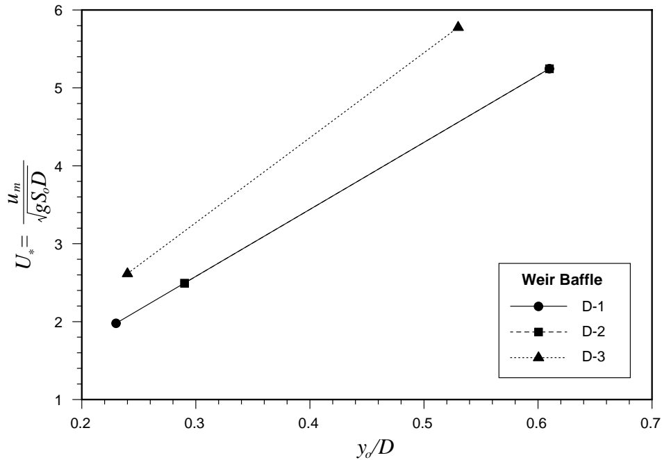
Figure 5.10 Weir baffle dimensionless velocity scales.
