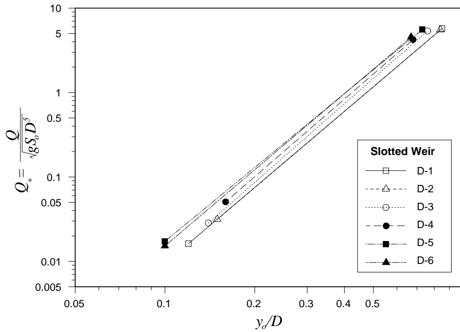
Figure 5.11 Slotted weir baffle dimensionless discharge curves.
