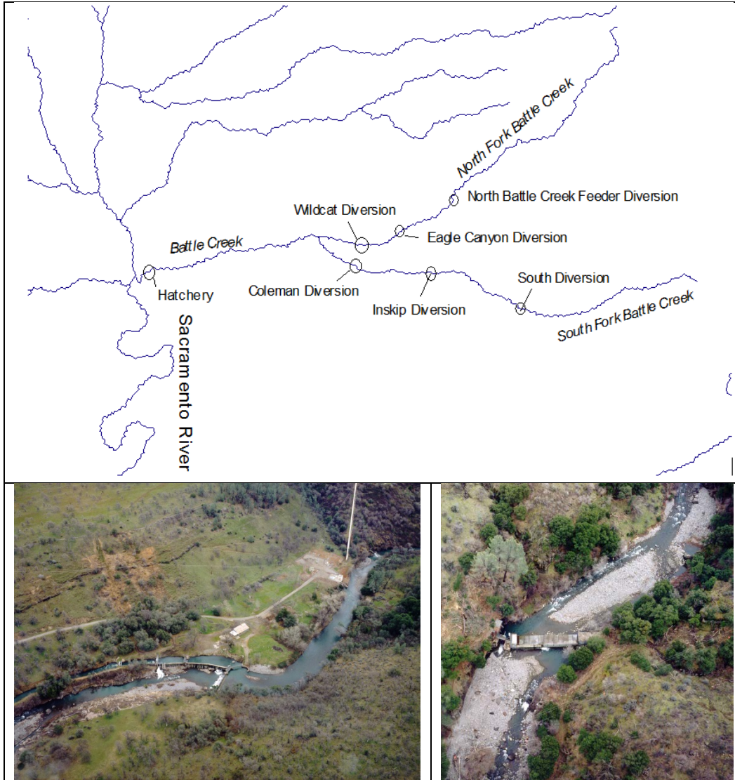
Figure 40. —Locations of dams removed within Battle Creek Salmon and Steelhead Restoration Project (upper image), view of Coleman Diversion Dam (lower left), and view of South Diversion Dam (lower right) (Jones and Stokes, 2005). Note that Inskip Diversion and the hatchery were not removed.
