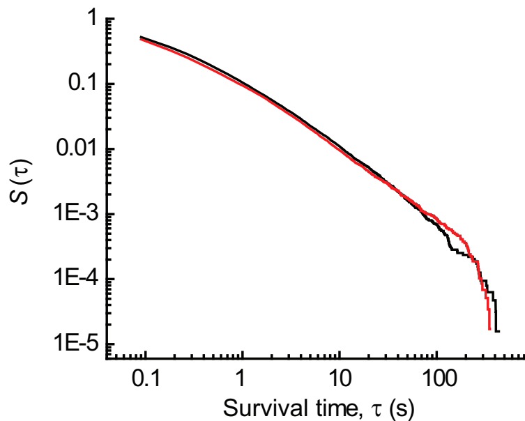
FIG. S2. The survival probability of BSA molecules on PEG surface. The data is similar to that of Fig. 1a in the main text, but the fluorophores are continually excited and the frame rate is 20 fold higher. As a consequence, the decay due to photobleaching takes place in a shorter timescale.
