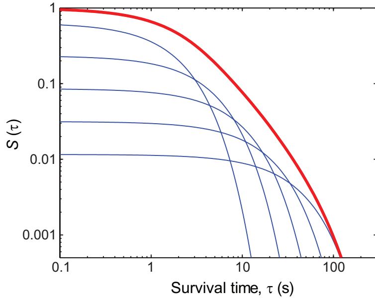
FIG. S7. Survival probability S(\tau) according to the multimer model when the approximation a/b \ll 1 does not hold. Here, a/b = 0.57 . Namely, n_0 = 1 , a = 0.57 , and b = 1 . Only the first five modes of k_n are used. The thin blue lines show the contribution of each of these modes to the survival probability: p(n) \exp(-k_n \tau) . The thick red line shows the survival probability: S(\tau) = \sum_{n=1}^5 S_n(\tau) p(n) . This survival probability also shows a power law tail.
