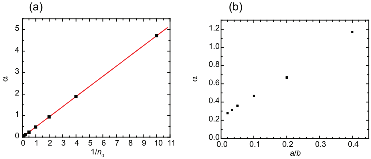
FIG. S5. Anomalous exponent \alpha in the multimer model, where S(\tau) = \sum_{n=1}^{\infty} S_n(\tau)p(n) and S(\tau) \sim \tau^{-\alpha} . The exponent \alpha is shown for different choices of parameters n_0 (characteristic number of monomers in adsorbed particle) and a and b (dissociation and association coefficients, respectively). (a) \alpha is shown as a function of 1/n_0 to highlight the behavior S \sim 1/n_0 . (b) \alpha is shown as a function of a/b . Different sets of a and b values are used but they all fall within a master curve that only depends on a and b via their ratio a/b .
