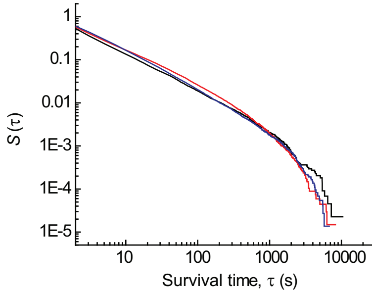
FIG. S6. Survival probability S(\tau) for the surface dwell times of BSA molecules on high density PEG surface.
