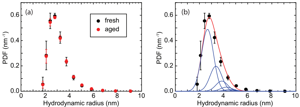
FIG. S3. Measurements of the distribution of Stokes hydrodynamic radii using dynamic light scattering (DLS). (a) Distributions of radii in a freshly prepared BSA solution and in a solution that was allowed to settle for a period of 90 minutes. The two distributions do not appear to be significantly different. (b) The distribution of radii is fit to a model where molecules are allowed to become multimers and they are in equilibrium, so that the multimer size follows a Boltzmann distribution. A least square fit to Eq. 12 in the main text (shown as a red line) yields A_1 = 0.49 , s = 0.4 , and w = 0.49 nm. The first six Gaussian terms of the sum in Eq. 12 are shown as blue lines.
