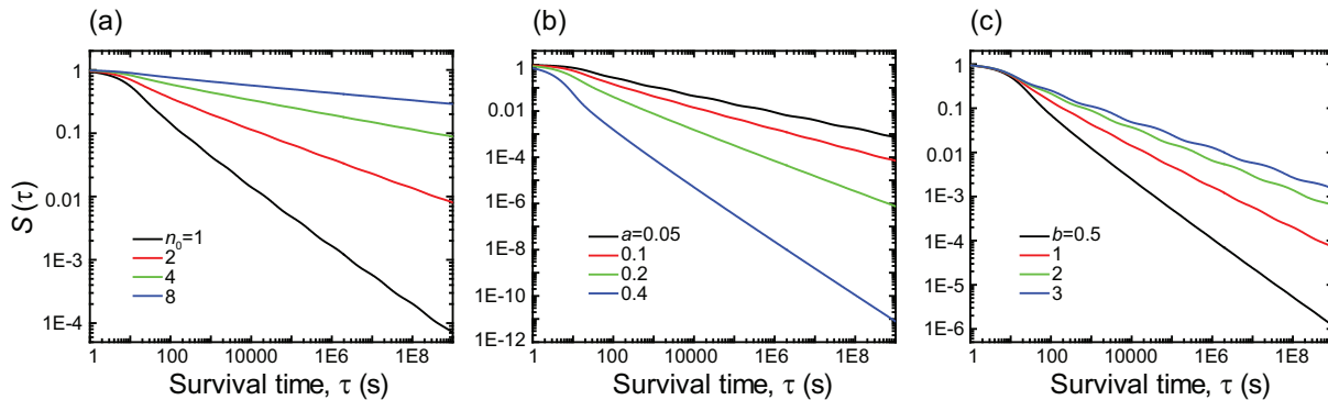
FIG. S4. Survival probability S(\tau) according to the multimer model presented in the main text exhibits a power law tail. The dwell time of particles on the surface obeys an exponential distribution, S_n(\tau) = \exp(-k_n\tau) , with mean time, 1/k_n that depends on the number of monomers within the adsorbed particle. The a priori probability is given by S(\tau) = \sum_{n=1}^{\infty} S_n(\tau)p(n) where p(n) is the probability of the particle having n monomers and it obeys a Boltzmann distribution with characteristic number of monomers n_0 . (a) Survival probability for different n_0 values. Note that larger n_0 means higher probability of the proteins to self-associate. Binding coefficient is b = 1 and unbinding rate is a = 0.1 . (b) Survival probability for different surface dissociation coefficients a . Binding coefficient is b = 1 and characteristic number of monomers is n_0 = 1 . (c) Survival probability for different surface binding affinities b . Dissociation coefficient is a = 0.1 and characteristic number of monomers is n_0 = 1 . Note that when the ratio a/b is very low, the survival probability also exhibits oscillations because the different modes separate in time.
