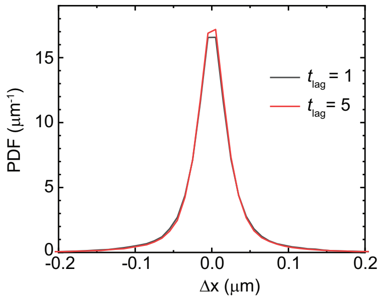
FIG. S1. Distribution of displacements along the projection on the x axis, \Delta x , for times equal to one frame (2 s) and five frames (10 s) for BSA molecules on a single PEG surface. Ignoring minor statistical errors, the two distributions are identical. The width of both distributions is dictated by the localization error of molecule detection. n = 238,415 displacements for a lag time t_{lag} = 1 frame and n = 169,642 displacements for t_{lag} = 5 frames.
