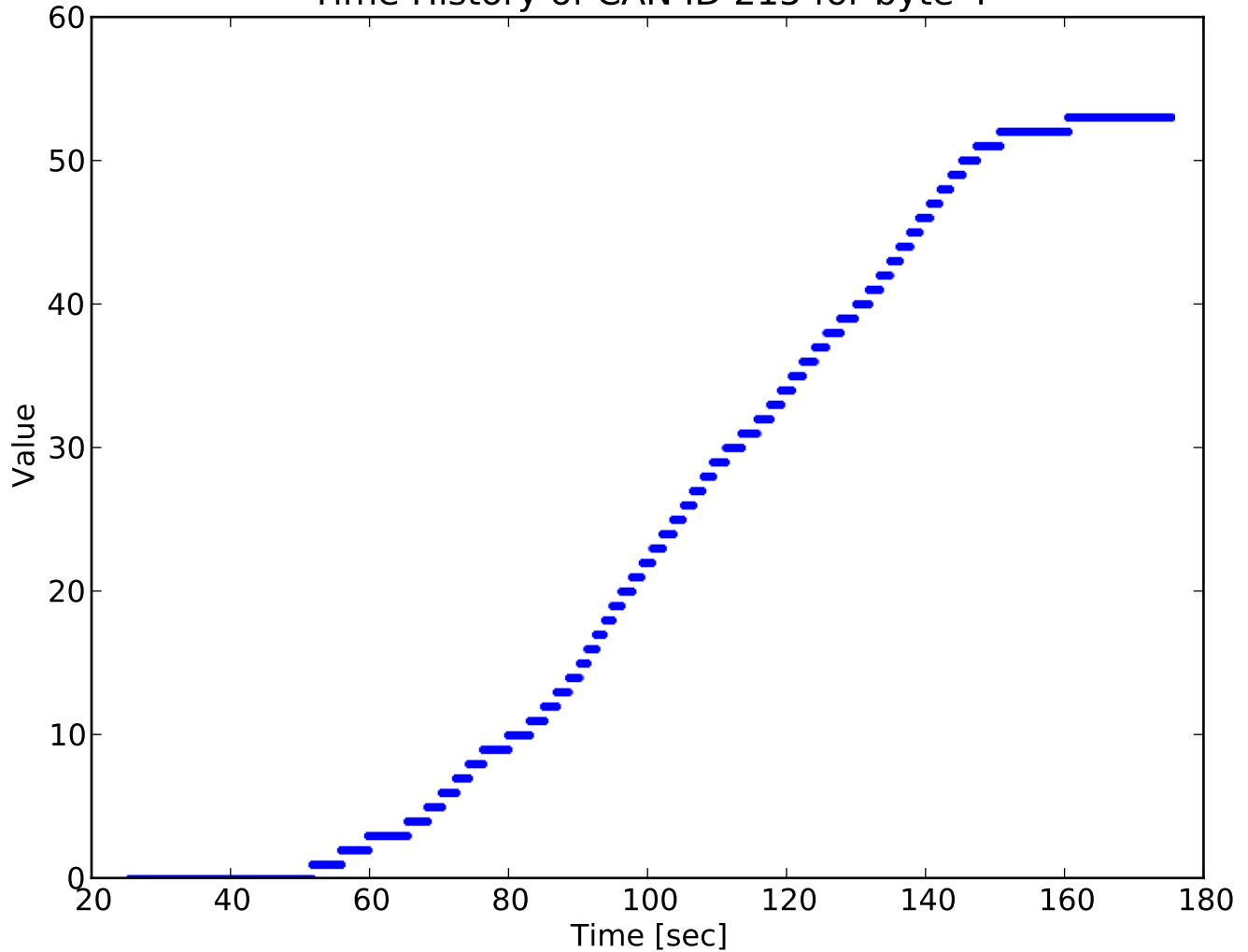
Time History of CAN ID 215 for byte 4
