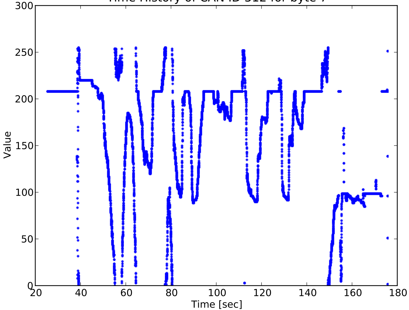
Time History of CAN ID 312 for byte 7
