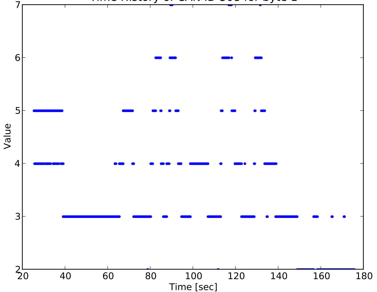
Time History of CAN ID 308 for byte 1
