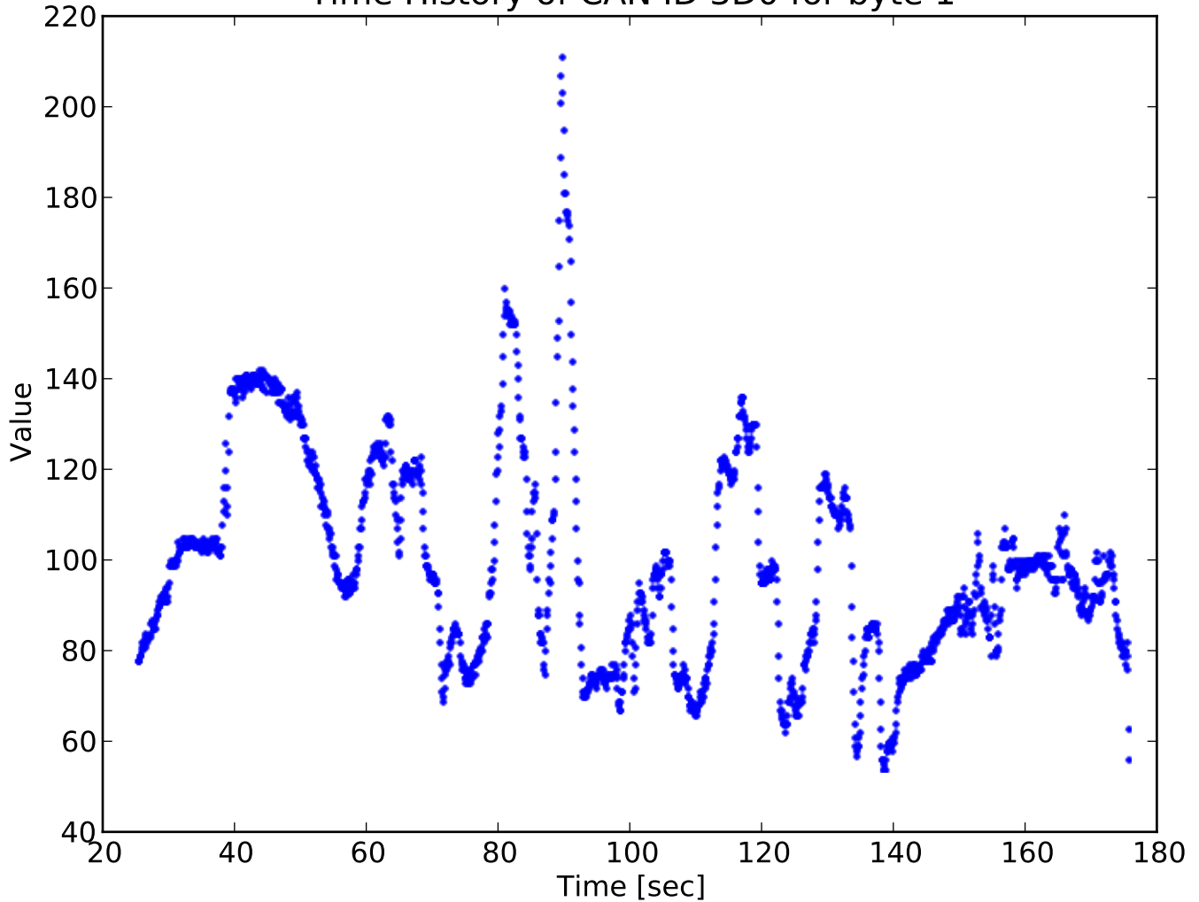
Time History of CAN ID 3D0 for byte 1
