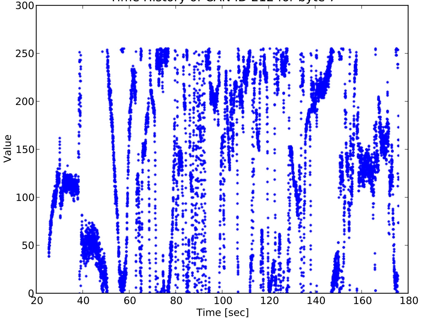
Time History of CAN ID 212 for byte 7
