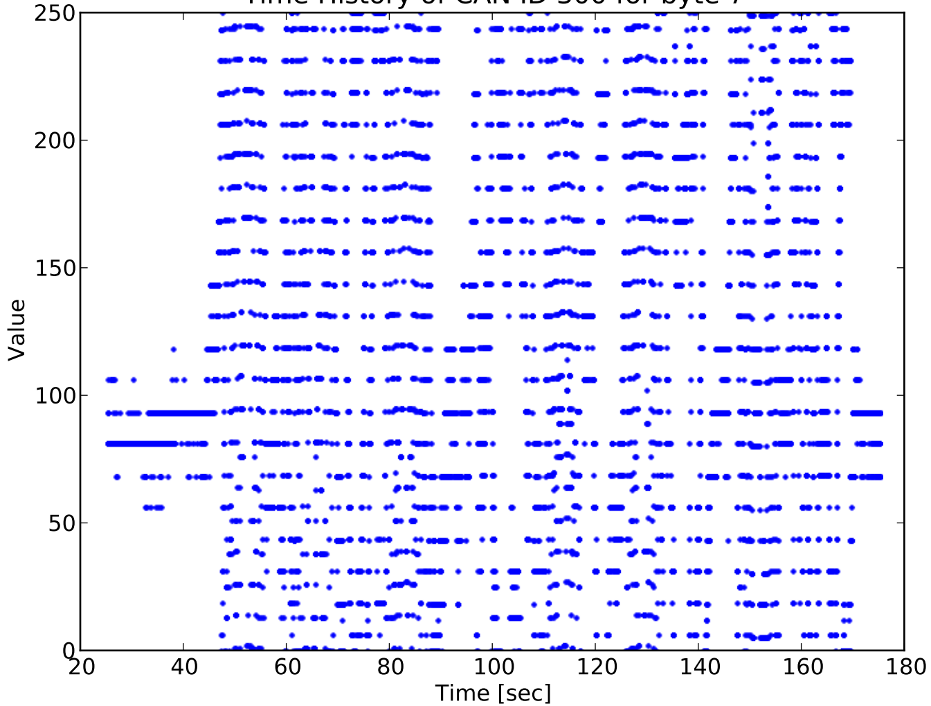
Time History of CAN ID 300 for byte 7
