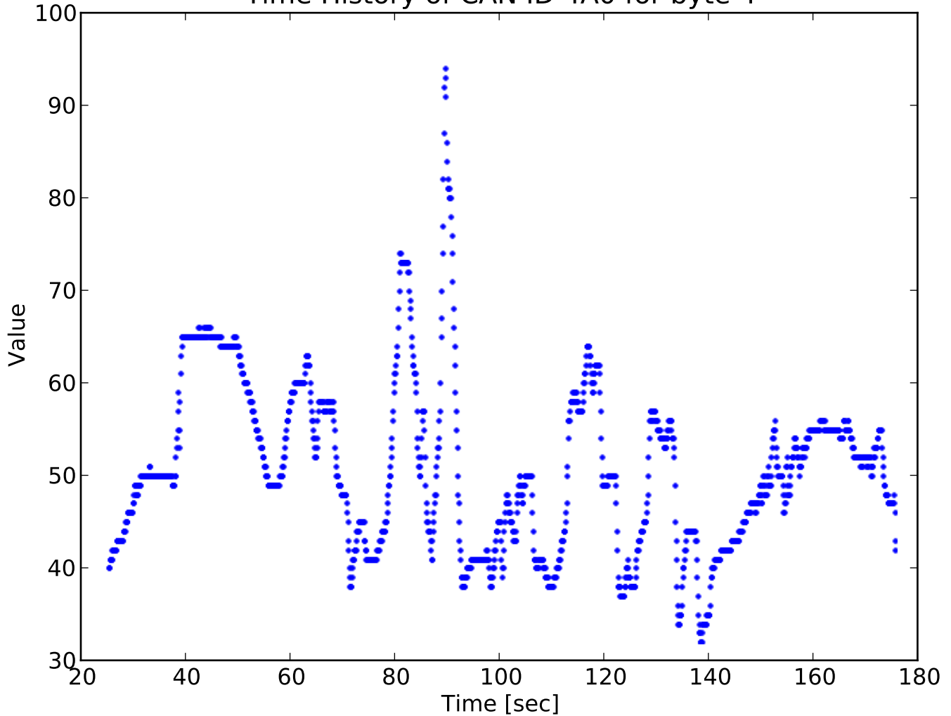
Time History of CAN ID 4A0 for byte 4
