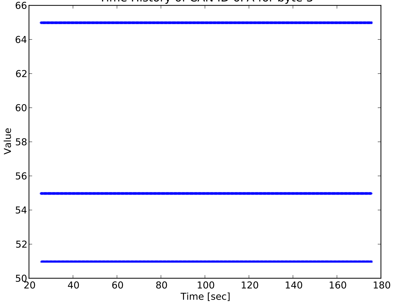
Time History of CAN ID 6FA for byte 3
