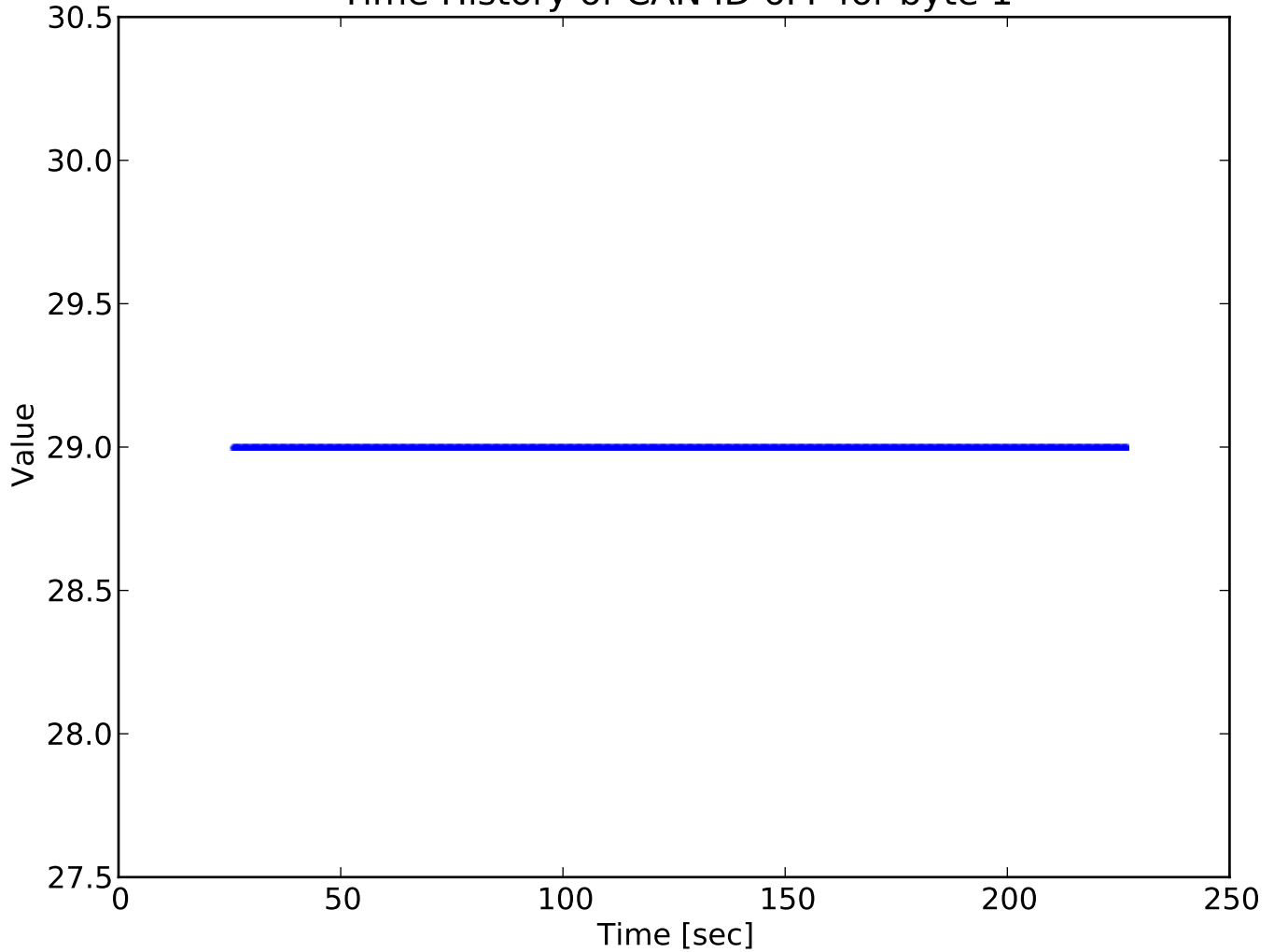
Time History of CAN ID 6FF for byte 1
