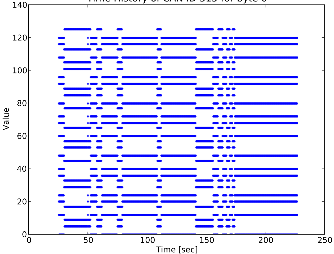
Time History of CAN ID 315 for byte 0
