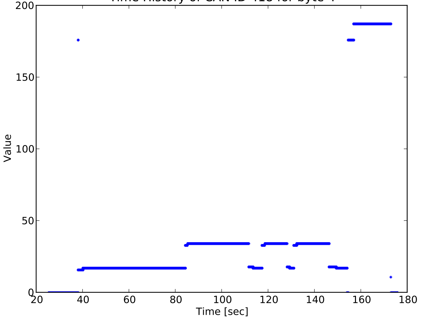
Time History of CAN ID 418 for byte 4
