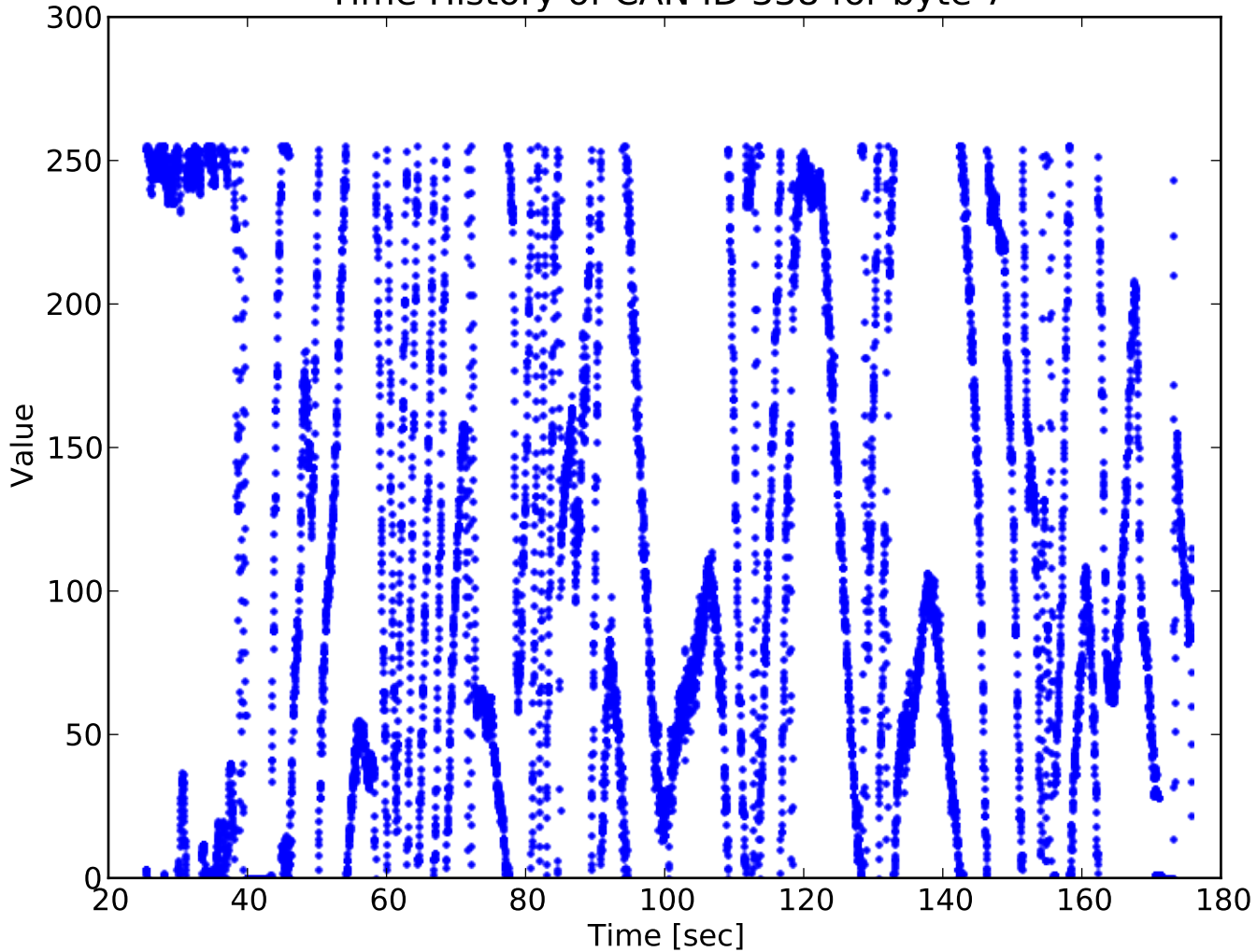
Time History of CAN ID 338 for byte 7
