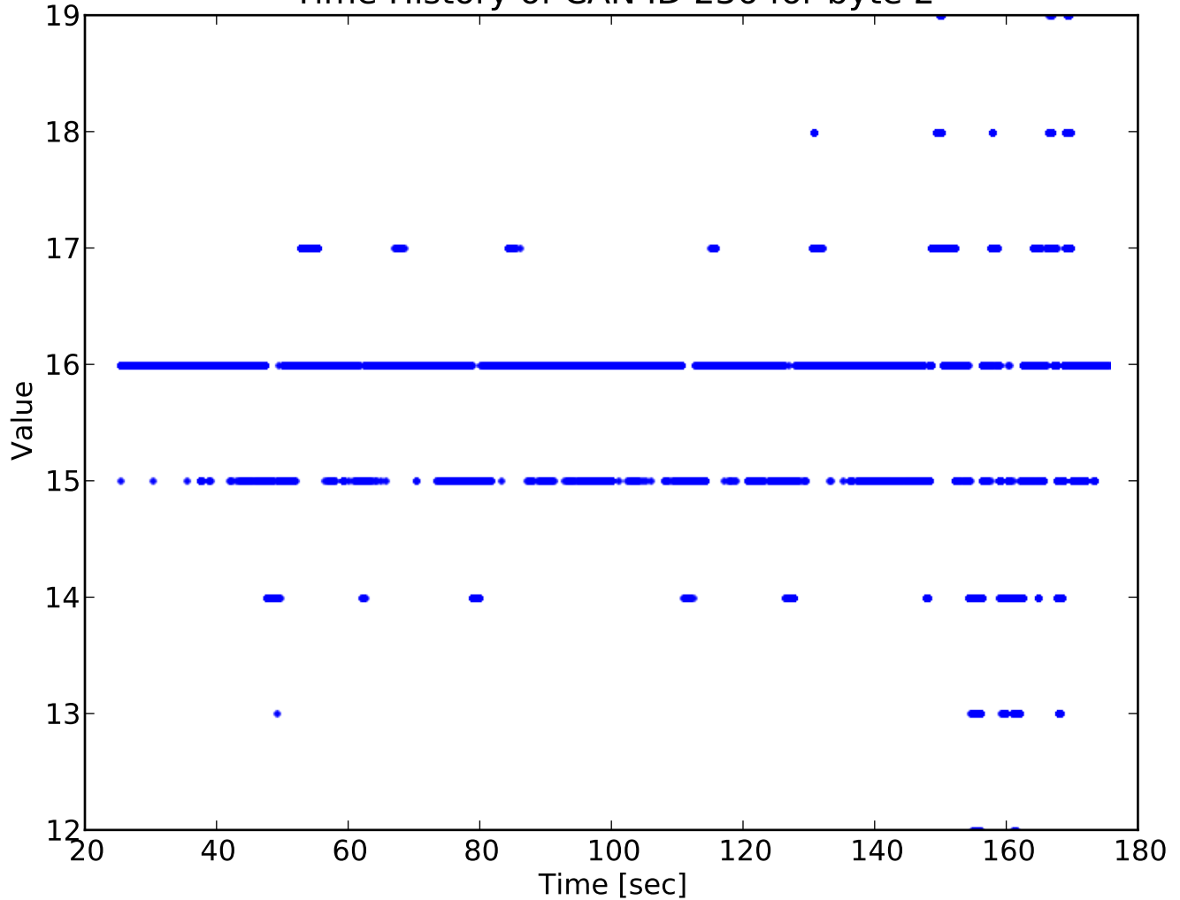
Time History of CAN ID 236 for byte 2
