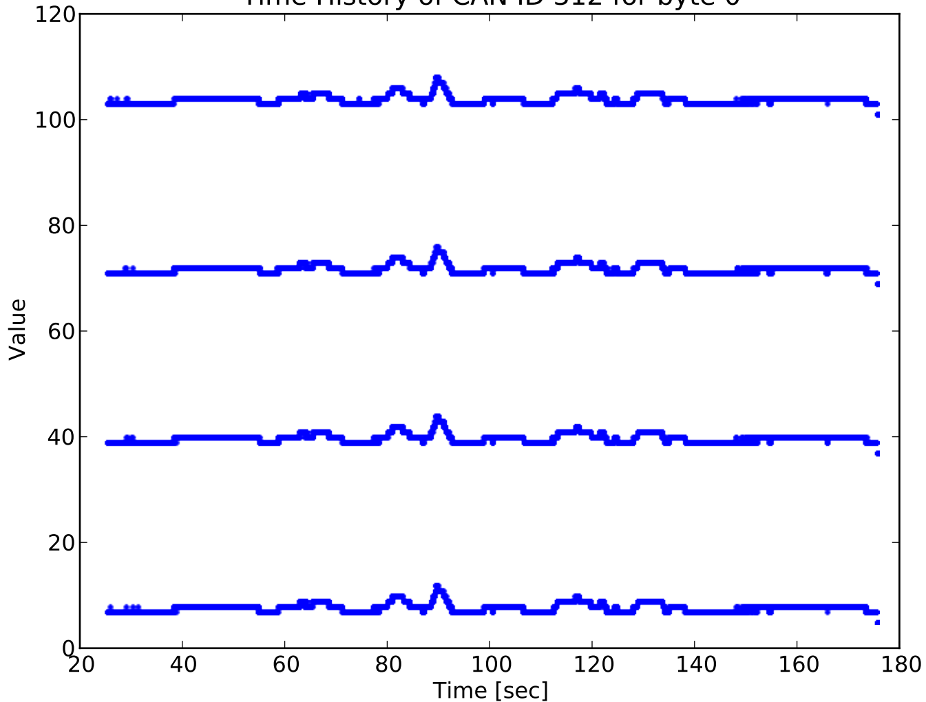
Time History of CAN ID 312 for byte 0
