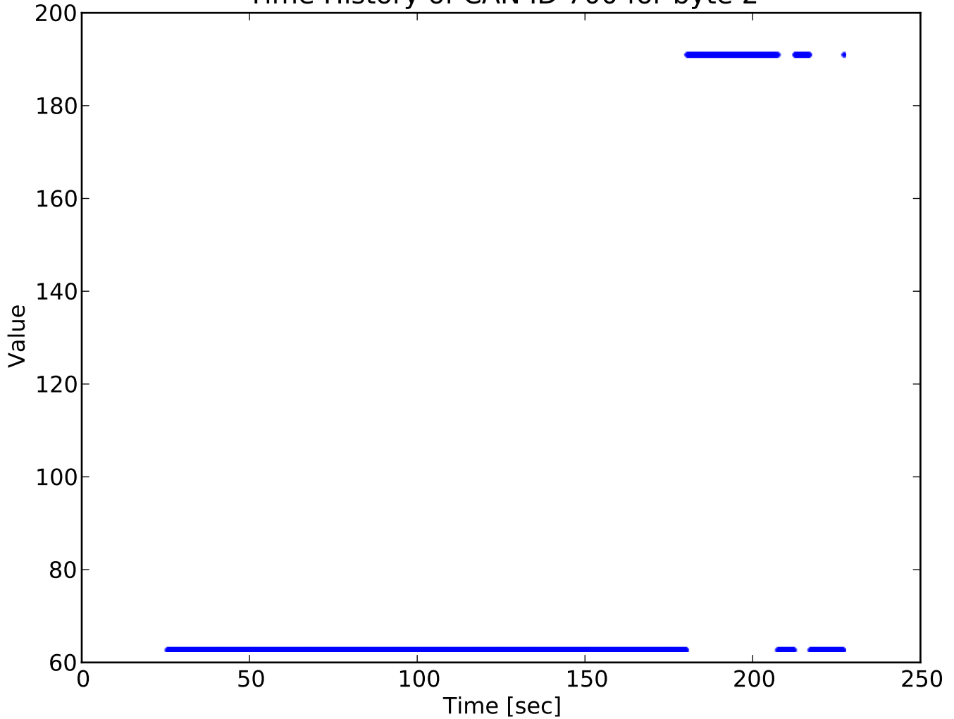
Time History of CAN ID 700 for byte 2
