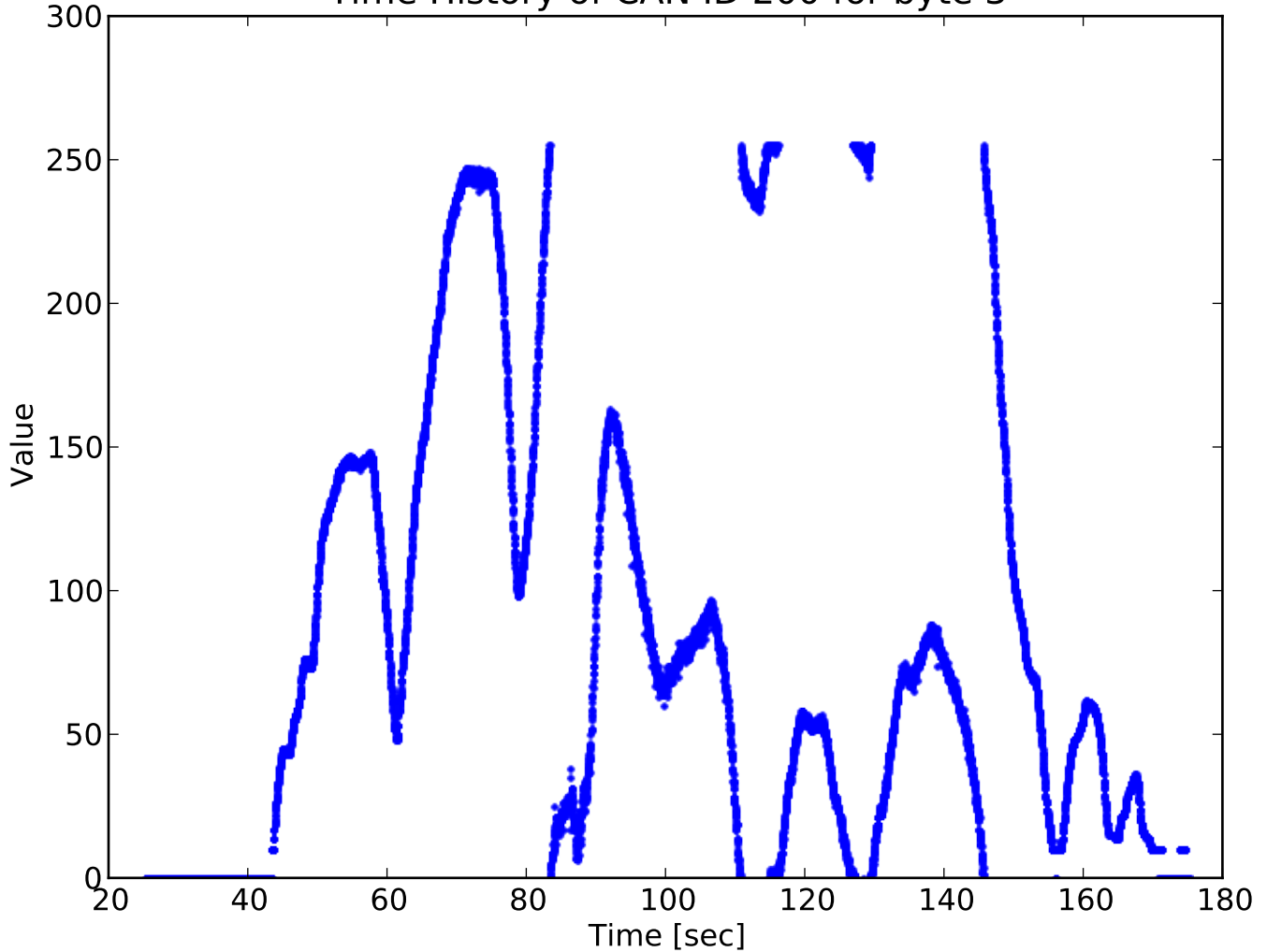
Time History of CAN ID 200 for byte 3
