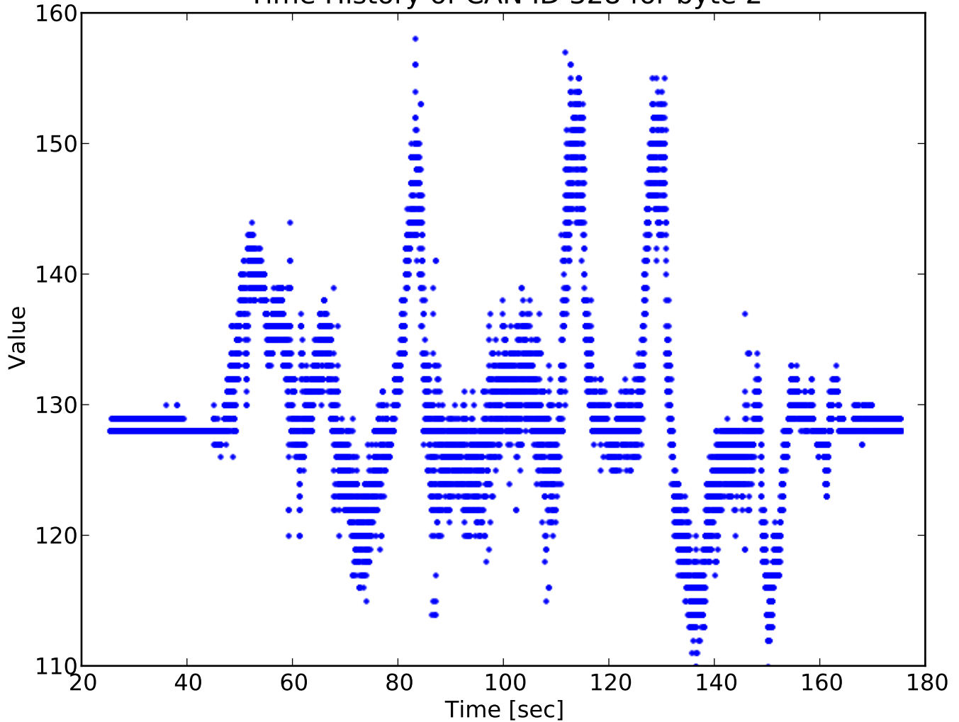
Time History of CAN ID 328 for byte 2
