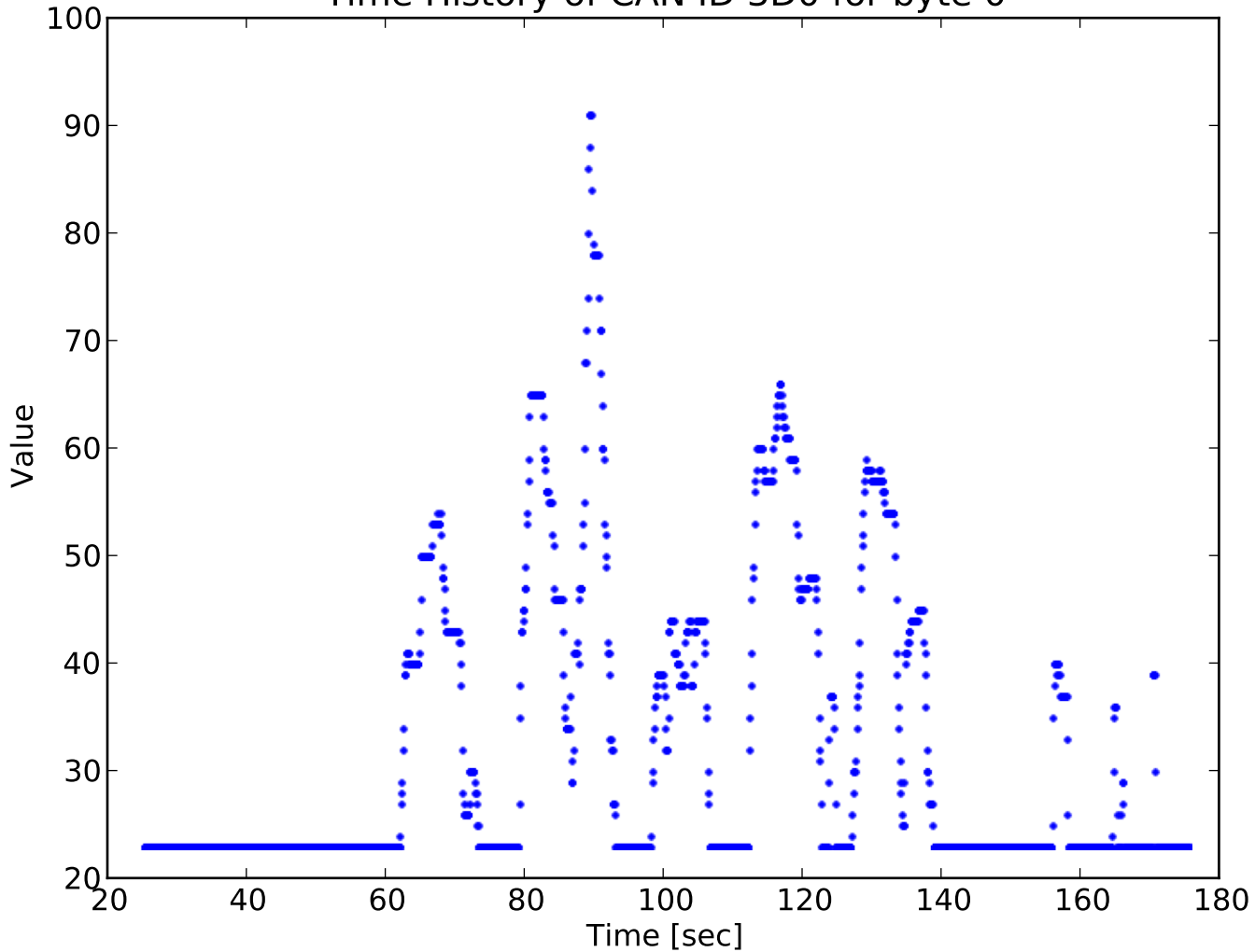
Time History of CAN ID 3D0 for byte 0
