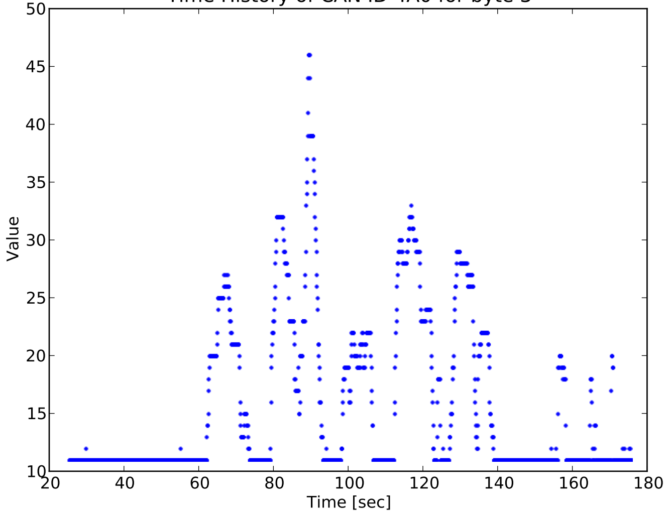
Time History of CAN ID 4A0 for byte 3
