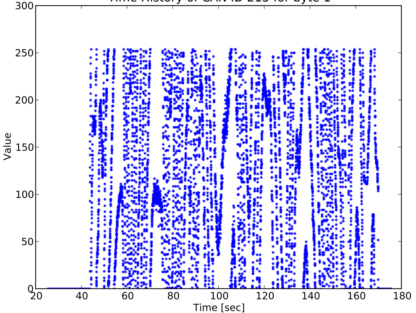
Time History of CAN ID 215 for byte 1
