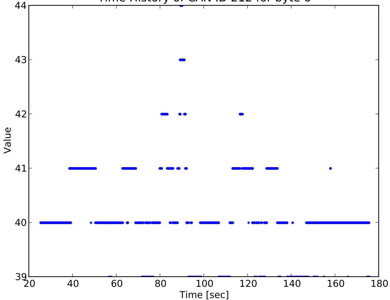
Time History of CAN ID 212 for byte 6
