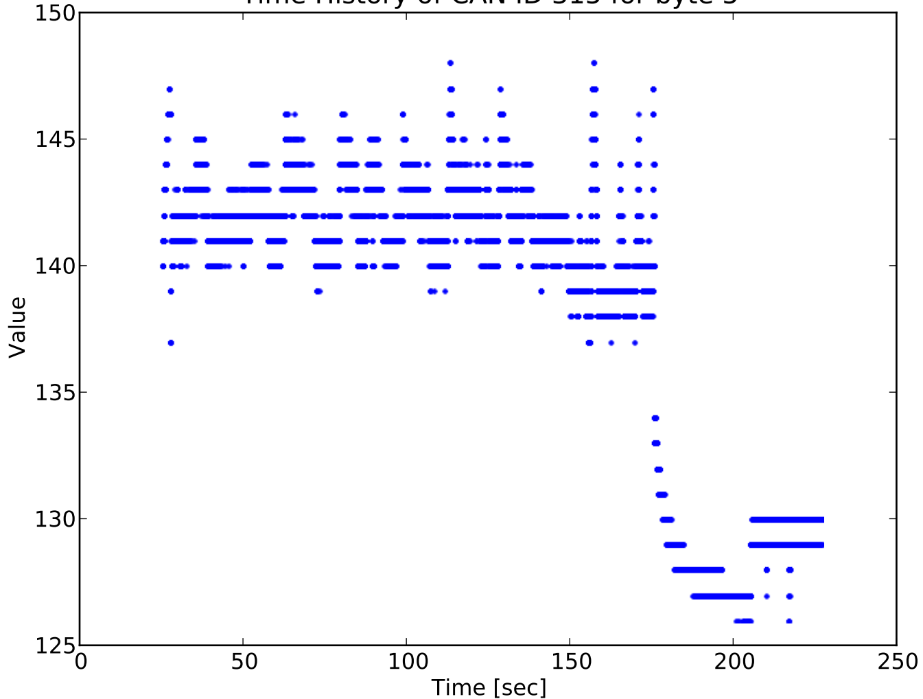
Time History of CAN ID 315 for byte 5
