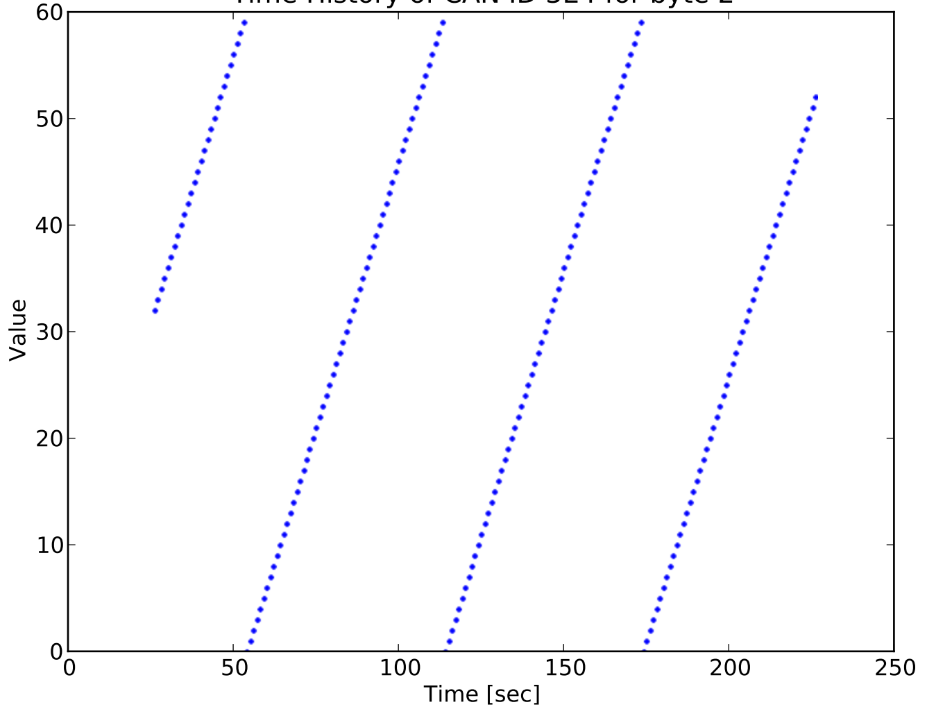
Time History of CAN ID 3E4 for byte 2
