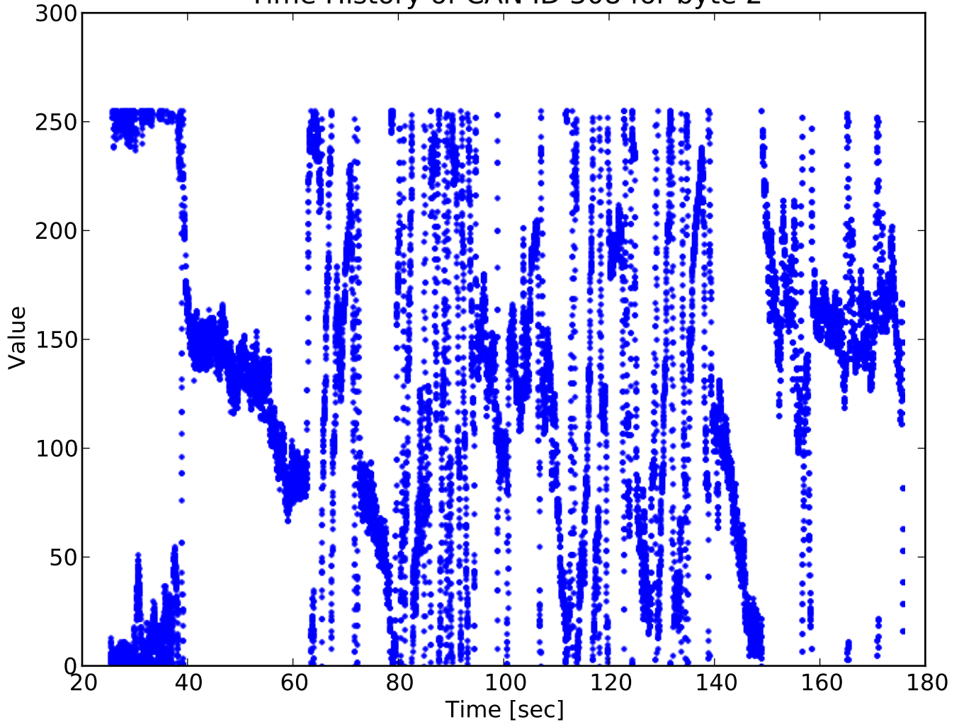
Time History of CAN ID 308 for byte 2
