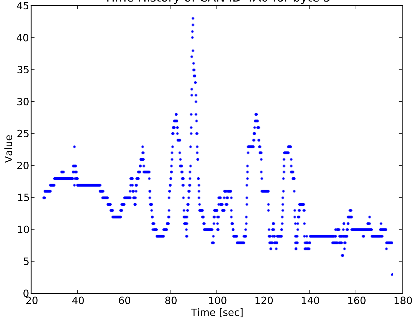
Time History of CAN ID 4A0 for byte 5
