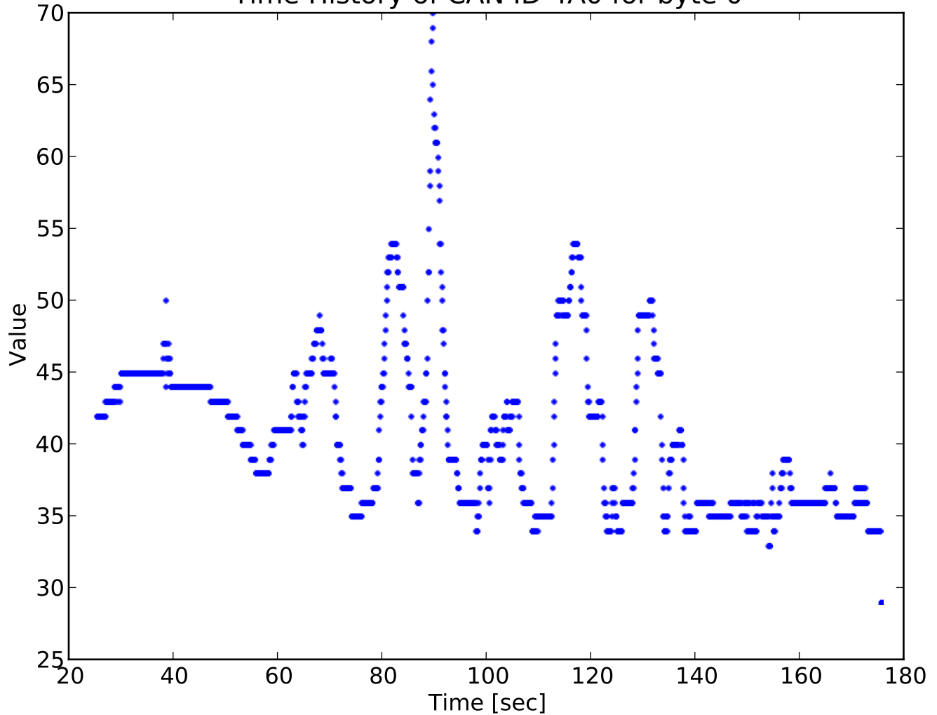
Time History of CAN ID 4A0 for byte 0
