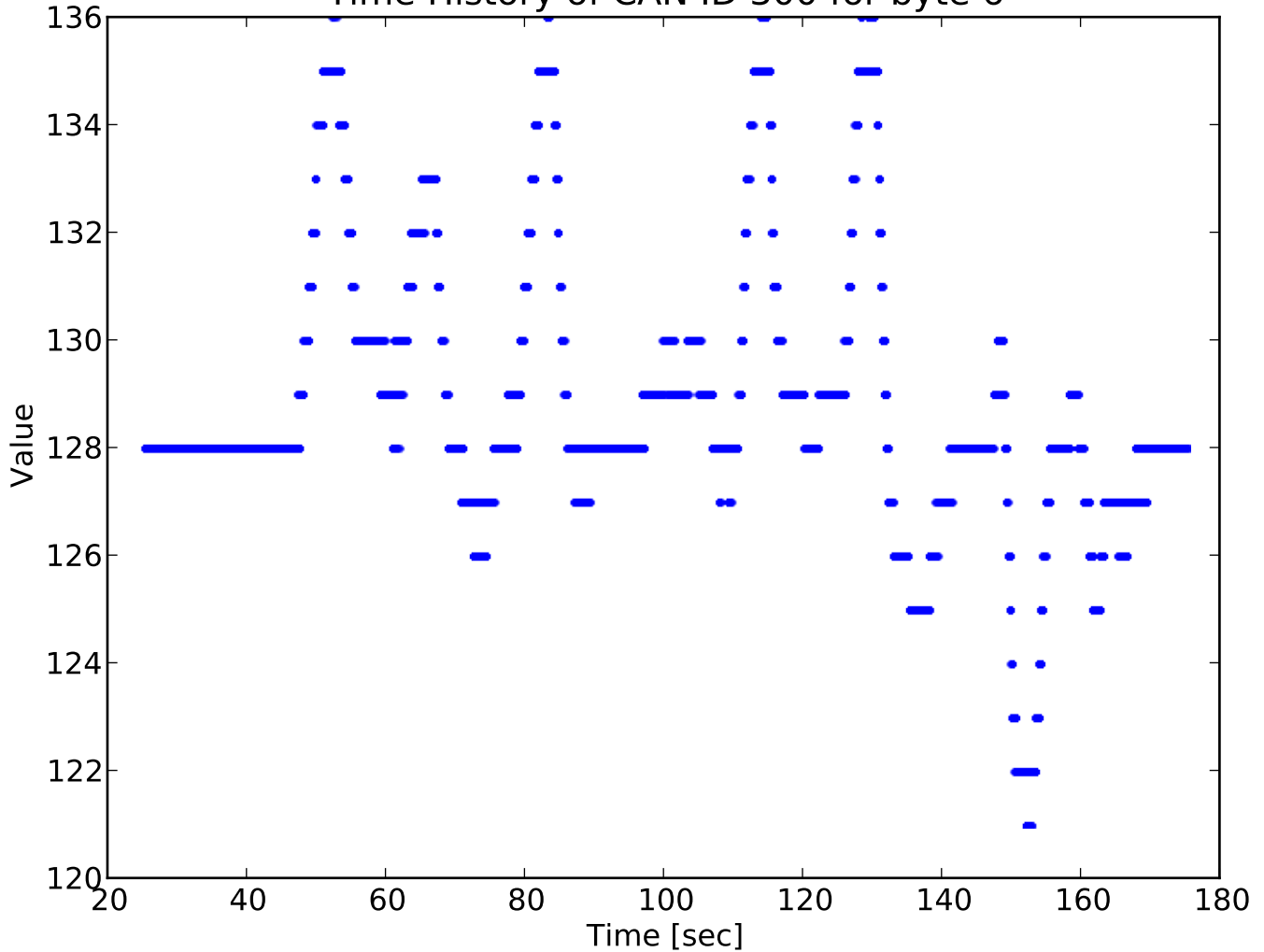
Time History of CAN ID 300 for byte 6
