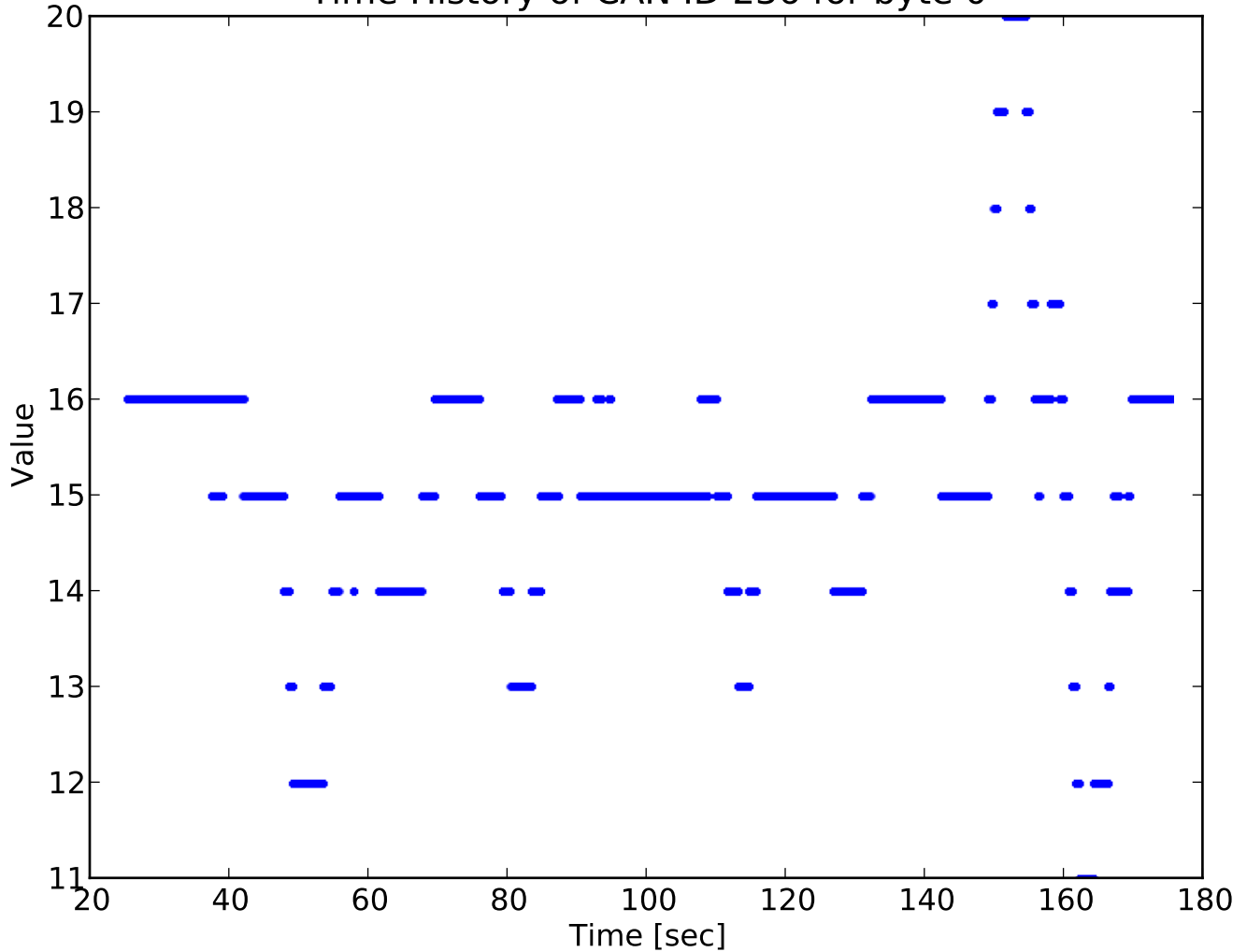
Time History of CAN ID 236 for byte 0
