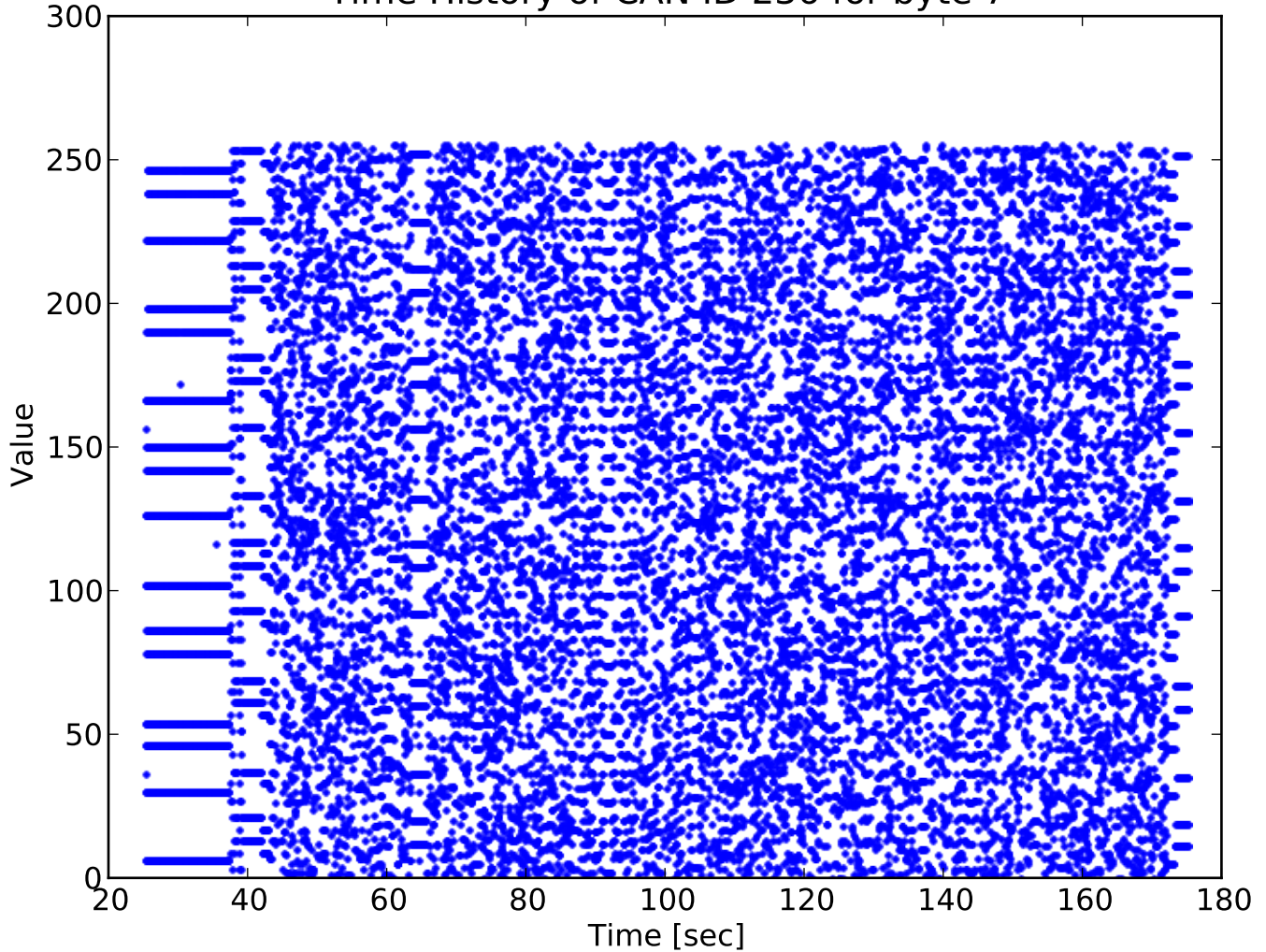
Time History of CAN ID 236 for byte 7
