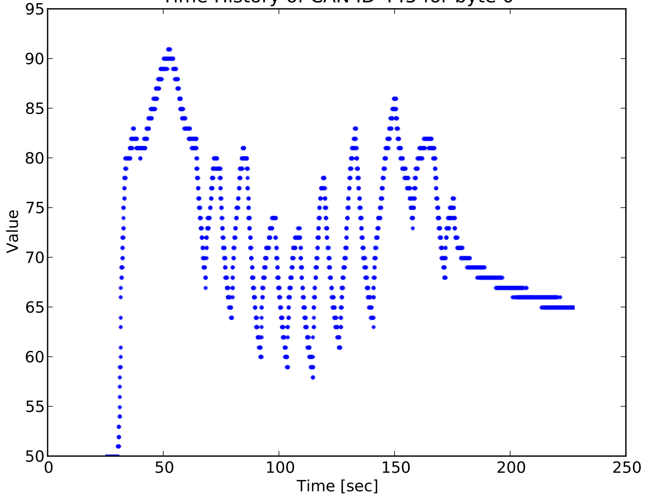
Time History of CAN ID 445 for byte 0
