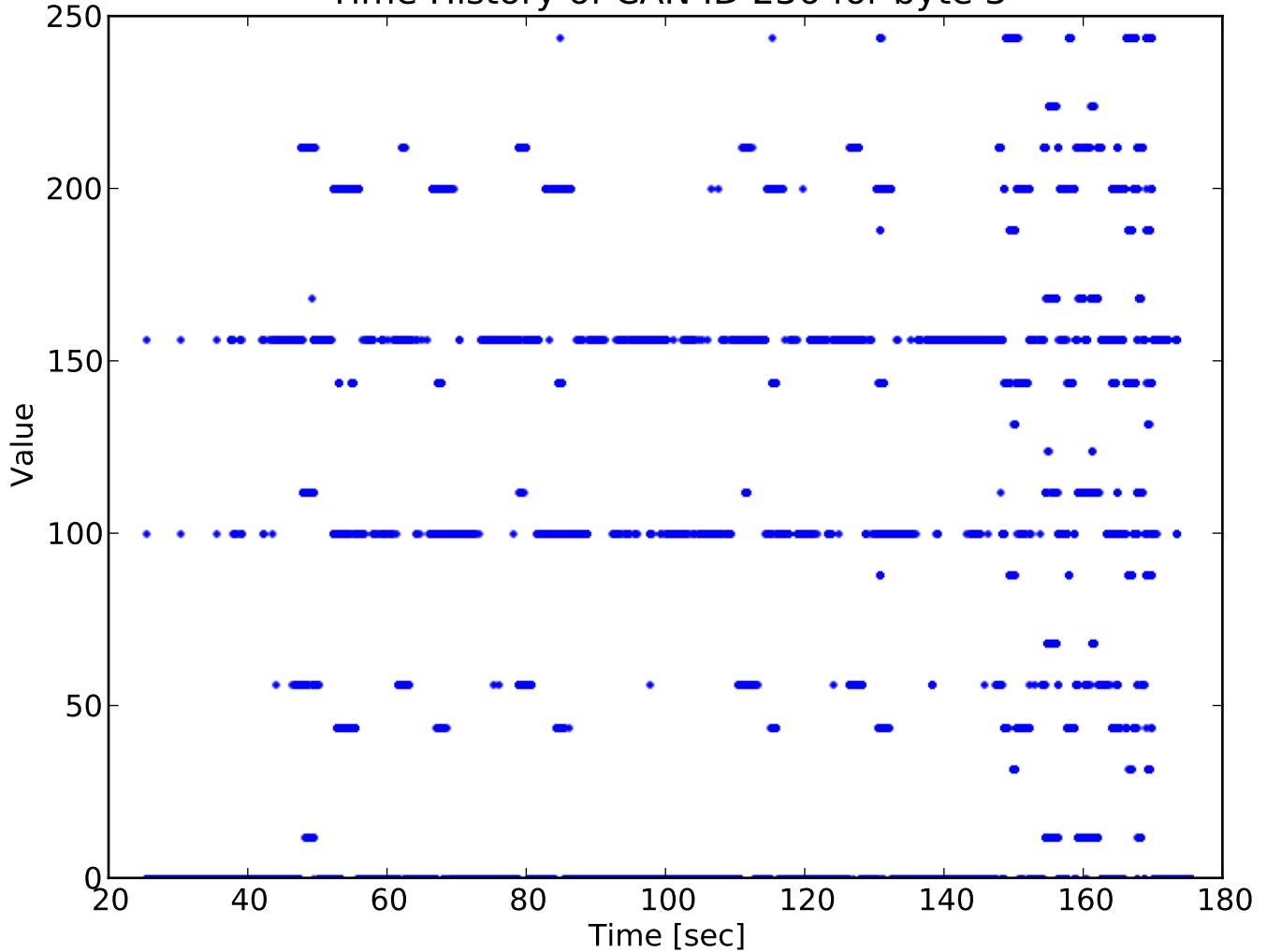
Time History of CAN ID 236 for byte 3
