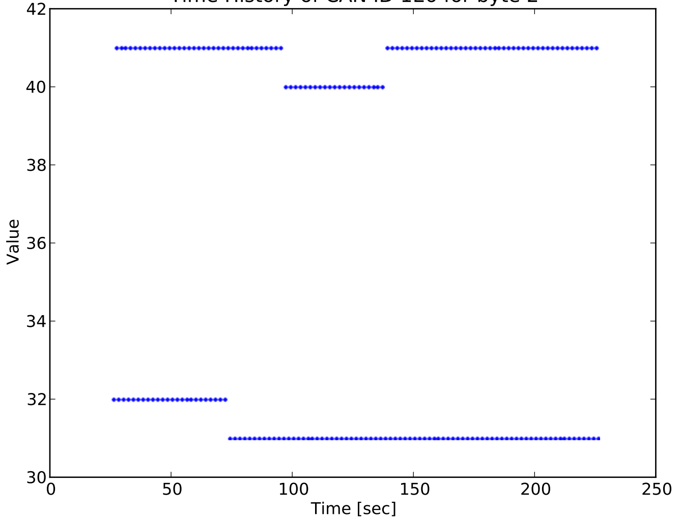
Time History of CAN ID 1E6 for byte 2
