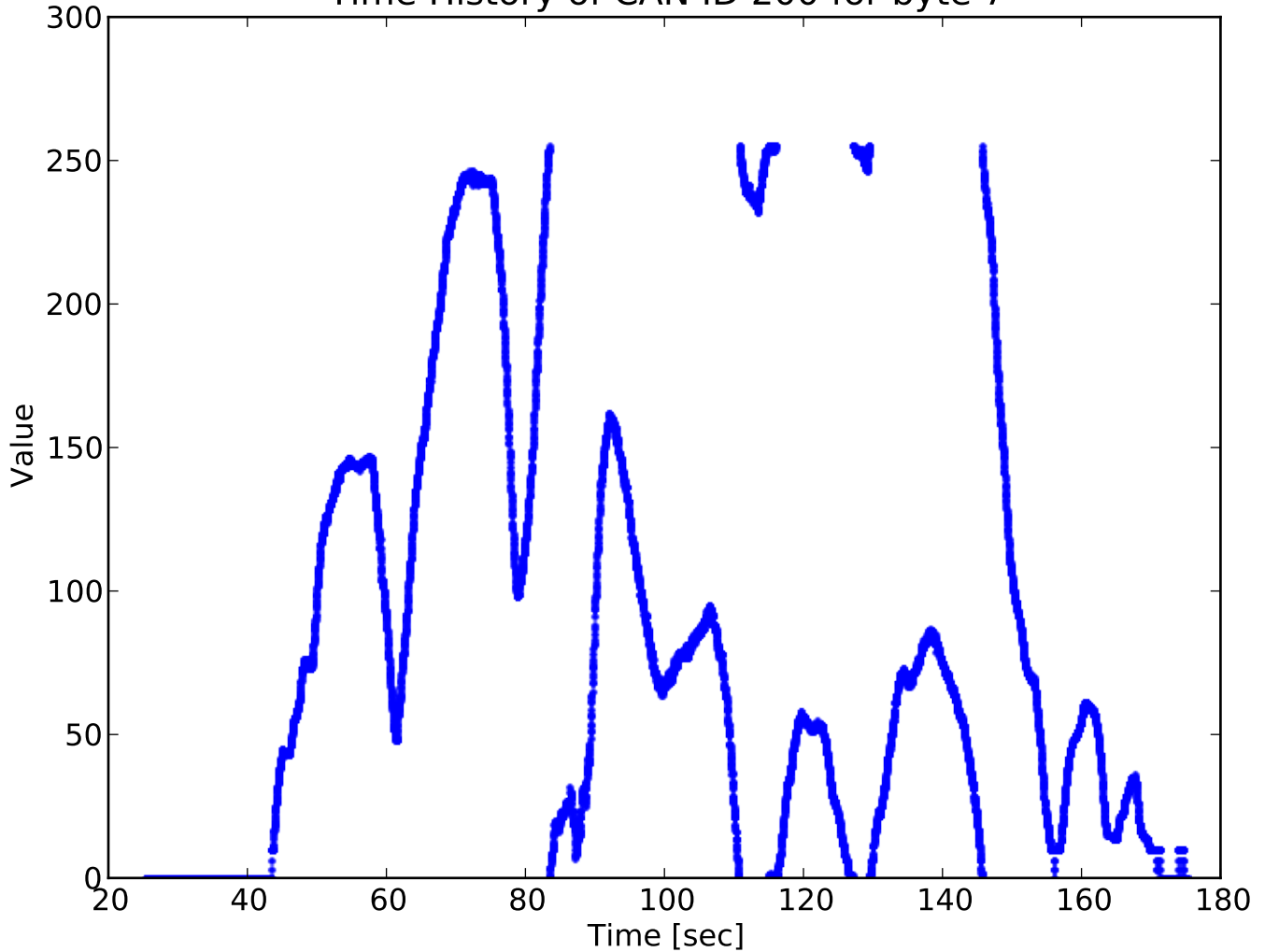
Time History of CAN ID 200 for byte 7
