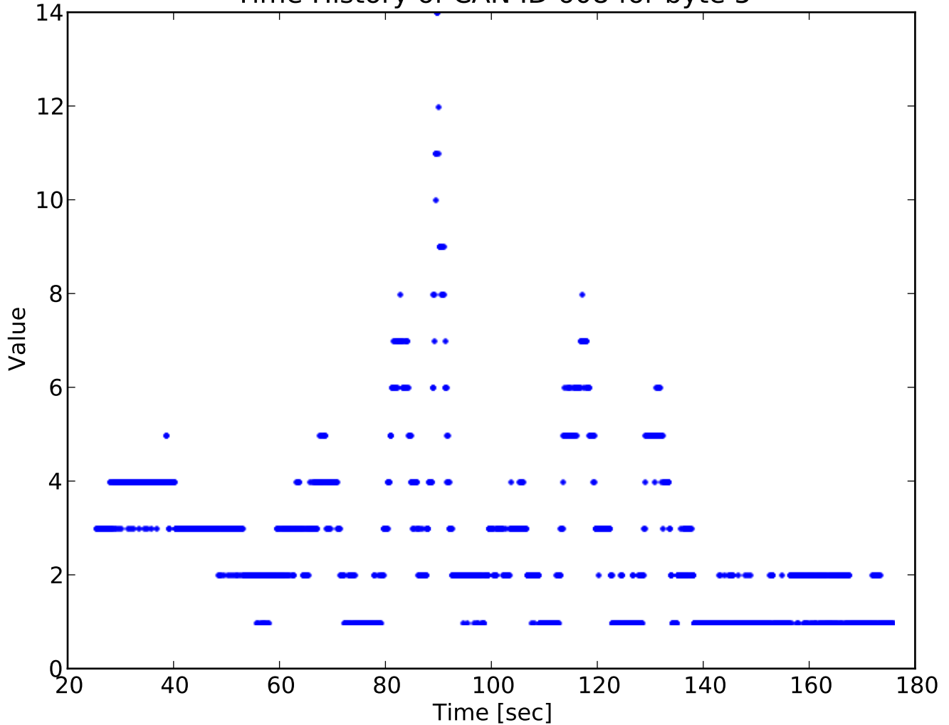
Time History of CAN ID 608 for byte 5
