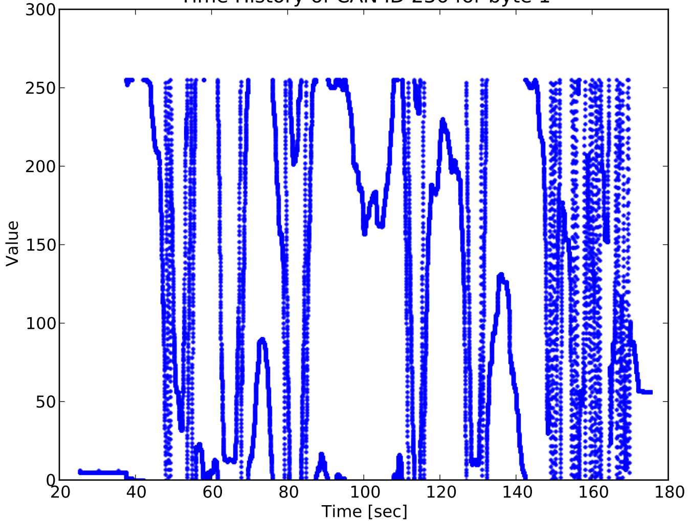
Time History of CAN ID 236 for byte 1
