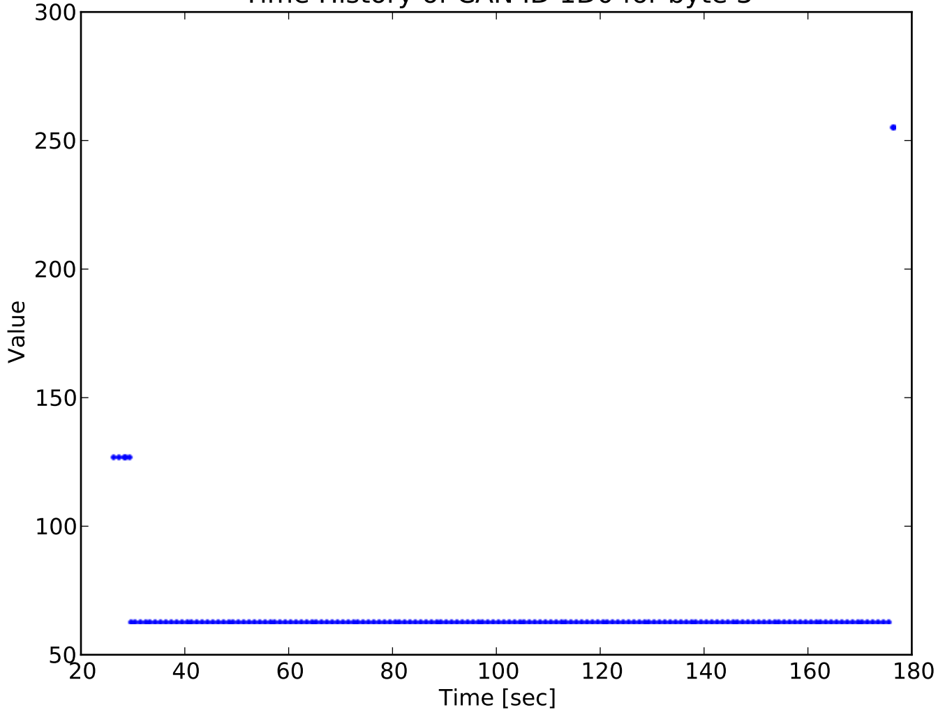
Time History of CAN ID 1D0 for byte 3
