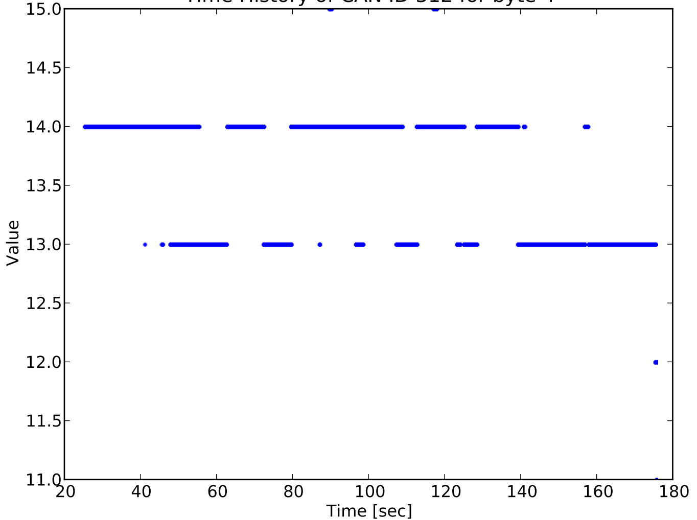
Time History of CAN ID 312 for byte 4
