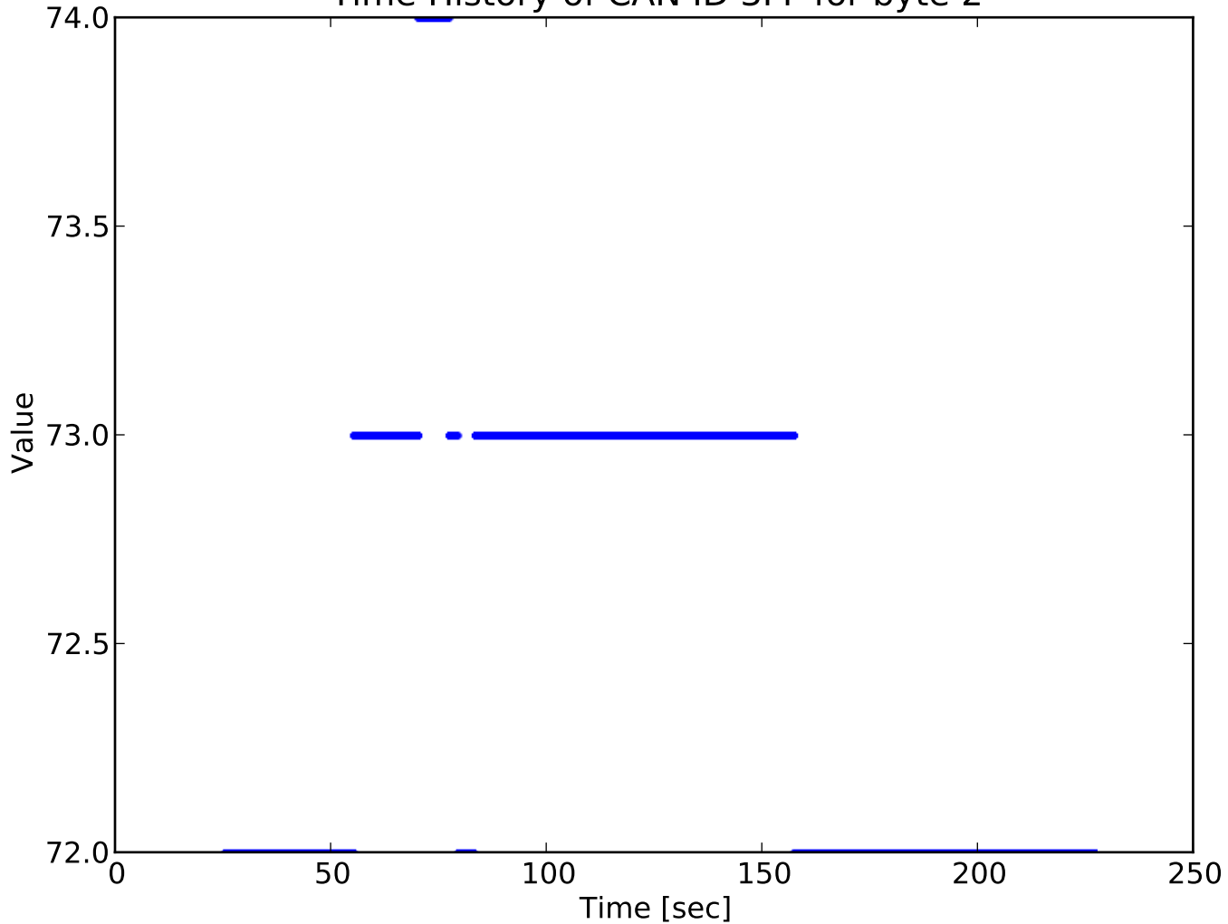
Time History of CAN ID 3FF for byte 2
