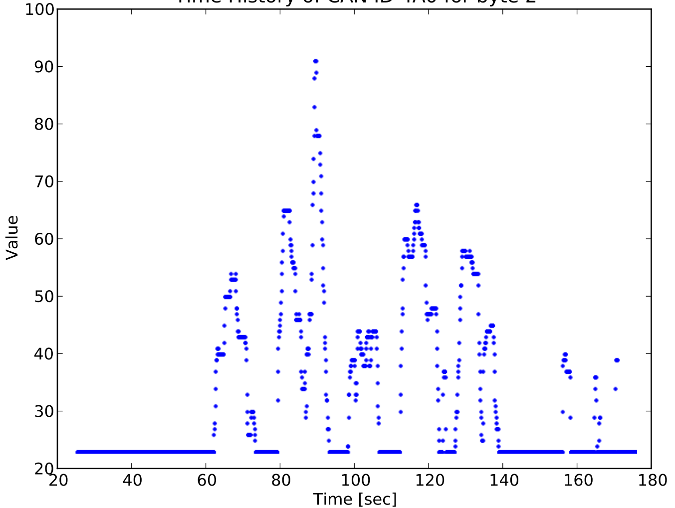
Time History of CAN ID 4A0 for byte 2
