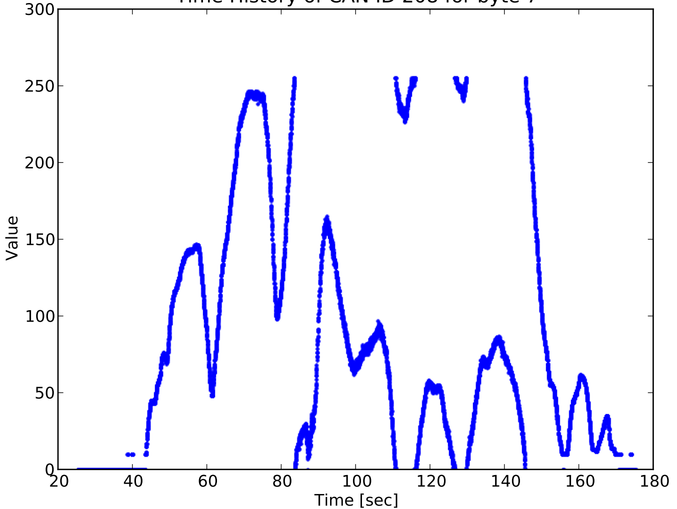
Time History of CAN ID 208 for byte 7
