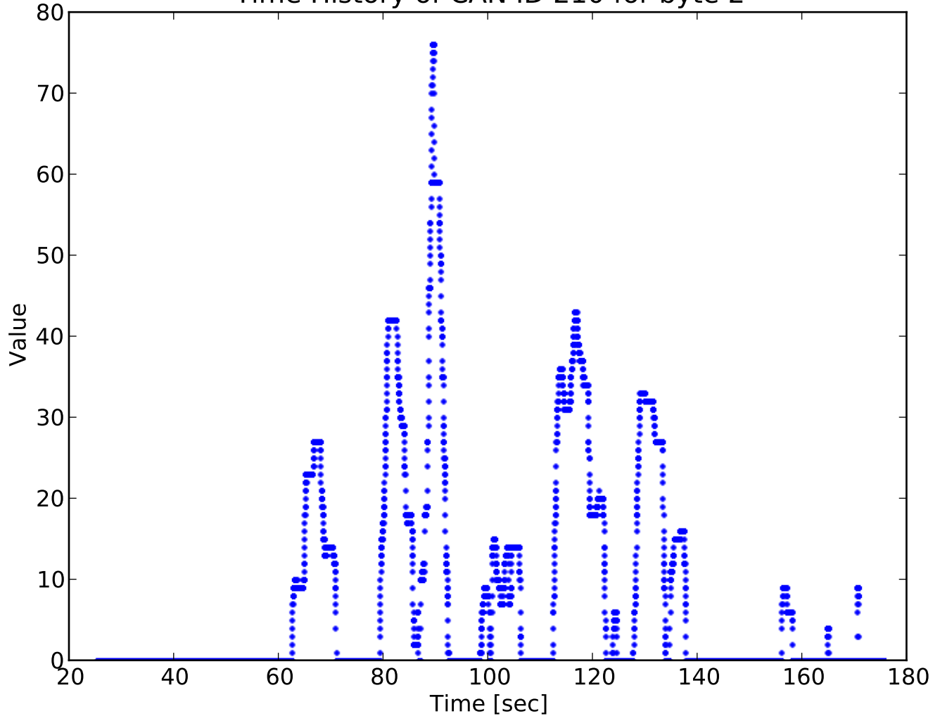
Time History of CAN ID 210 for byte 2
