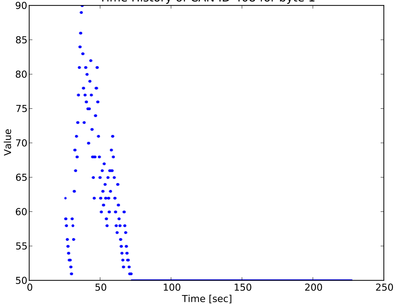
Time History of CAN ID 408 for byte 1
