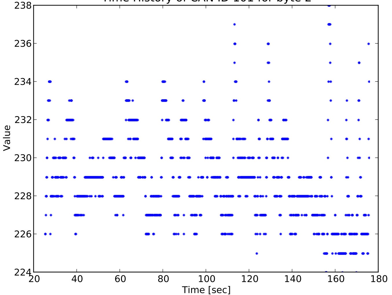
Time History of CAN ID 101 for byte 2
