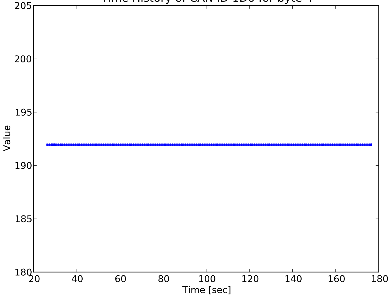
Time History of CAN ID 1D0 for byte 4
