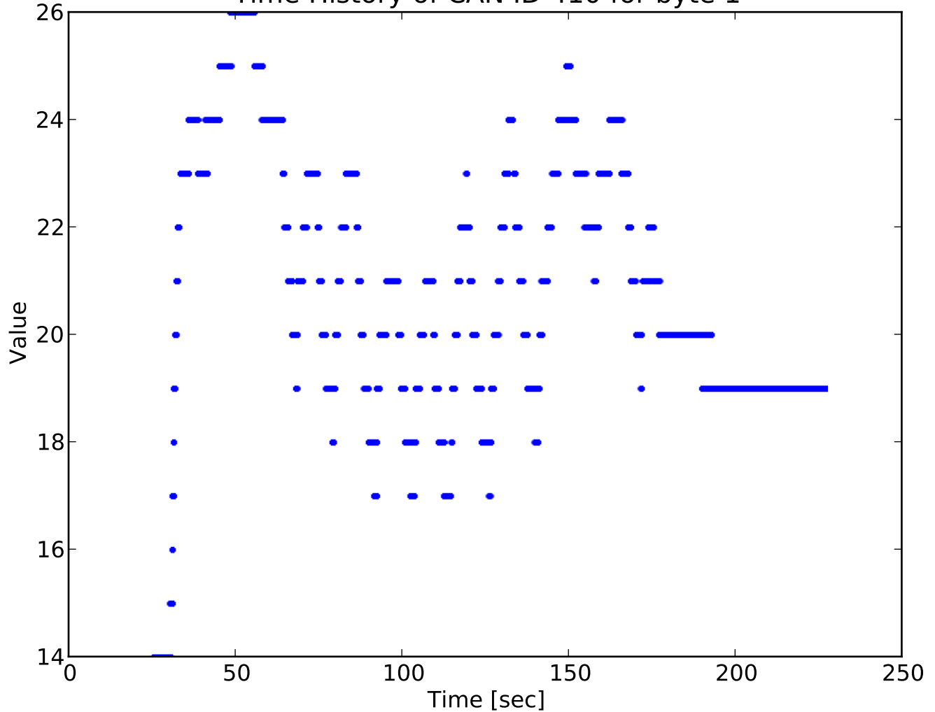
Time History of CAN ID 410 for byte 1
