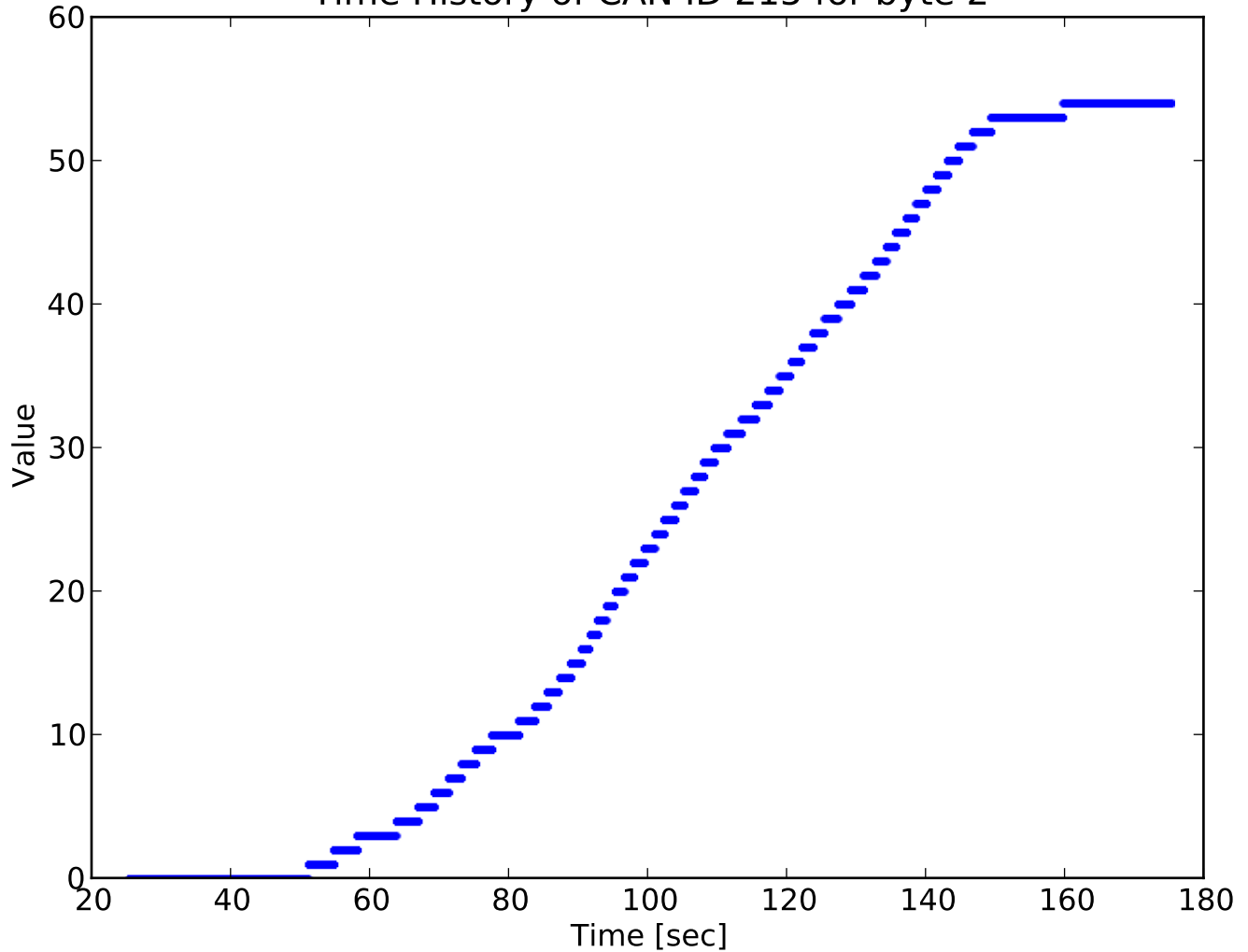
Time History of CAN ID 215 for byte 2
