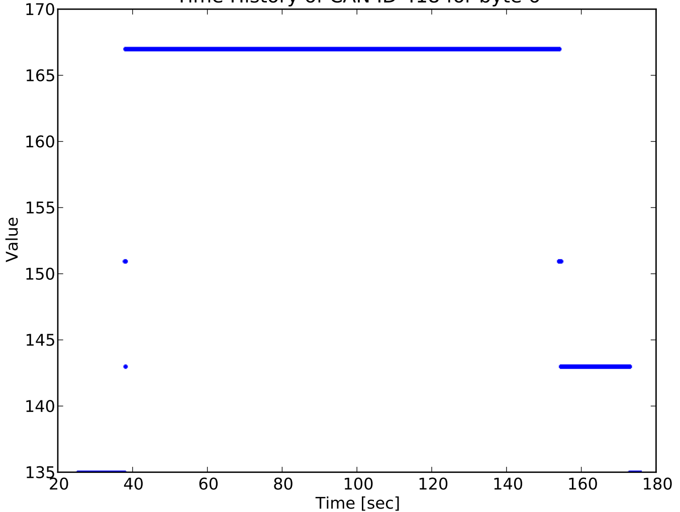
Time History of CAN ID 418 for byte 6
