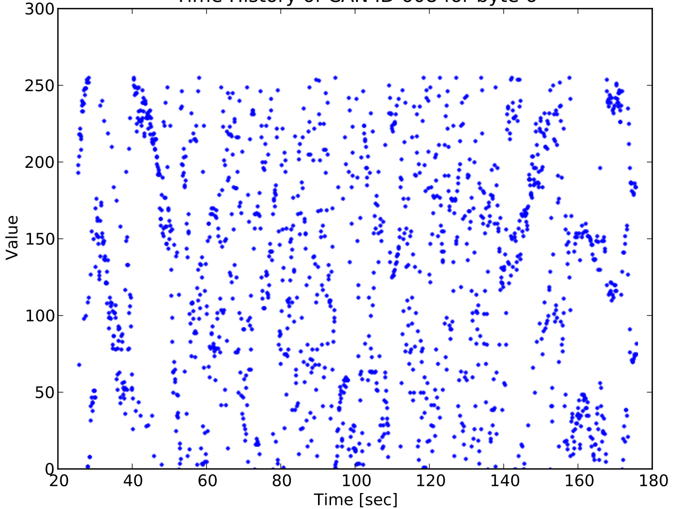
Time History of CAN ID 608 for byte 6
