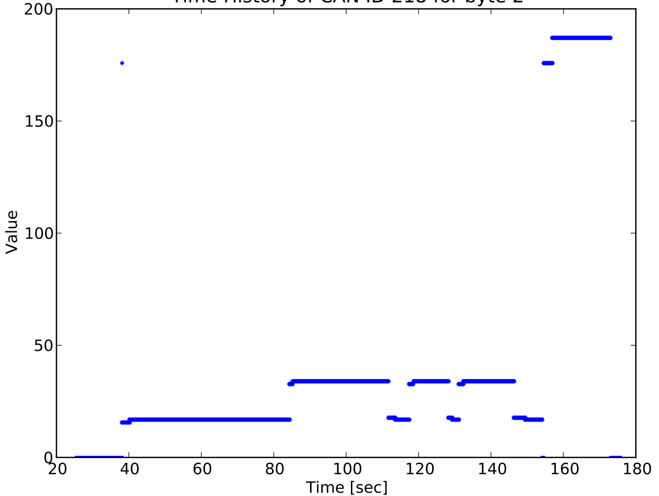
Time History of CAN ID 218 for byte 2
