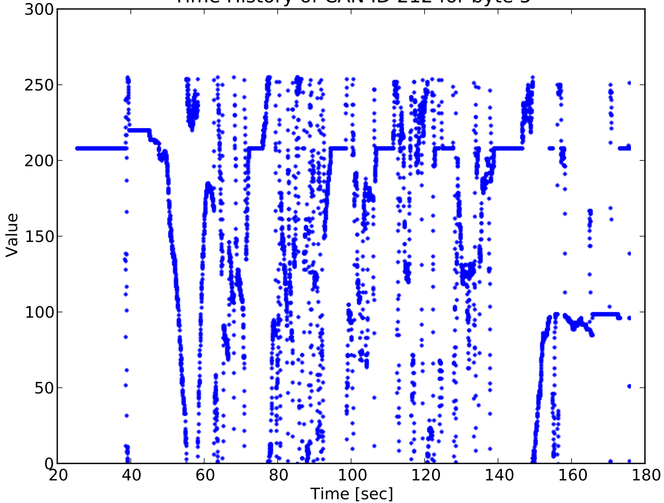
Time History of CAN ID 212 for byte 5
