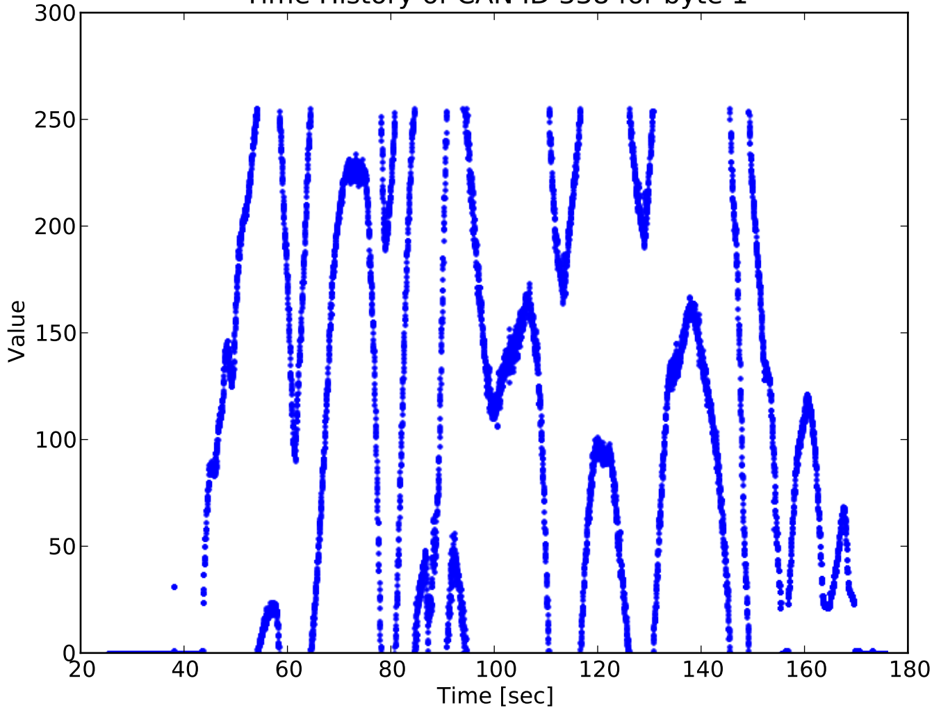
Time History of CAN ID 338 for byte 1
