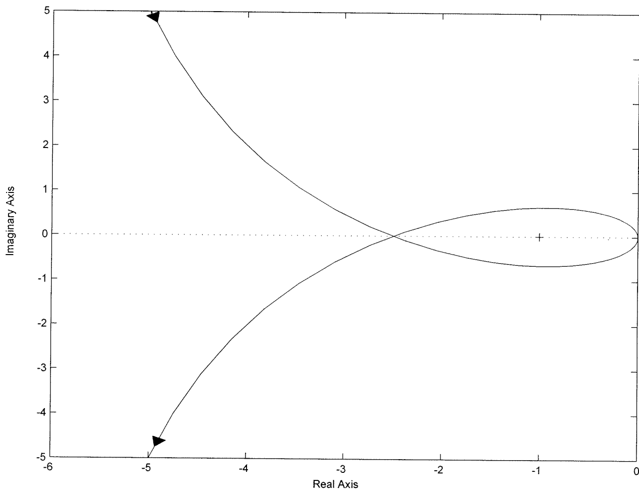
Nyquist Diagram
