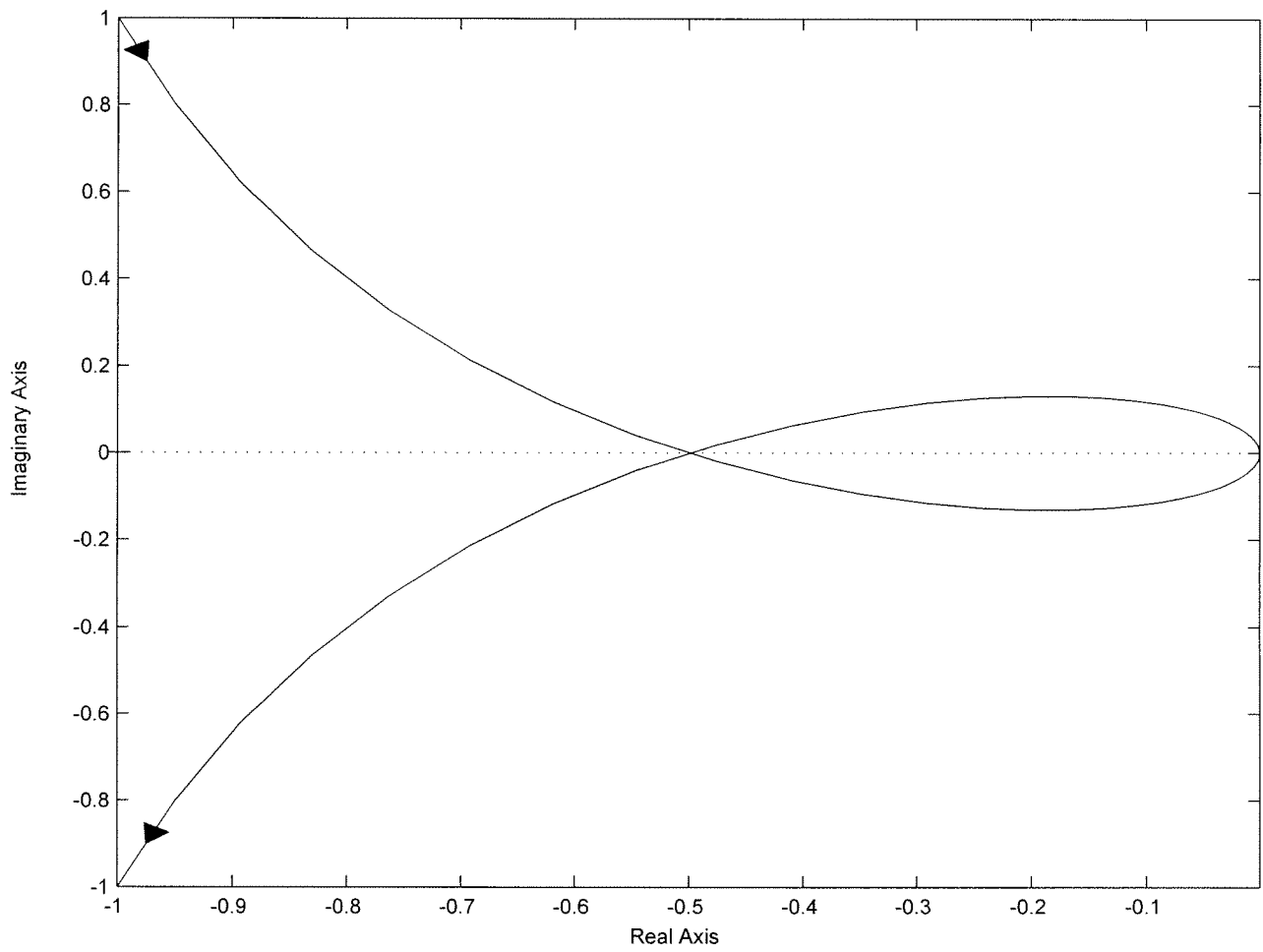
Nyquist Diagram
