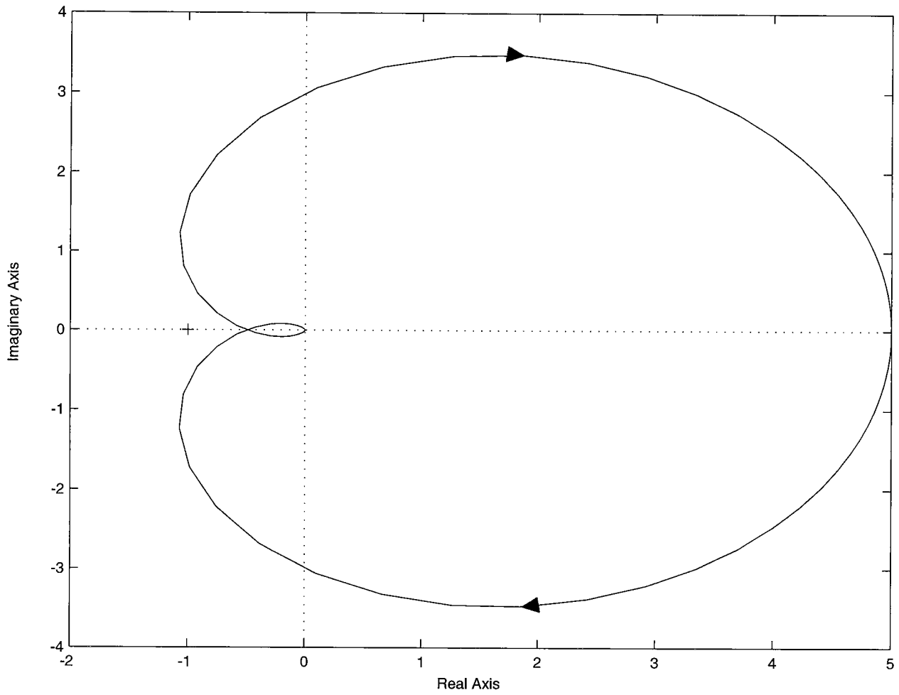
Nyquist Diagram
