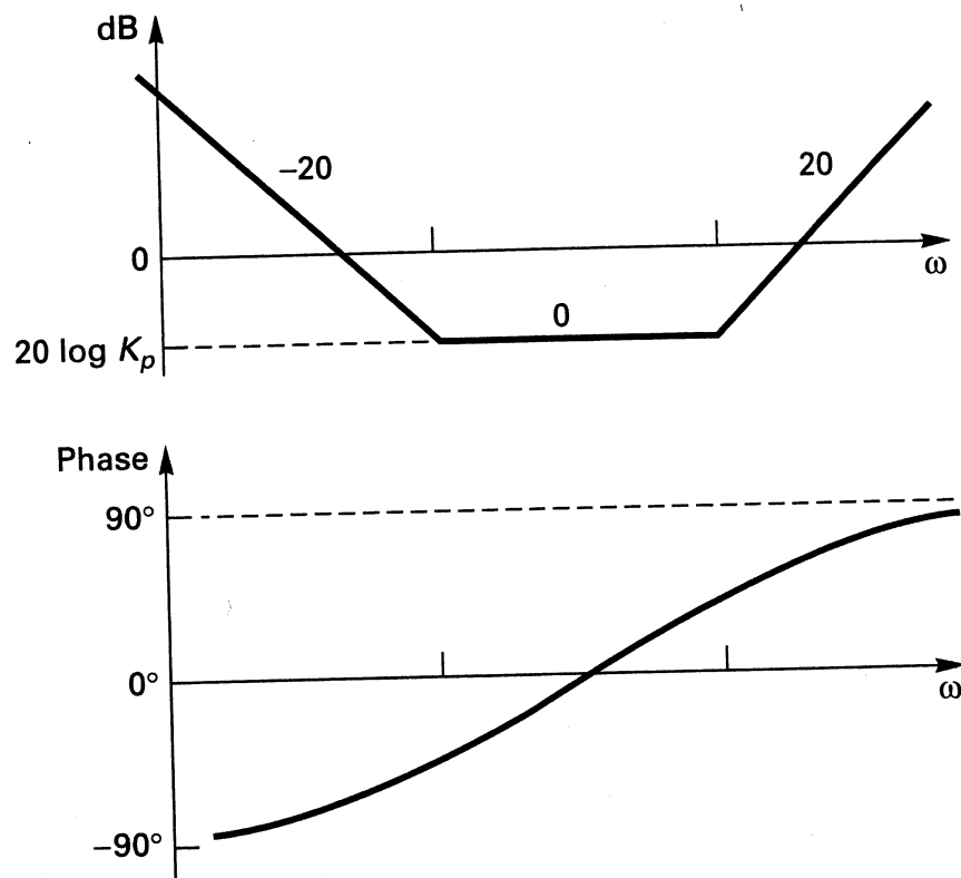
FIGURE 9.32 Bode diagram of PID controller.
