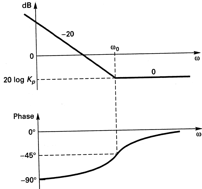
FIGURE 9.29 Bode diagram for PI controller.
