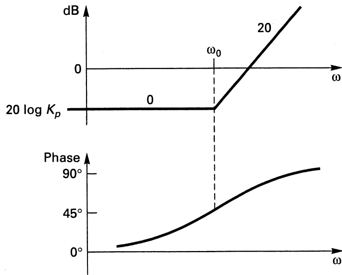
FIGURE 9.31 Bode diagram of PD controller.
