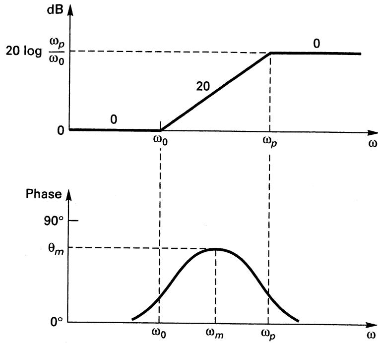
FIGURE 9.16 Bode diagram for phase-lead compensation.
