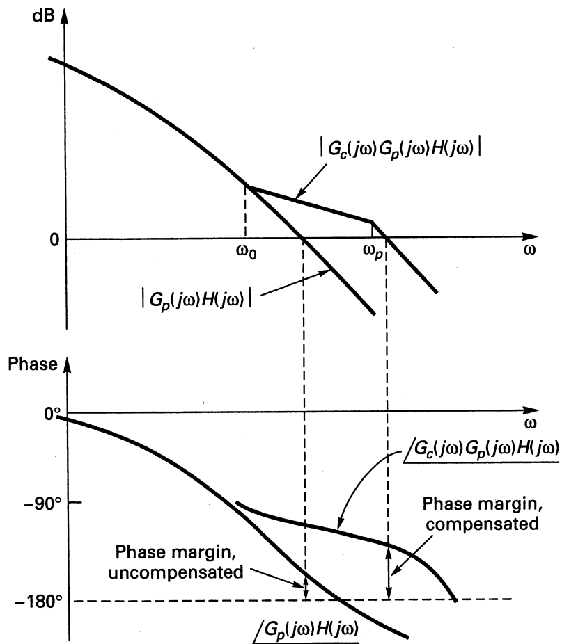
FIGURE 9.19 Phase-lead compensator design.
