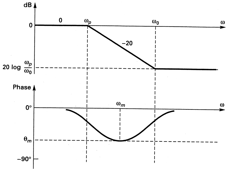
FIGURE 9.12 Bode diagram for phase-lag compensation.
