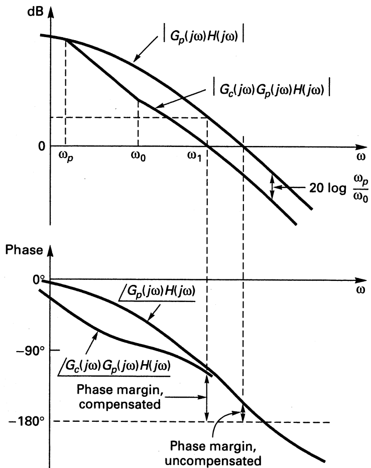
FIGURE 9.14 Phase-lag design.
