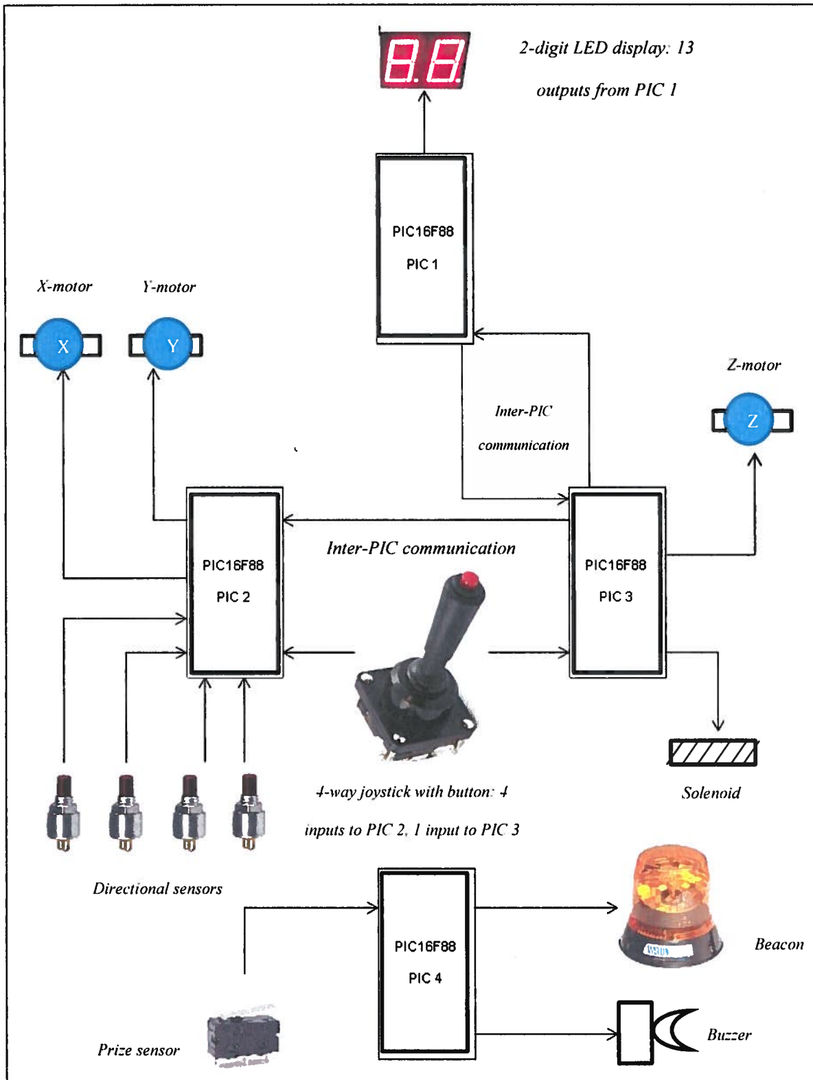
Figure 10: Skill crane functional diagram
