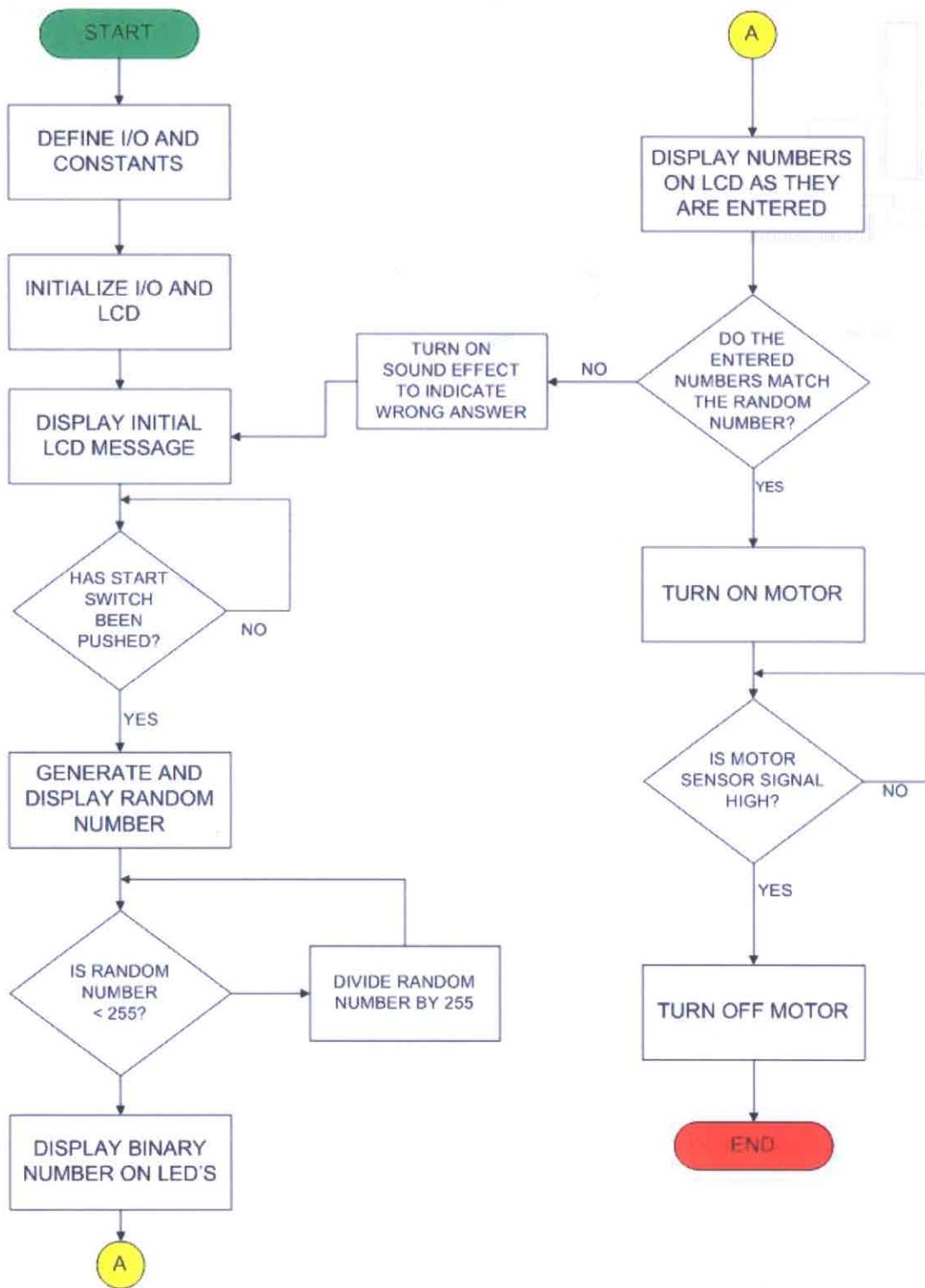
Figure 20 Software Flowchart
