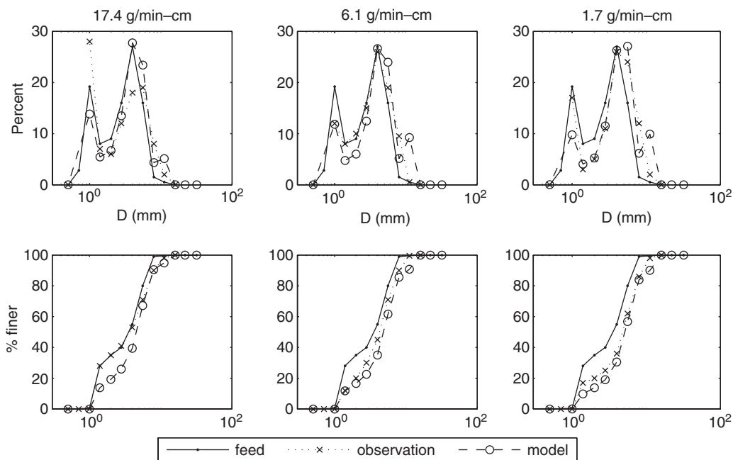
Figure 4. Probability (top) and cumulative (bottom) grain size distributions of the feed, the observed bed surface, and the bed surface predicted by the 1-D model, for the Dietrich et al. (1989) experiments.
