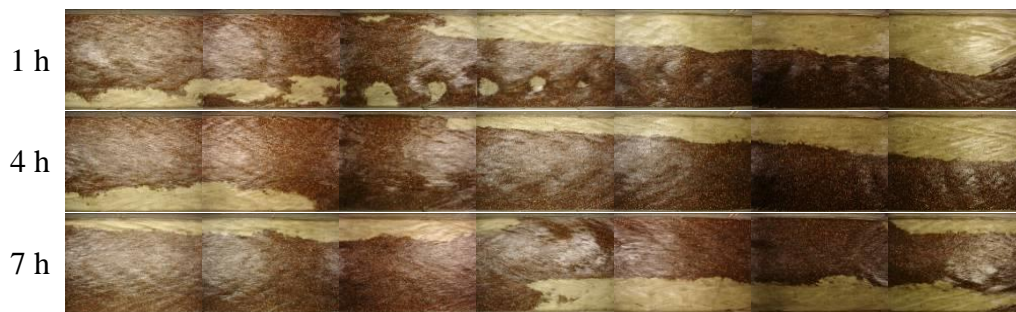
Figure 2.7. Time evolution of bedrock exposure Run 2-B4: Q_s = 97 g/s, q_s/q_c = 0.88 , and P_c = 0.78 [Chatanantavet and Parker, 2008 (personal communication)]. The channel is 0.9 m wide, 13 m long, water and sediment flow from left to right, and light and dark areas correspond to bedrock and sediment, respectively.
