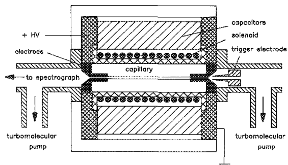
FIG. 1. Schematic diagram of the capillary discharge setup.
