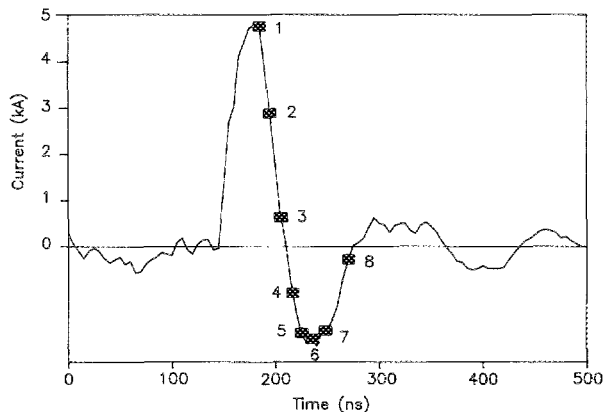
FIG. 2. Discharge current pulse corresponding to a 500- \mu\text{m} -diam lithium hydride capillary 38 mm in length excited by a 6.6 nF capacitor charged to 40 kV. The marks indicate the times at which spectra were obtained. The horizontal dimension of the marks represents the time error bars.
