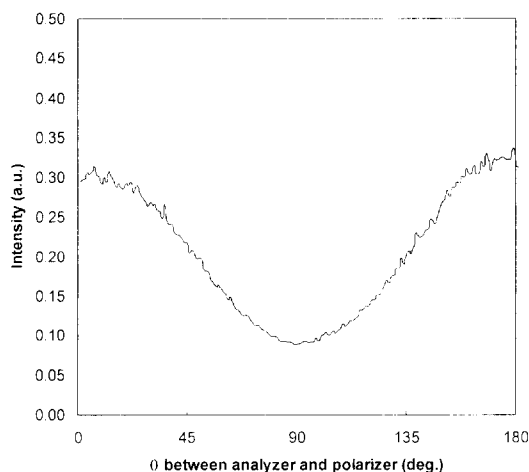
Figure 7. The experimentally measured intensity of the beam outgoing from the optical system as function of rotation angle.
