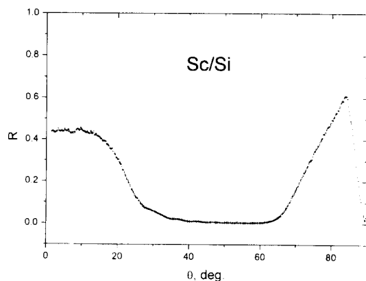
Figure 1. Reflectivity of a Sc/Si multilayer mirror as function of incidence angle.
