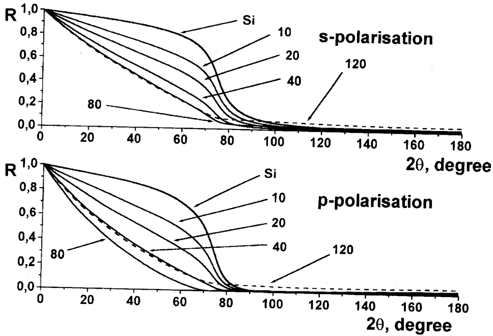
Figure2. Reflectivity of Si covered with oxide \text{SiO}_2 film at 0.154 nm and 46.9 nm. Numbers (10,20...) indicate film thickness in Å.
