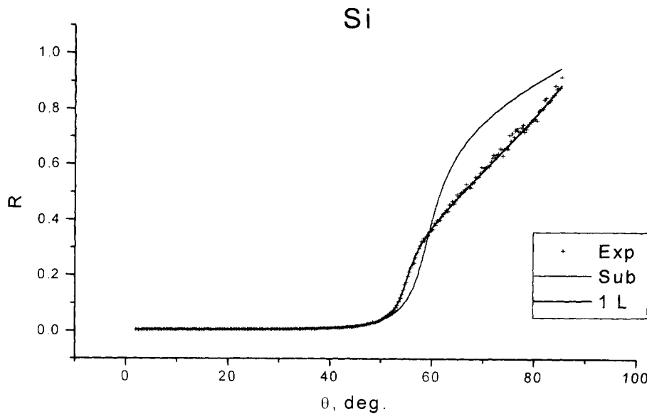
Figure 3. Reflectivity data for Si at 46.9 nm and results of fitting procedure Thin solid line — Fresnel formula for a clean surface, thick solid line — Fresnel formula with the account for contamination layer.
