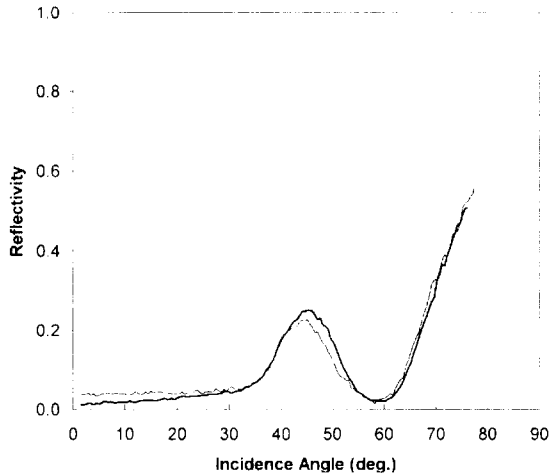
Figure 5. The reflectivities of two mirror used in the experiments.
