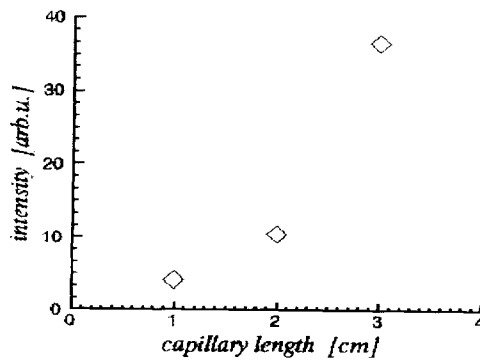
Figure 5. Maximum output signal vs. the capillary length.
