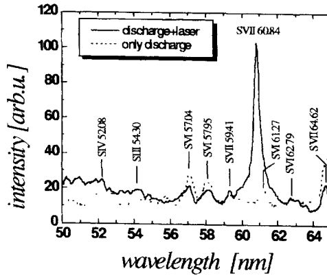
Figure 4. The spectra of the sulphur plasma measured at ~35 ns delay relative to the current peak for pure discharge (dotted line) and discharge irradiated by a picosecond laser pulse. The capillary length was 30 mm.
