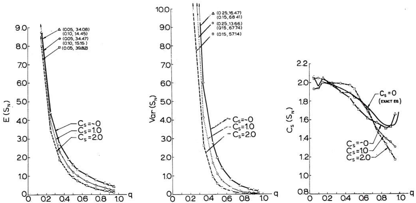
Fig. 6 Properties of run-sum for the independent standard normal variable ( C_s = 0 ) and the independent log-normal variable ( C_s = 1.0 and C_s = 2.0 ), obtained by the data generation method (Monte Carlo method): The mean, the variance and the skewness coefficient of S_n as function of q , for the above three values of C_s of x ( C_s = 0 ; C_s = 1 ; C_s = 2 ), respectively as the left, central and right graph.
