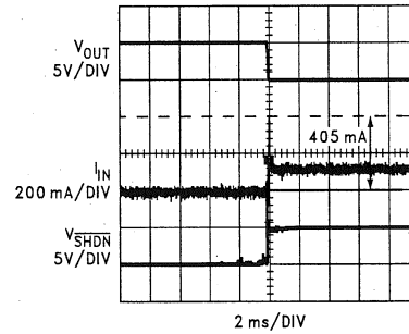
FIGURE 13. Start-Up Waveforms without Soft Start Circuit
