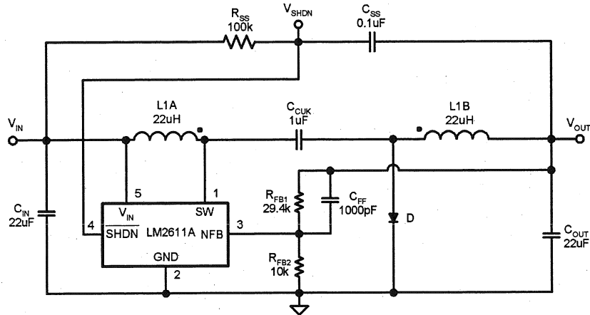
FIGURE 11. LM2611 Soft Start Circuit
