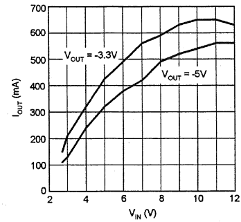
FIGURE 5. I_{OUT(MAX)} vs V_{IN} using 1oz. copper layout. See Figure 14 for the test circuit.
