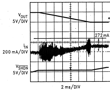
FIGURE 12. Start-Up Waveforms with Soft Start Circuit
