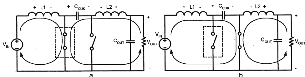
FIGURE 1. Operating Cycles of a Cuk Converter
