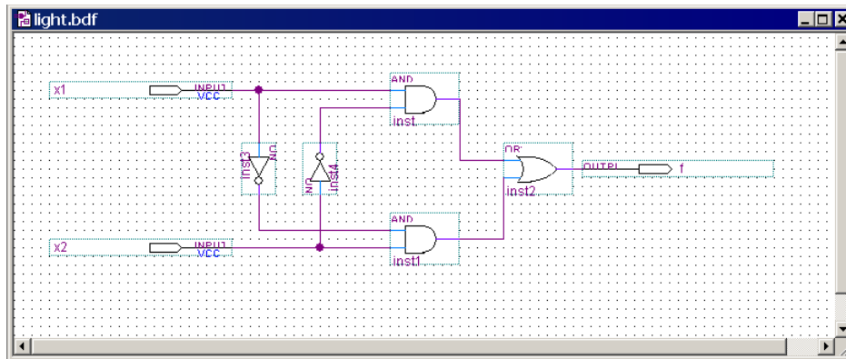
Figure 20. The completed schematic diagram.
