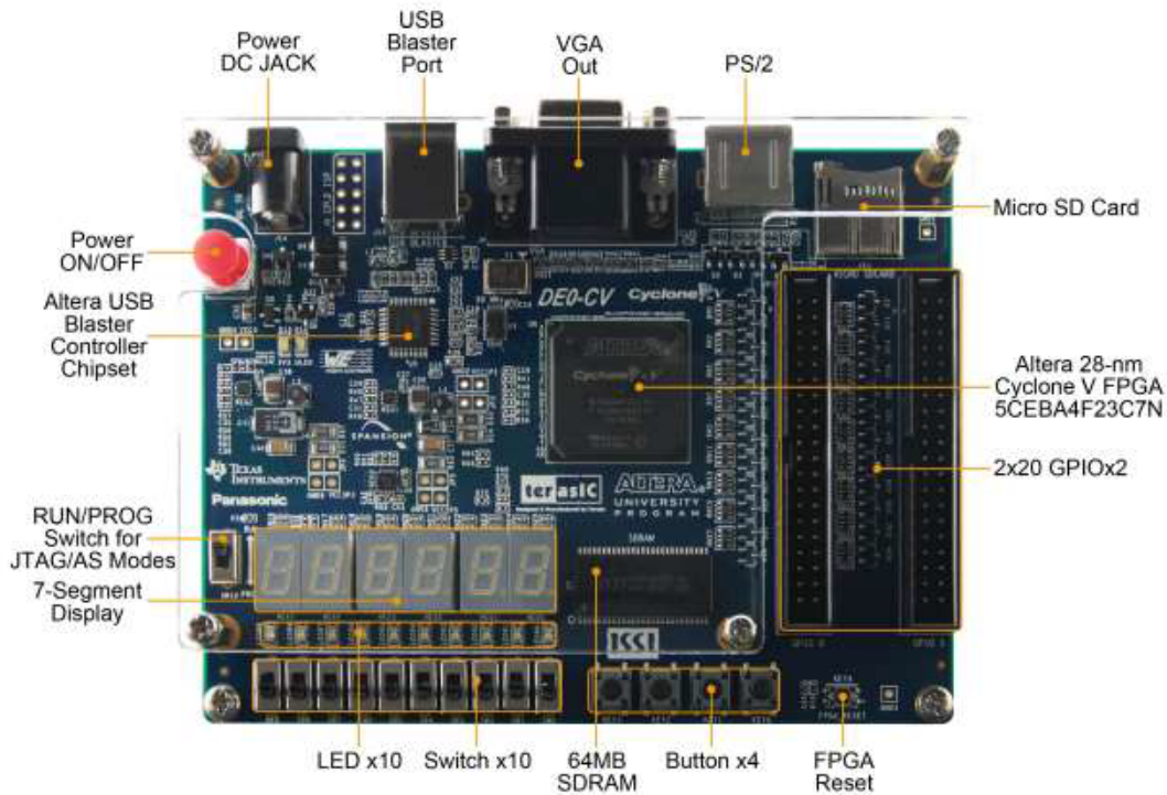
Figure 1 – Altera DE0 Development and Education Board
