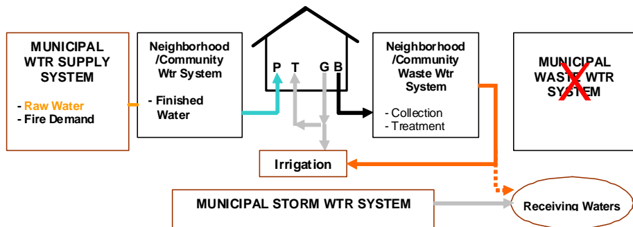
IV. Household Graywater Reuse in Neighborhood/Community Systems
