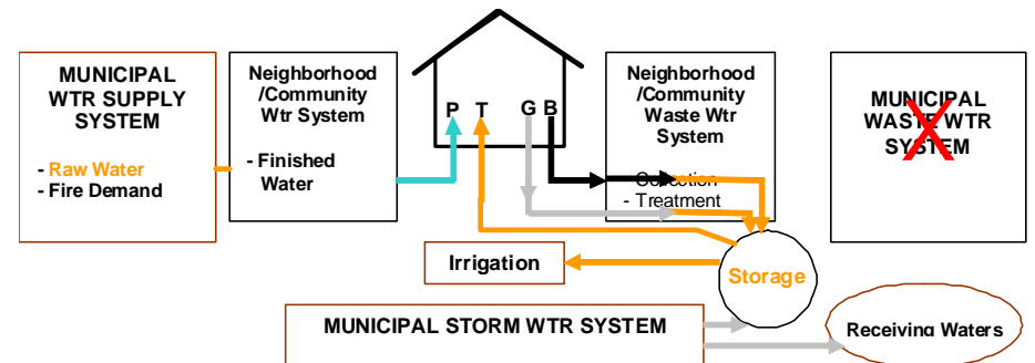
V. Completely Integrated, Distributed Neighborhood/Community Urban Water System
