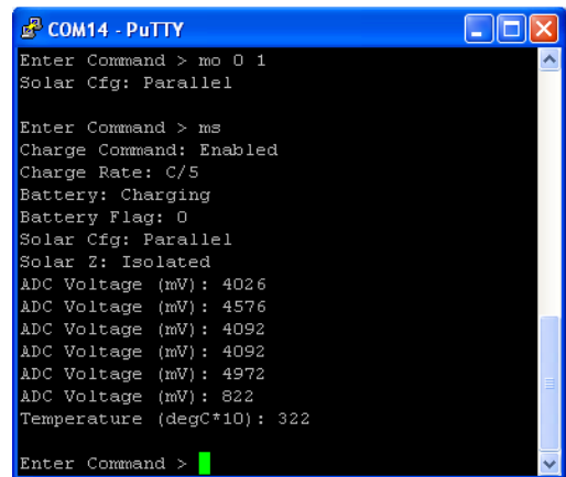
Figure 7: Solar Parallel Configuration
