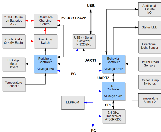
Figure 2: System Overview
