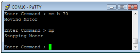
Figure 8: Both motors commanded forward at 27% speed
