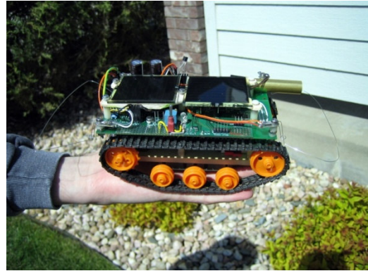
Figure 4: Rover Physical Size
