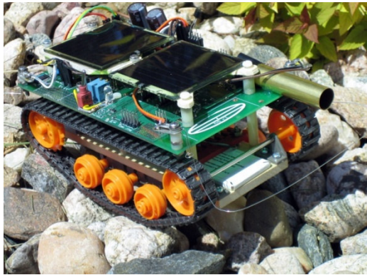
Figure 3: Rover Platform
