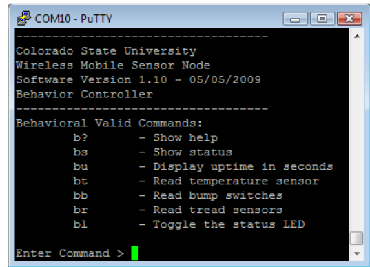
Figure 11: Behavioral Boot Up
