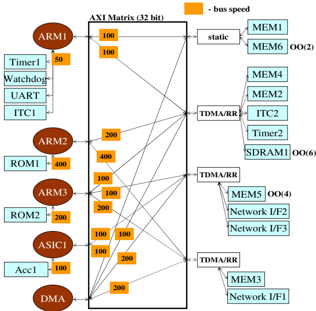
Fig. 13. Synthesized bus matrix for SIRIUS
