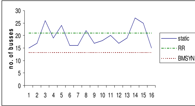
Fig. 11. Effect of ignoring arbitration space during bus matrix synthesis
