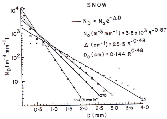
FIG. 9.5. Size distributions of snowflakes in terms of diameters of drops produced by melting the snowflakes. (From Gunn and Marshall, 1958.)
