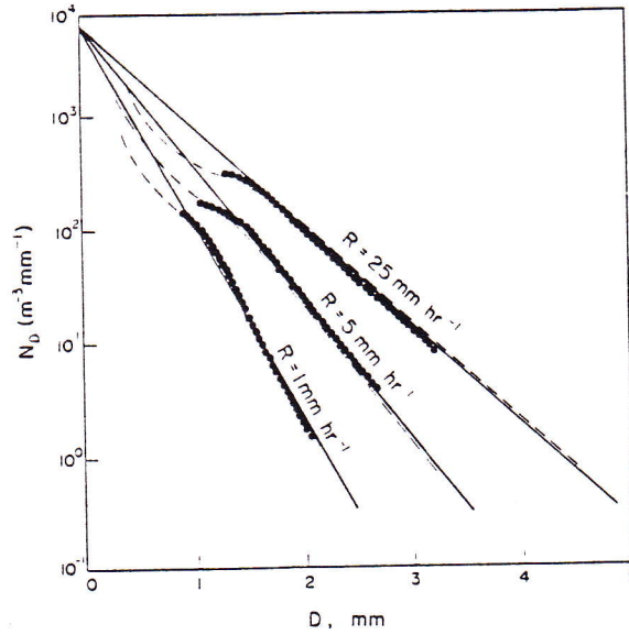
FIG. 9.2. Measured drop-size distributions (dotted lines) compared with best-fit exponential curves (straight lines) and distributions reported by others (dashed lines). (From Marshall and Palmer, 1948.)
