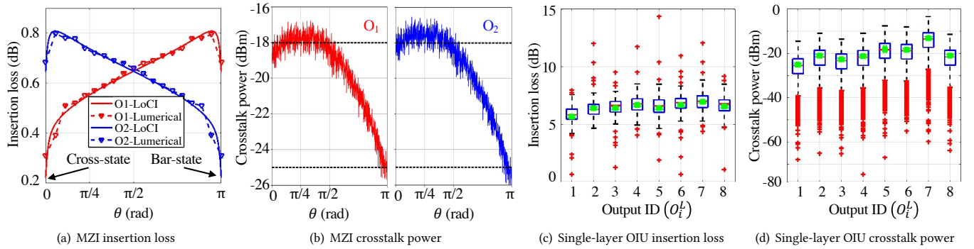
Figure 2: Insertion loss, (a), and crosstalk power, (b), at the output of the 2 \times 2 MZI in Fig. 1(b)-right simulated using the parameters listed in Table 1. Boxplots for the insertion loss, (c), considering 100 random weight matrices and the coherent crosstalk noise power, (d), analyzed at each output of the OIU in a single layer ( M = 1 ) with N = 8 (see Fig. 1(a)). Green dots show the average results.
