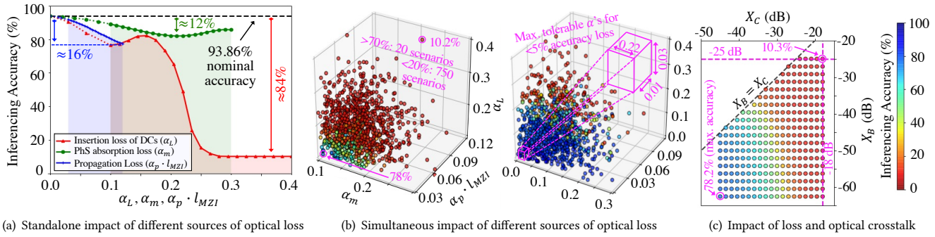
Figure 4: (a) SP-NN inferring accuracy in the presence of DC insertion loss (red), metallic absorption loss (green), and propagation loss in the MZI (blue)—see Table 1. In each case, only one source of optical loss is considered at a time. The \alpha 's are expressed in dB and the shaded regions represent their respective expected range (see Section 2.3). The dotted section of each plot shows the accuracy loss for lower \alpha 's (outside their expected range). (b) Left: Inferring accuracy when the loss parameters ( \alpha_L , \alpha_m , and \alpha_p \cdot l_{MZI} ) are simultaneously varied. Each of the 1000 points in the scatter plot represents an instance of the SP-NN where the \alpha 's are sampled from a half-normal distribution with mean, \mu = their minimum expected value and standard deviation, \sigma , such that 3\sigma = their maximum expected value. Right: Inferring accuracy when \alpha 's are sampled from a half normal distribution with mean, \mu = 0 , \sigma , such that 3\sigma = their maximum expected value. (c) Inferring accuracy in the presence of both optical loss and crosstalk noise for different values of X_B and X_C where X_B \leq X \leq X_C (see Section 3.1).
