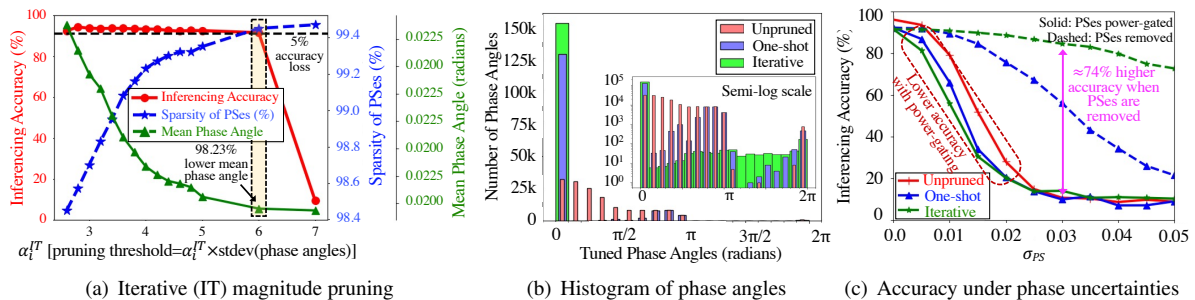
Fig. 3: (a) Fine-tuned inferring accuracy, PS sparsity, and mean phase angle for iterative pruning for different \alpha_i^{IT} . Yellow rectangle: best-performing IT-pruned model. (b) Histogram of the tuned phase angles in unpruned, best-performing one-shot-pruned, and best-performing iterative-pruned models. (c) Accuracy of the unpruned, best-performing one-shot-pruned, and best-performing iterative-pruned models under random phase uncertainties.
