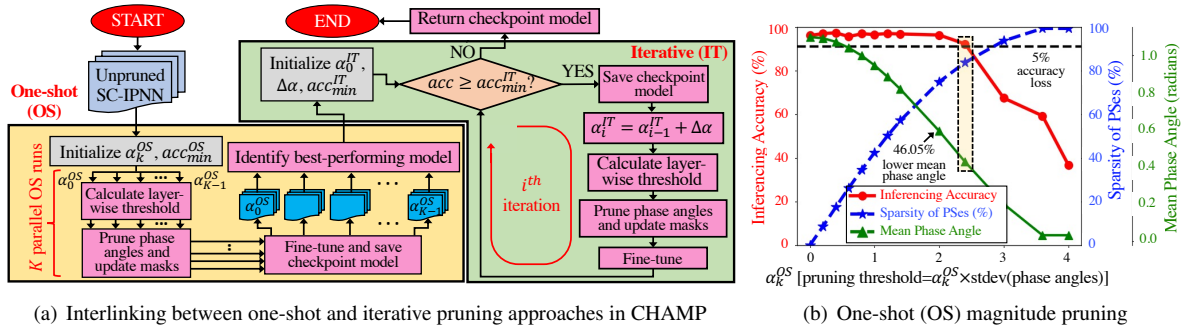
Fig. 2: (a) Block diagram highlighting the hybrid (one-shot and iterative) pruning approach in CHAMP. (b) Fine-tuned inferring accuracy, PS sparsity, and mean phase angle for one-shot magnitude pruning for different \alpha_k^{OS} . The yellow rectangle shows the best-performing (high sparsity and low accuracy loss) one-shot-pruned model.
