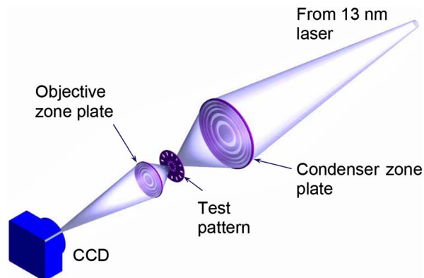
Fig. 1. (Color online) Schematic diagram of the 13 nm wavelength imaging system.
