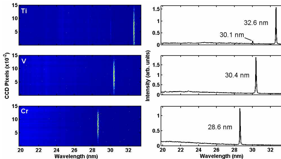
Fig. 1. Single shot on-axis spectra of 4 mm long line focus plasmas showing lasing in the 2p^3 3p^1 S_0 - 2p^2 3s^1 P_1 transition of Ne-like Ti, V and Cr ions. In all three cases, this laser-line dominates the spectrum.
