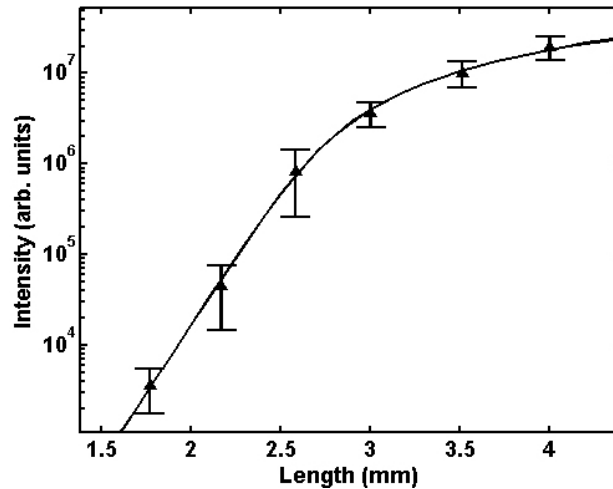
Fig. 4. Intensity of the 30.4 nm line of Ne-like V as a function of plasma length. Each point is the average of 10 or more shots. A fit of the data results in a gain coefficient of 72 \text{ cm}^{-1} and a gain-length product of 21.7. Each point is the average of 10 or more laser shots; the error bars correspond to \pm the standard deviation of the set.
