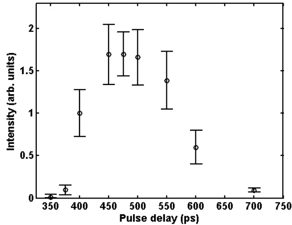
Fig. 3. Laser output intensity of the 30.4 nm line of Ne-like V as a function of time delay between the main pre-pulse and the short pulse. Lasing is strong for delays ranging from 400 ps to 600 ps. Each point is the average of 10 or more laser shots; the error bars correspond to \pm the standard deviation of the set.
