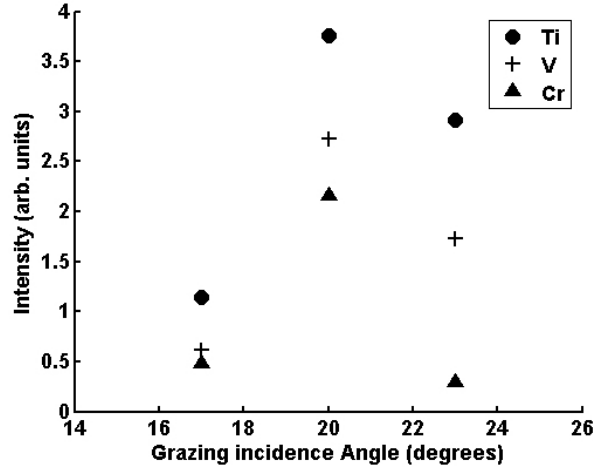
Fig. 2. Variation of output laser intensity as a function of grazing incidence angle for Ne-like Ti, V and Cr. Each point represents the mean of 15 or more consecutive laser shots. In all three cases the laser operates best at 20 degrees. At this angle the standard deviation of each data set ranges from 14% to 38% of the mean.
