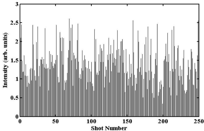
Fig. 5. Shot-to-shot variation of the intensity of the 30.4 nm Ne-like V laser line at 5 Hz repetition rate. The 250 consecutive shots have a distribution characterized by a standard deviation which is 35% of the mean.
