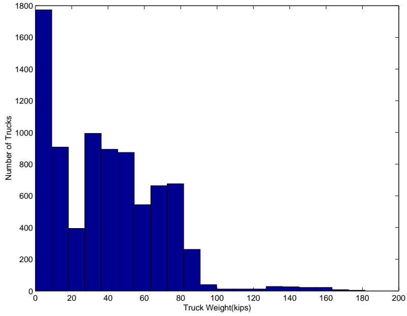
Figure 1-2: Gross Truck Weight Histogram for Bridge on I-94 over Pierce Road
