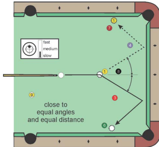
Diagram 5 Example rolling \frac{1}{2} -ball hit safety
