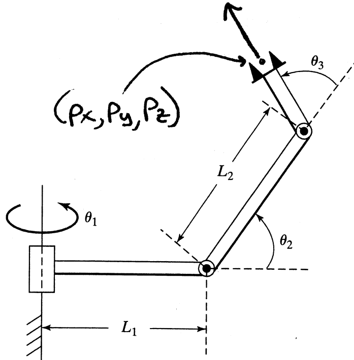
FIGURE 3.29: The 3R nonplanar arm (Exercise 3.3).
