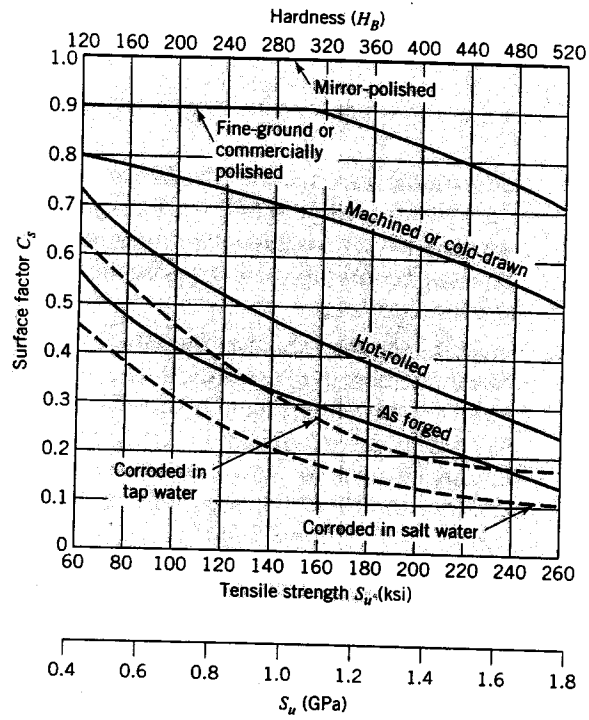
FIGURE 8.13 Reduction in endurance limit owing to surface finish—steel parts.
