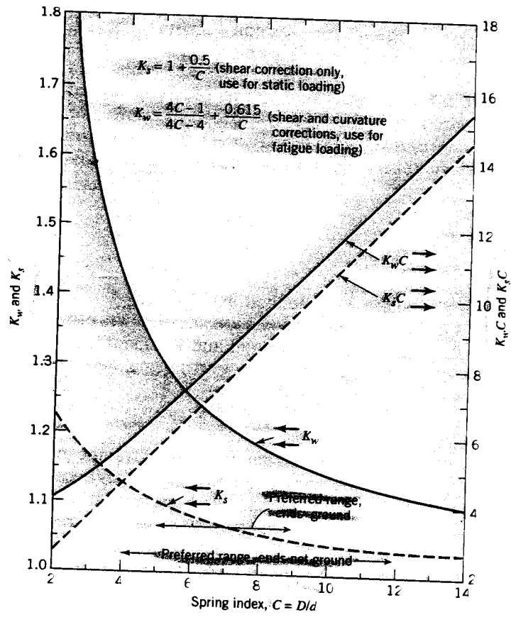
FIGURE 12.4 Stress correction factors for helical springs.
