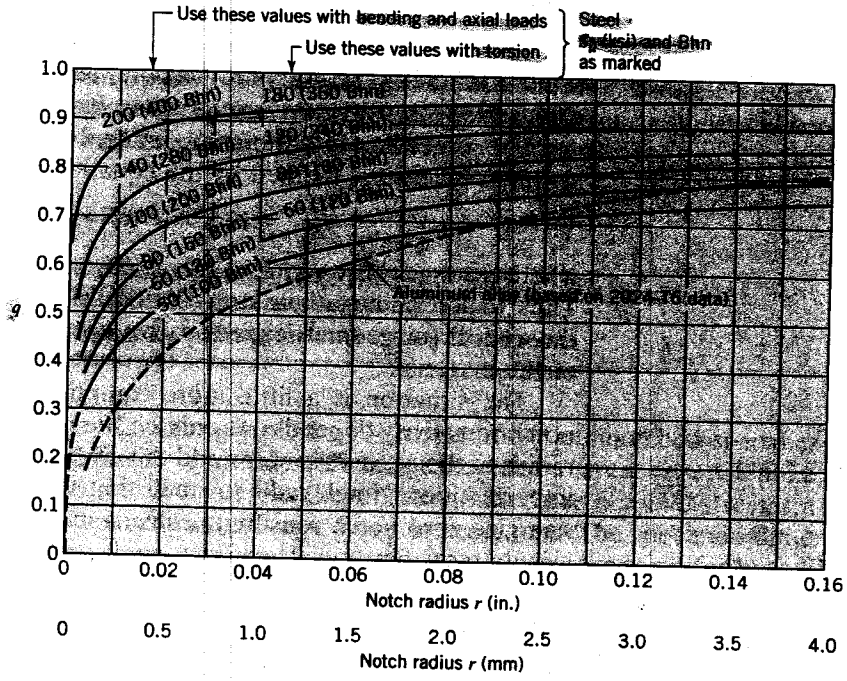
FIGURE 8.24 Notch sensitivity curves (after [9]). Note: (1) Here r is the radius at the point where the potential fatigue crack originates. (2) For r > 0.16 in., extrapolate or use q \approx 1 .
