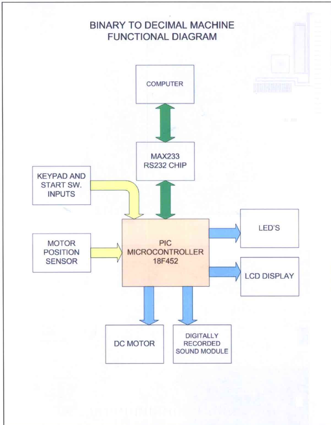
Figure 5 Functional Diagram
