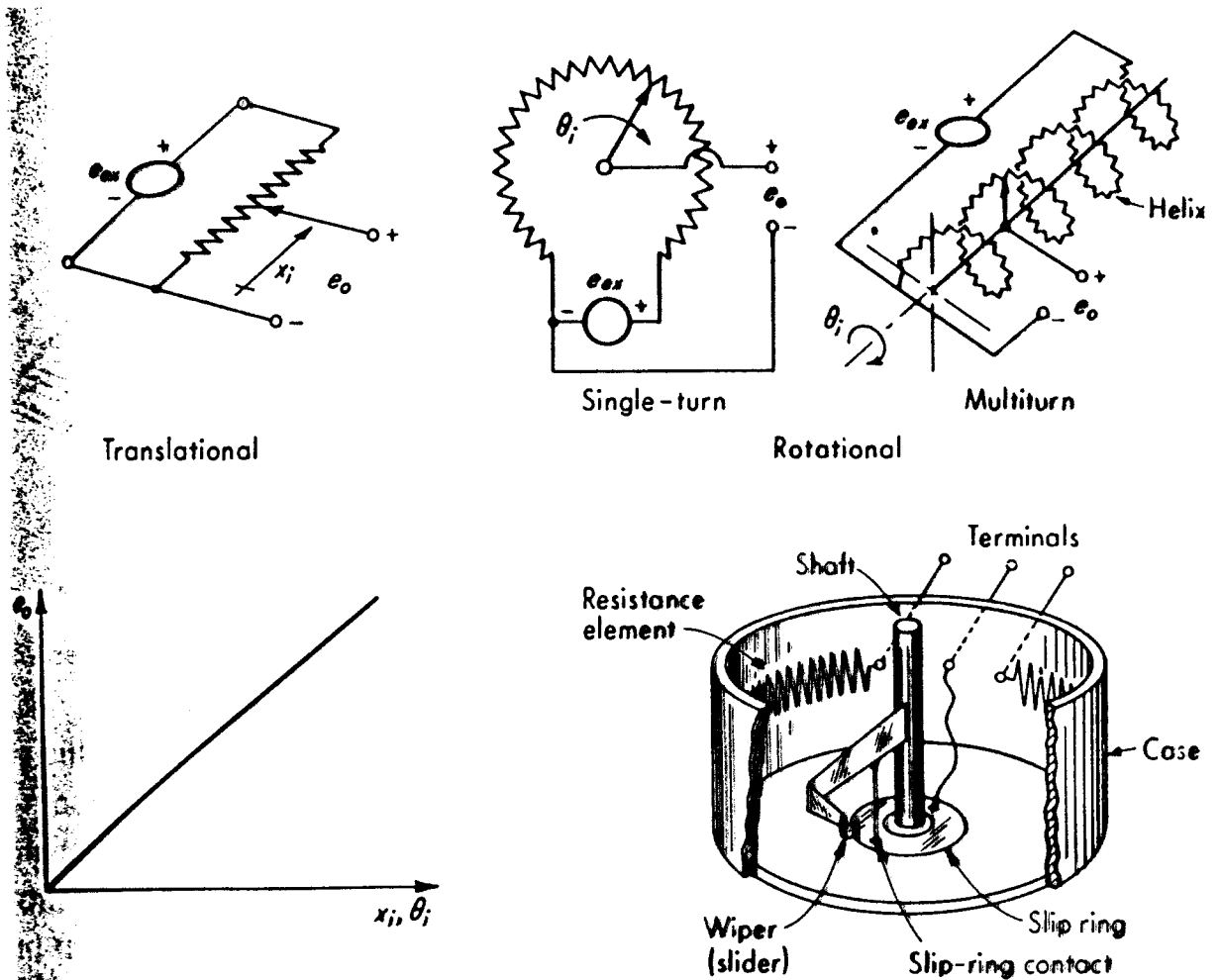
Figure 4.4 Potentiometer displacement transducer.
