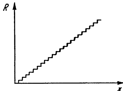
Figure 4.7 Resolution of wirewound potentiometers.
