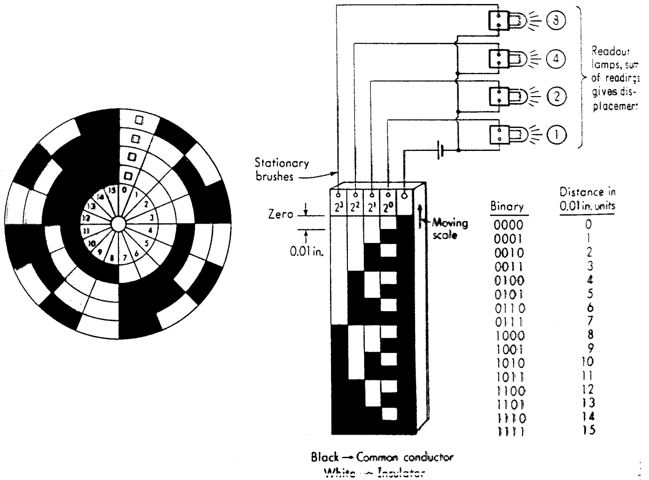
Figure 4.64 Translational and rotary encoders.
