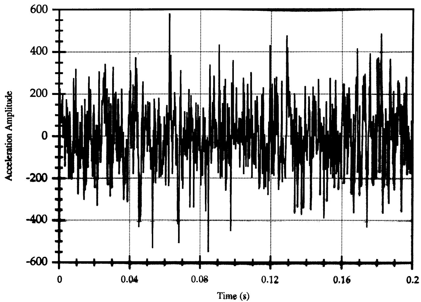
Data from bad bearing
