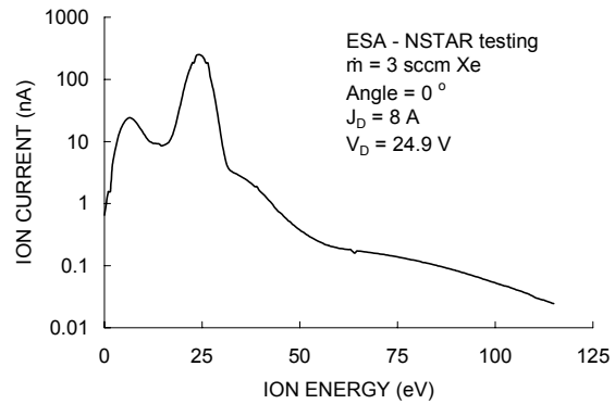
Fig. 4b) Ion energy distribution shown on a log-linear scale.
