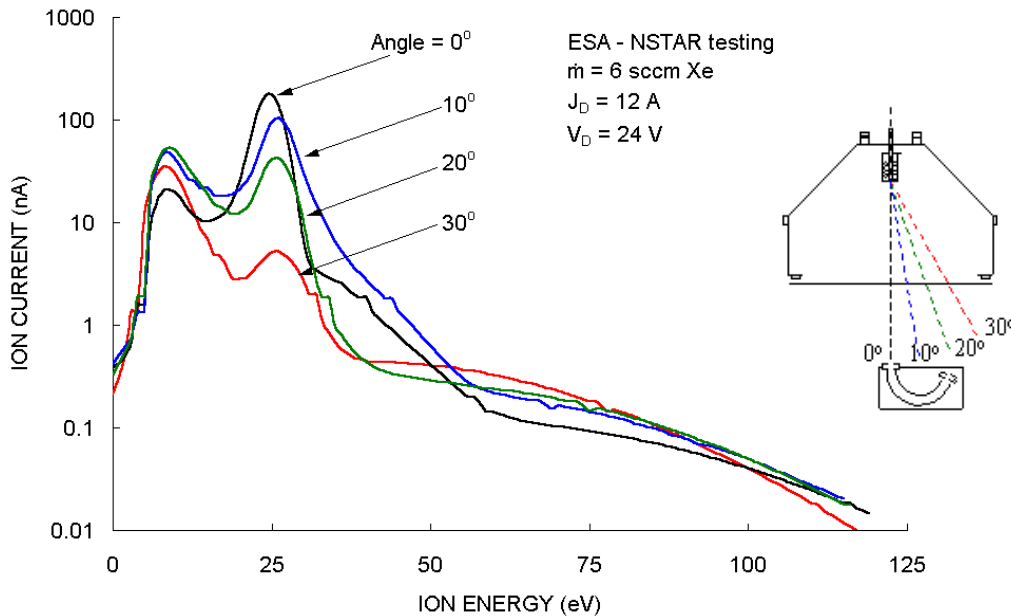
Fig. 5 Effect of zenith angle on the ion energy distribution function.
