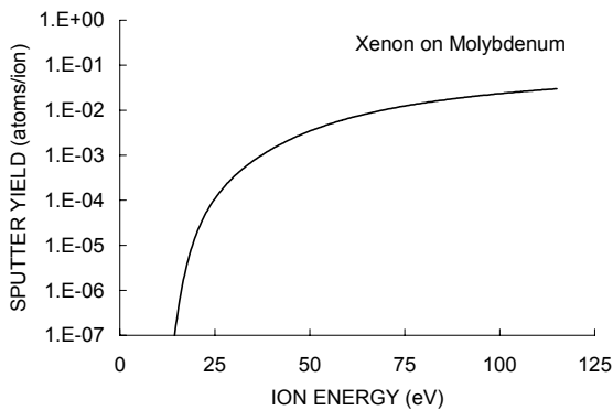
Fig. 4c) Sputter yield data for xenon on molybdenum.
