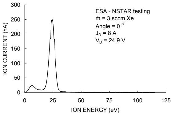
Fig. 4a Typical ESA ion energy distribution function (linear-linear scale).
