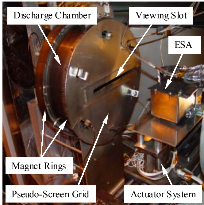
Fig. 1b Photograph of experimental apparatus.
