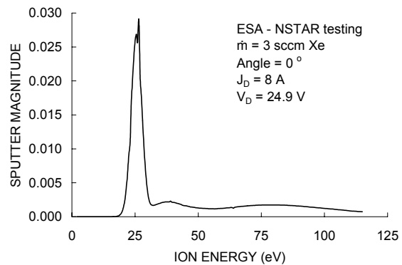
Fig. 4d) Magnitude comparison of sputtering caused by each ion group.
