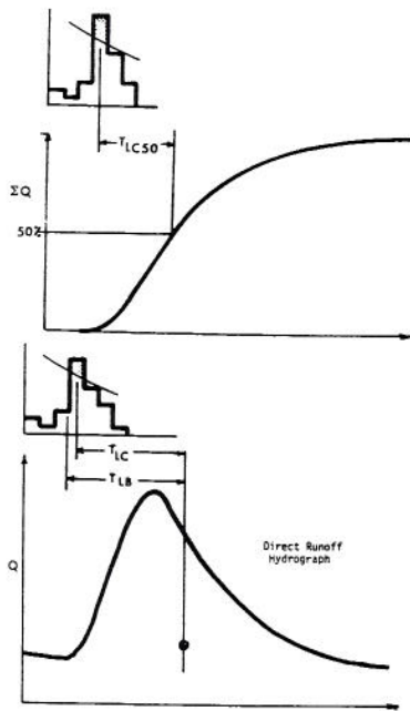
Fig. 4. Definition Sketch for Lag Time
