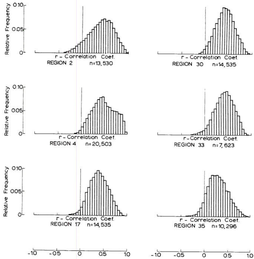
Fig. 14 Distributions of inter-station correlation coefficients for precipitation gross subdivisions, numbers 2, 4, 17, 30, 33 and 35 (n is the number of computed coefficients).
