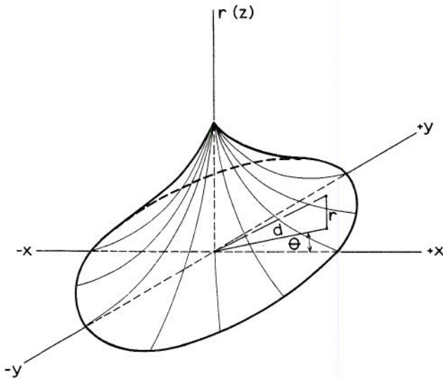
Fig. 11 Diagram of surface elements.
