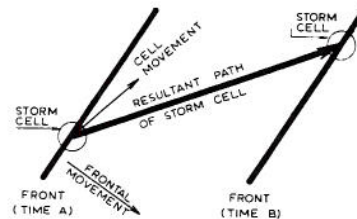
Fig. 7 Resultant frontal storm path.
