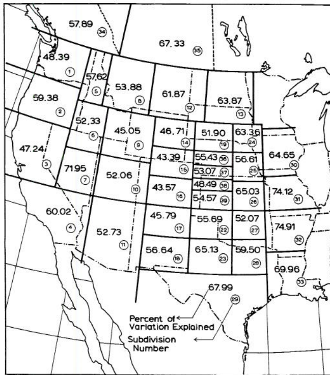
Fig. 3 Delineation of the net subdivisions and the average value of the variation in the correlation coefficients explained by regression for precipitation.
