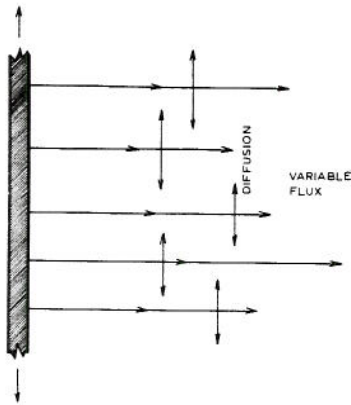
Fig. 6 Line moisture source.
