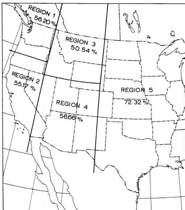
Fig. 4 Delineation of the net subdivisions and the average value of the variation in the correlation coefficients explained by regression for effective precipitation.
