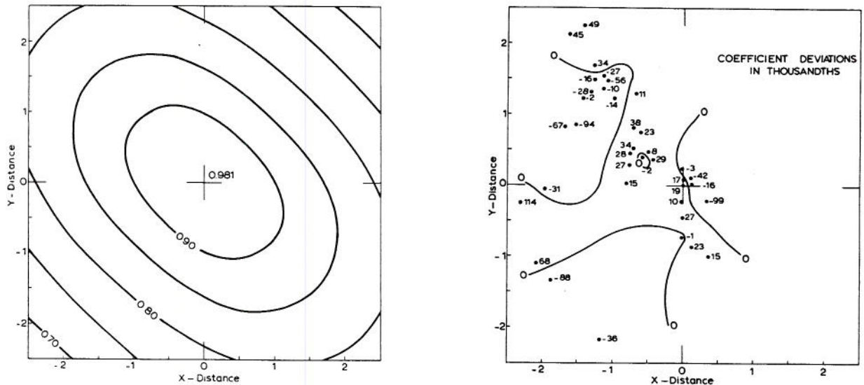
Fig. 18 Isolines of inter-station coefficients for the selected function (EP-series, NS = 153) Y = 0.98 \text{ Exp} [(-0.087 + 0.002 \cos 2\theta - 0.021 \sin 2\theta)d] , 65.47 percent of the variation explained by regression (Top, left) and the deviations of the actual coefficients (Fig. 1) from the fitted surface (Top, right).
