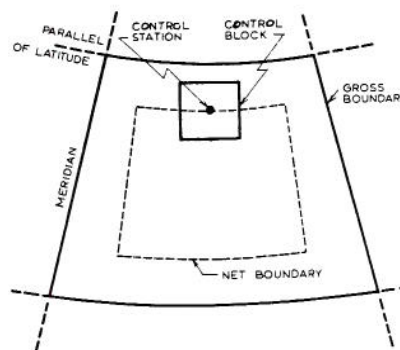
Fig. 2 Portrayal of the working subdivisional elements.
