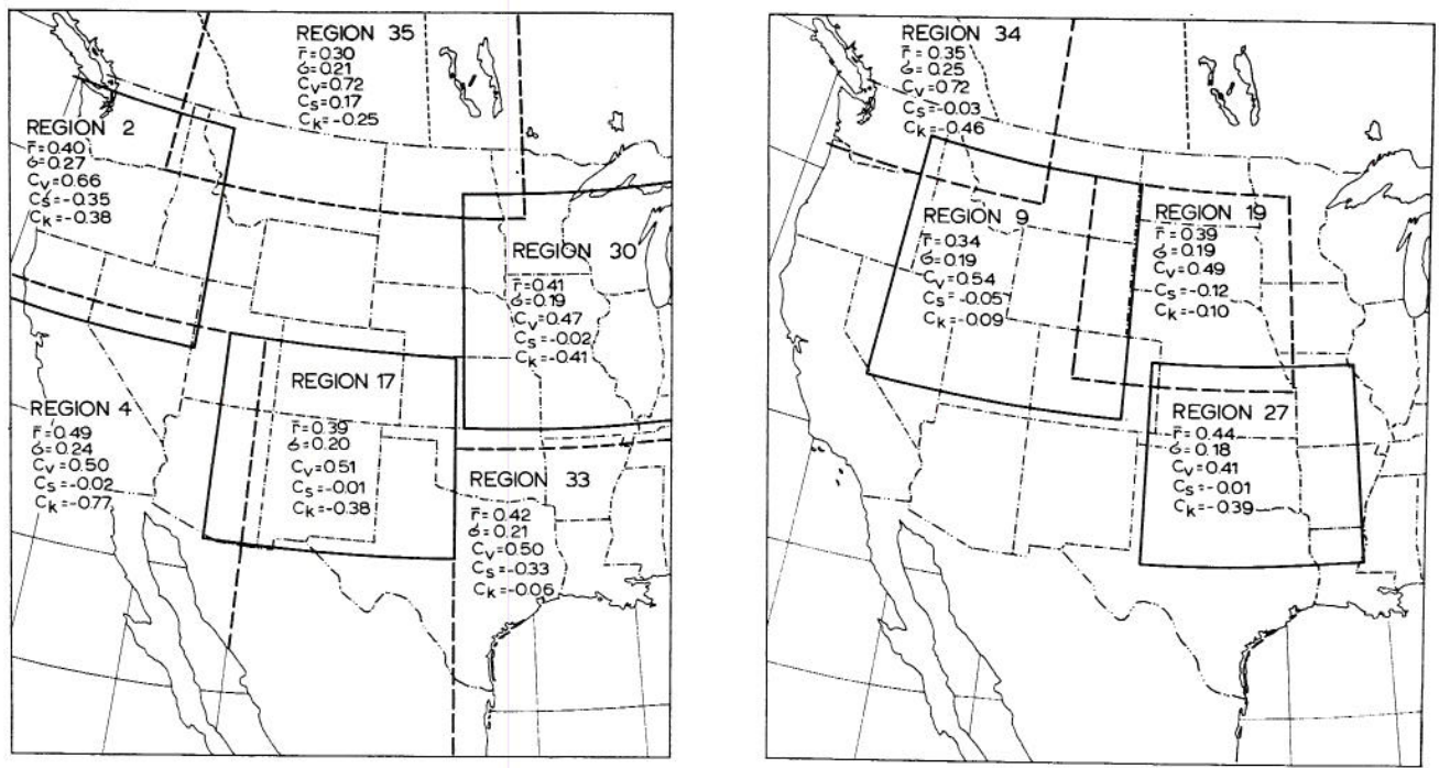
Fig. 13 Delineation of the selected gross subdivisions for precipitation and the statistics for the distributions of the inter-station correlation coefficients between all stations in each of the gross subdivisions.
