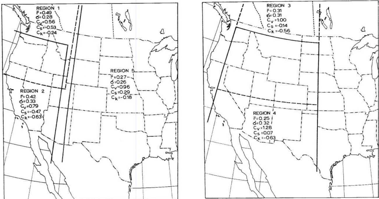
Fig. 16 Delineation of the gross subdivisions for effective precipitation and the statistics for the distributions of the inter-station correlation coefficients between all stations in each of the gross subdivisions.
