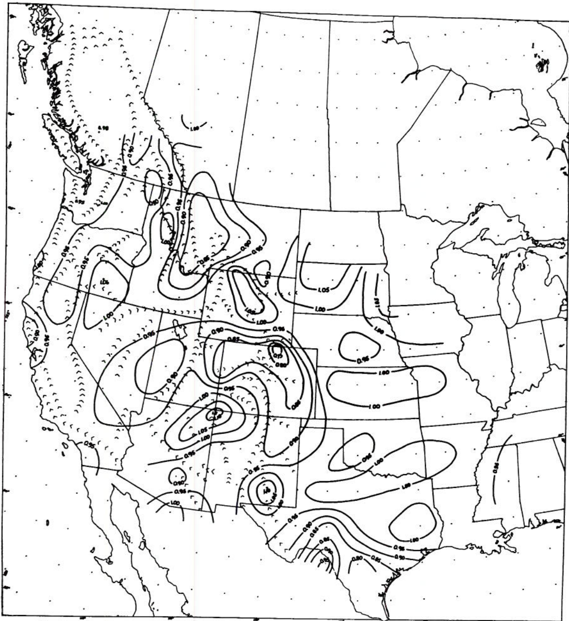
Fig. 28 Regional distribution of the regression coefficient a_1^1 for the annual effective precipitation variable.
