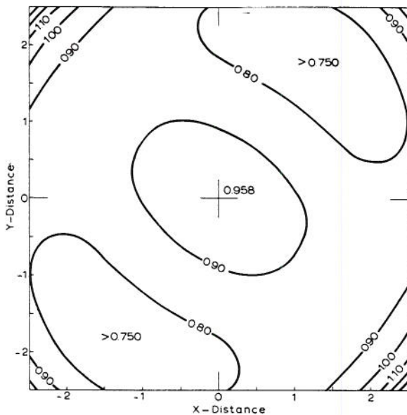
Fig. 12 Isolines of inter-station coefficients for an irrational fit (EP-series, NS = 153) Y = (1.04 - 0.7d + 0.19d^2 - 0.01 \cos 2\theta + 0.03 \sin 2\theta)^{-1} , 75.25 percent of the variation explained by regression (fitted to the data of fig. 1).
