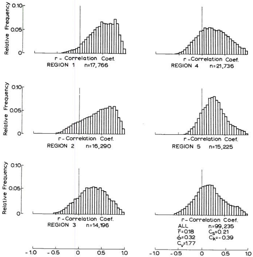
Fig. 17 Distributions of inter-station correlation coefficients for the effective precipitation gross subdivisions and the total area (n is the number of computed coefficients).
