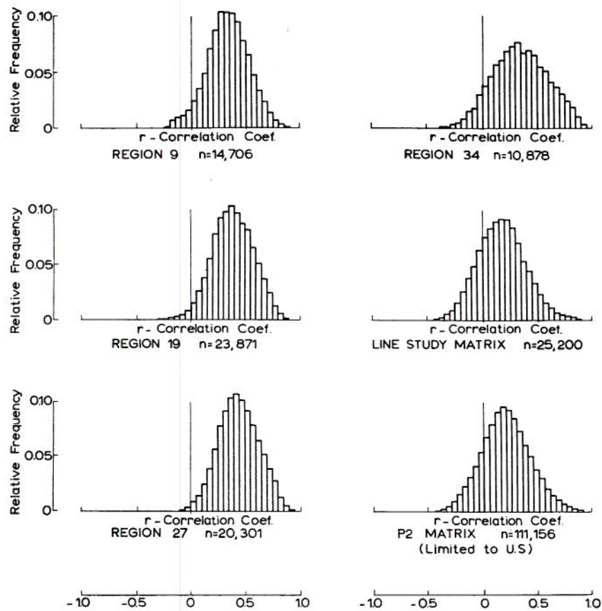
Fig. 15 Distributions of inter-station correlation coefficients for precipitation gross subdivisions, numbers 9, 19, 27, 34, line study subsample, and nonhomogeneous sample (n is the number of computed coefficients).
