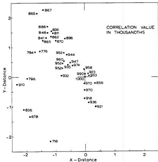
Fig. 1 Raw inter-station correlation coefficients (EP-series) plotted at their respective station locations. Each unit of distance (X or Y) is approximately equal to 60 nautical miles.
