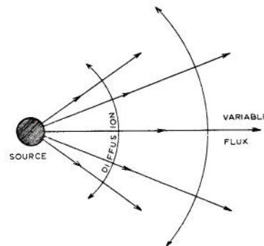
Fig. 5 Point moisture source.
