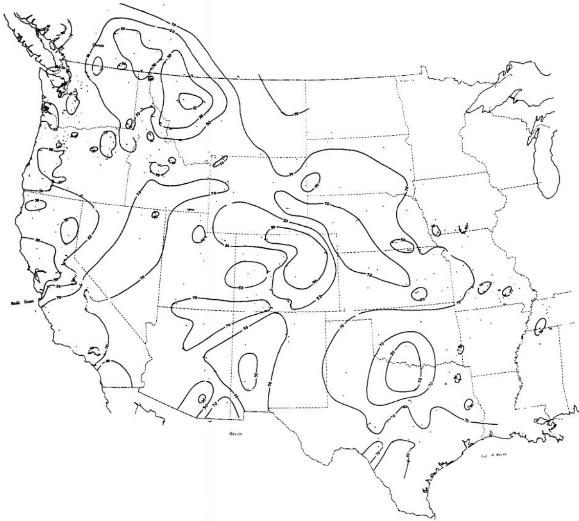
Fig. 23 Regional distribution of the percentage of the variation in the inter-station correlation coefficients explained by regression for the annual effective precipitation variable.
