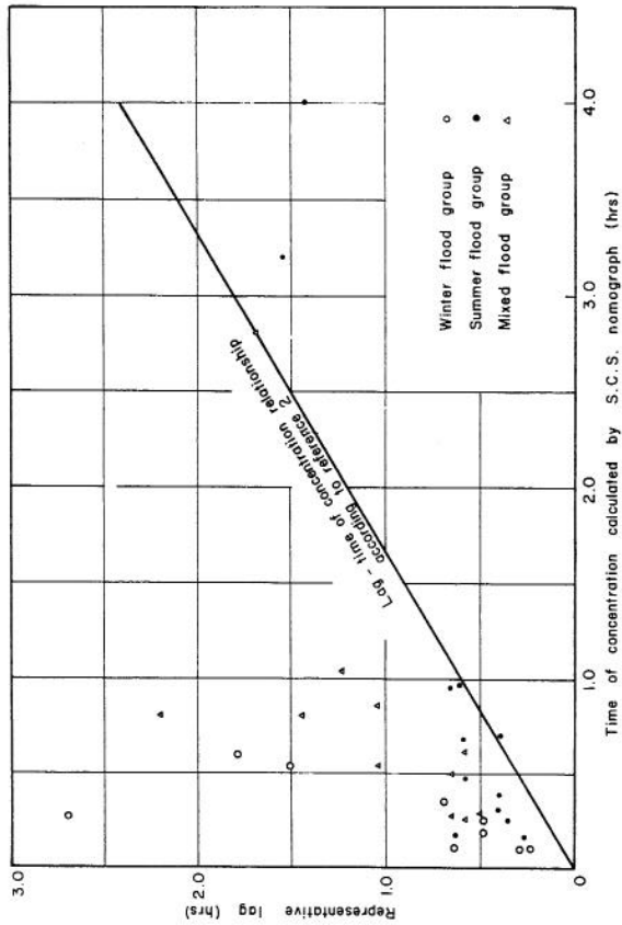
Fig. 9 Lag - time of concentration relationship
