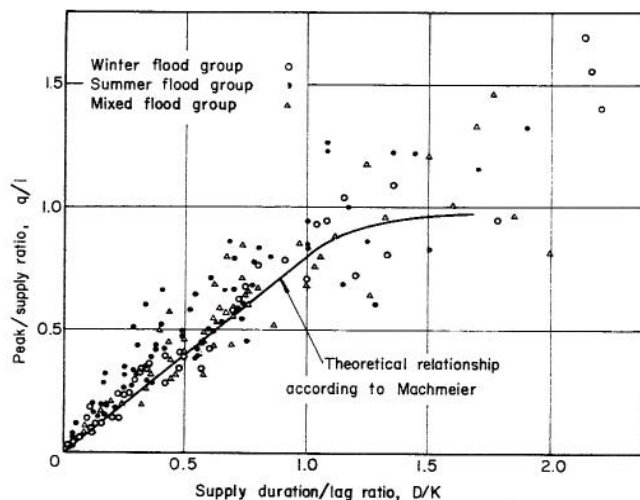
Fig. 4 Dimensionless peak/supply relationship for all floods
