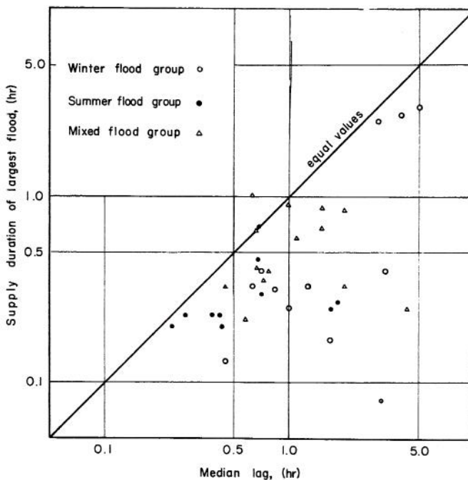
Fig. 13 Lag - duration correlation
