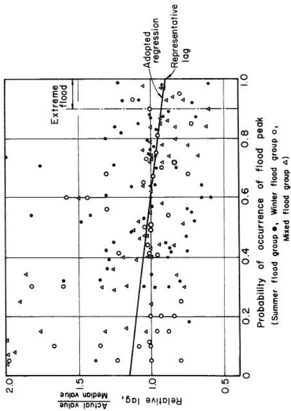
Fig. 7 Lag - probability relationship
