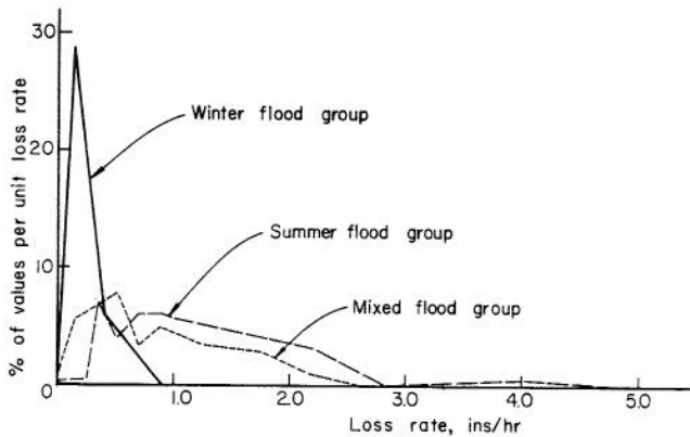
Fig. 16 Loss rate distributions for sample watersheds
