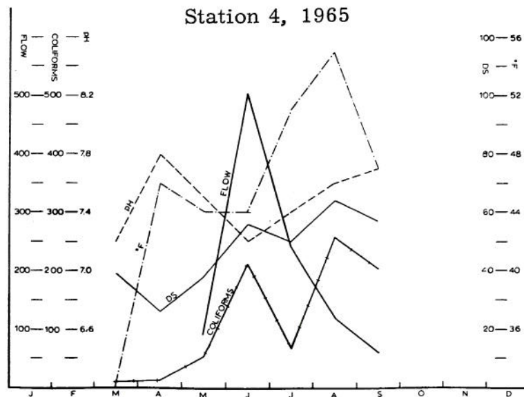
Figure E-- Monthly mean values plotted for flow, pH, temperature, dissolved solids, and coliform bacteria for Station 4, 1964 and 1965.
