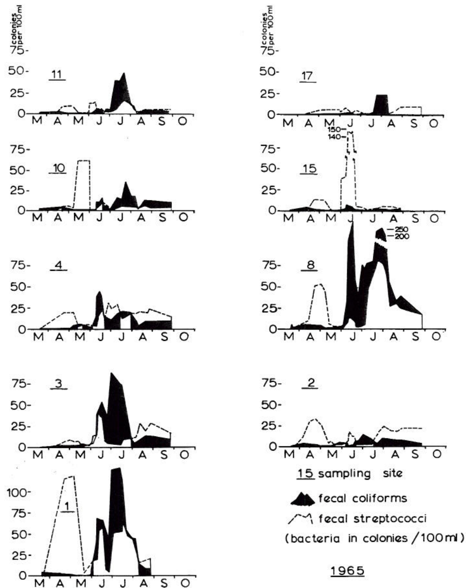
Figure 26--Moving means (three consecutive samples) for fecal streptococcus and fecal coliform bacteria concentrations, by stations, 1965.
