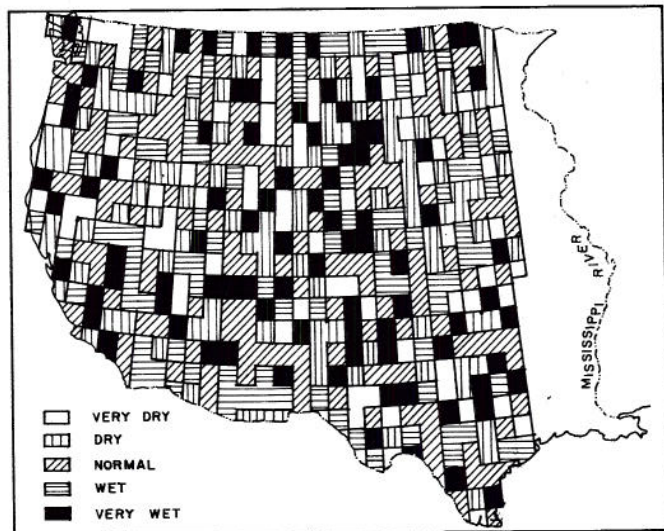
Fig. 18 Synoptic map of wet and dry years, as assigned to sub-areas of the Western United States, for a given year, obtained from the table of independent numbers.
