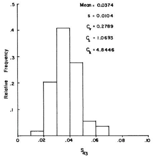
Fig. 21 Areal and frequency distributions of standard error of estimate S_{43} for Model I.
