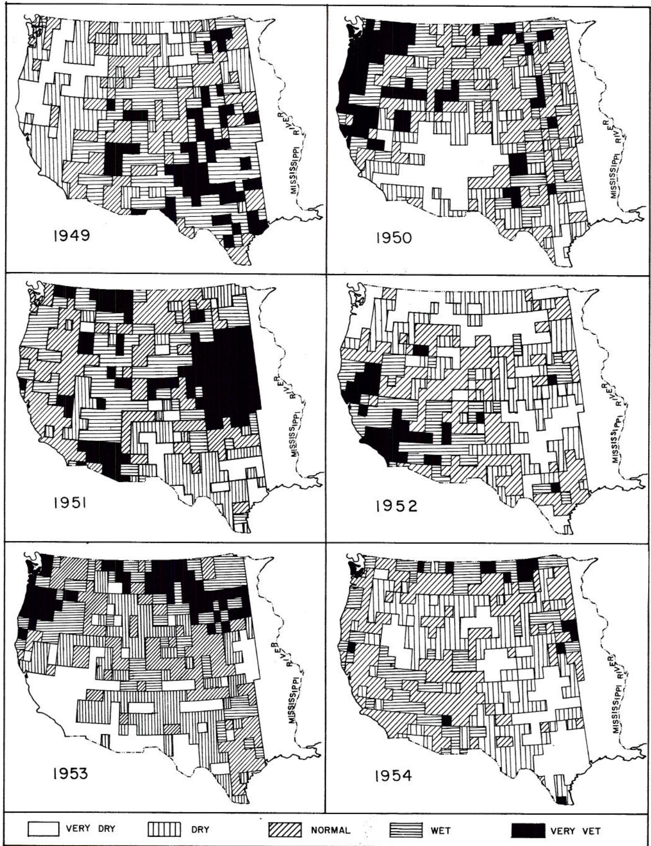
Fig. 7 Synoptic maps of wet and dry years in the Western United States for individual years during the period 1949 to 1954
