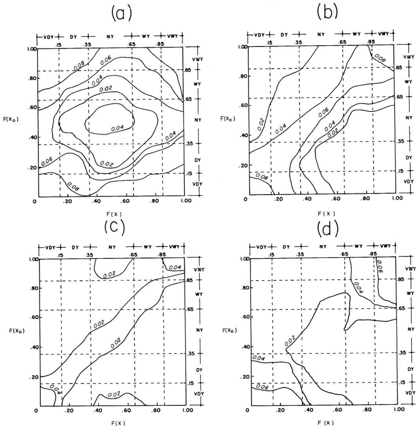
Fig. 35 Standard error of estimate of the four mathematical models as a function of F(x_0) and F(x) :
