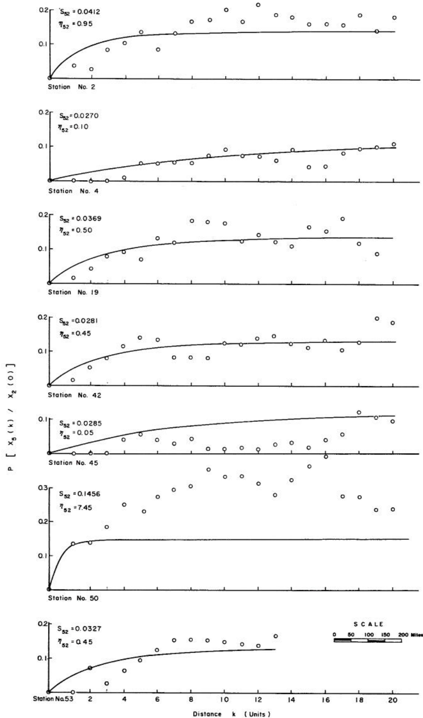
Fig. 30 Comparison of conditional probabilities of having a very wet year at the sub-areas at the distance k from the central sub-area, given a dry year at the central sub-area, with those of Model IV. Points are the computed conditional probabilities; the solid line represents Model IV.
