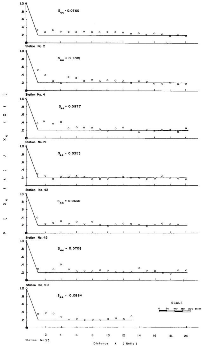
Fig. 13 Comparison of conditional probabilities of having a wet year at the sub-areas at the distance k from the central sub-area, given a wet year at the central sub-area, with those of Model I. Points are the computed conditional probabilities; the solid line represents Model I
