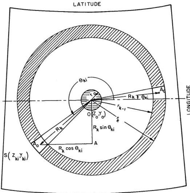
Fig. 40 Circular grid system used for computation of conditional probabilities of wet and dry years as a function of distance, by the use of the first method.
