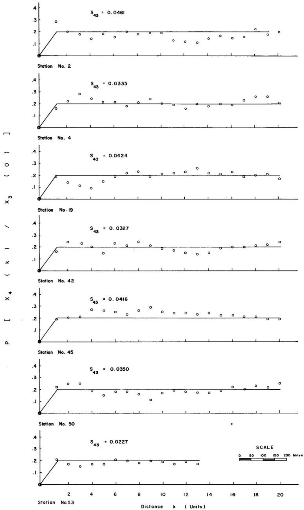
Fig. 14 Comparison of conditional probabilities of having a wet year at the sub-areas at the distance k from the central sub-area, given a normal year at the central sub-area, with those of Model I. Points are the computed conditional probabilities: the solid line represents Model I.
