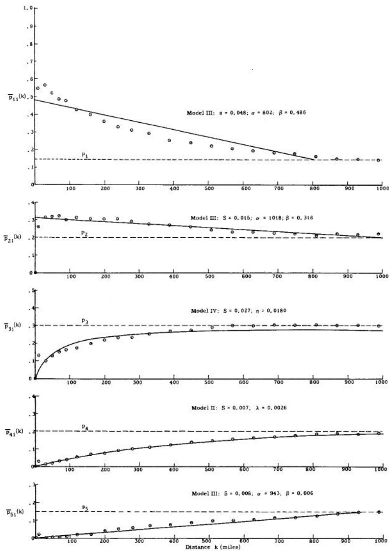
Fig. 39 Five cases of mean conditional probabilities, \bar{p}_{ij}(k) , fitted by the recommended mathematical models.
