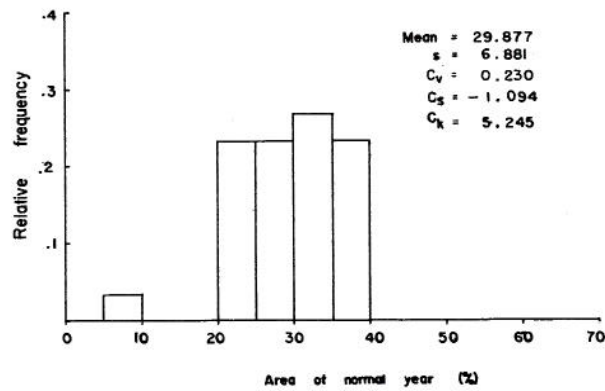
Fig. 10 Frequency distributions of percent of areas in the Western United States having very dry, dry, normal, wet and very wet years
