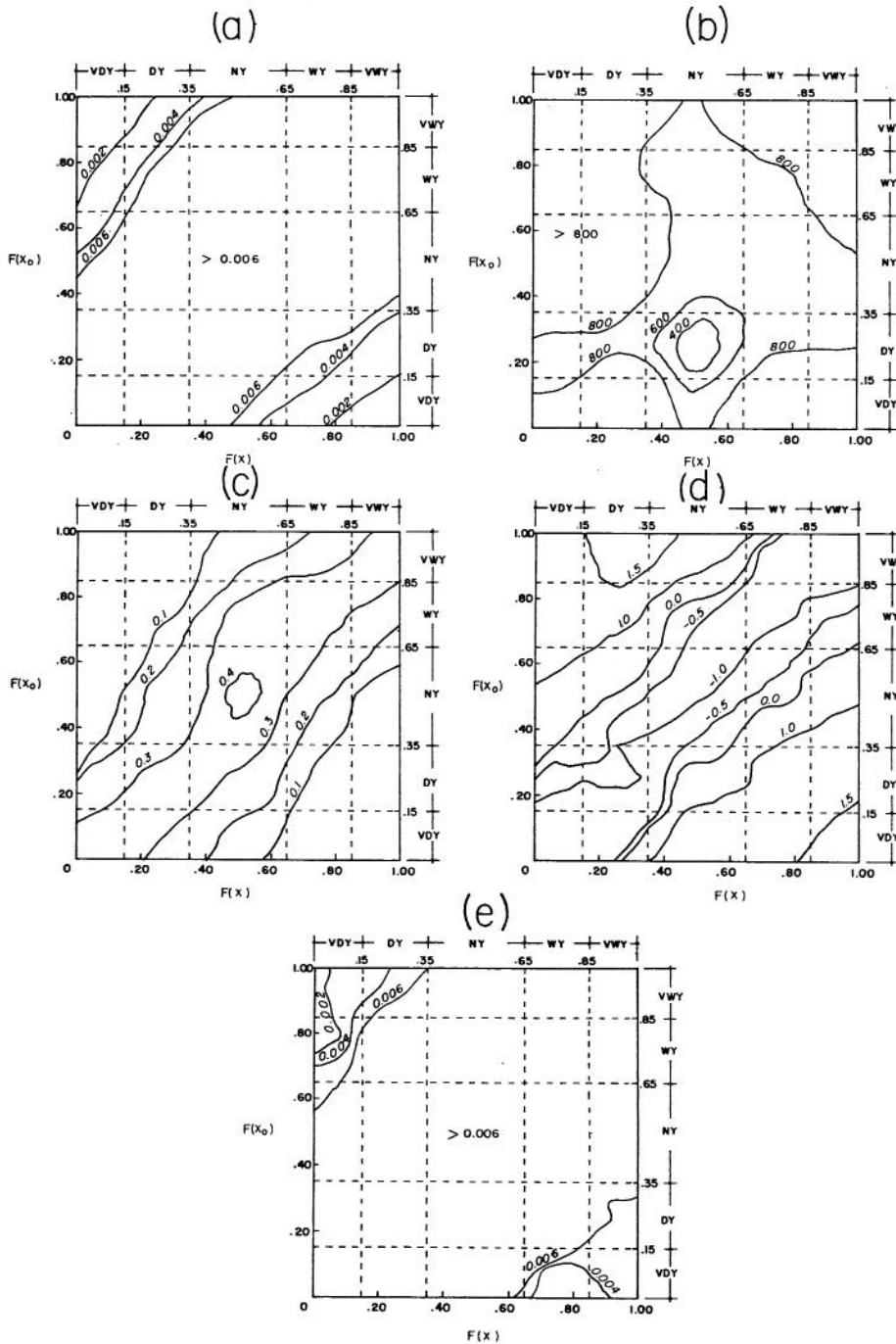
Fig. 36 Parameters of the four mathematical models as a function of F(x_0) and F(x) : (a) Model II, \lambda_{ij} ; (b) Model III, \alpha_{ij} ; (c) Model III, \beta_{ij} ; (d) Model III, \nu_{ij} ; and (e) Model IV, \eta_{ij} .
