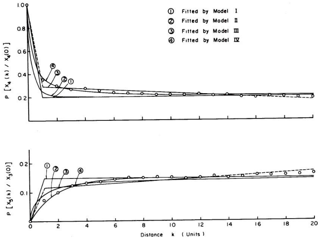
Fig. 31 Comparison of mean conditional probabilities of wet and dry years, \bar{p}_{ij}(k) , with those of Models I, II, III and IV. Points are the computed mean conditional probabilities: the solid lines represent Models I through IV.
