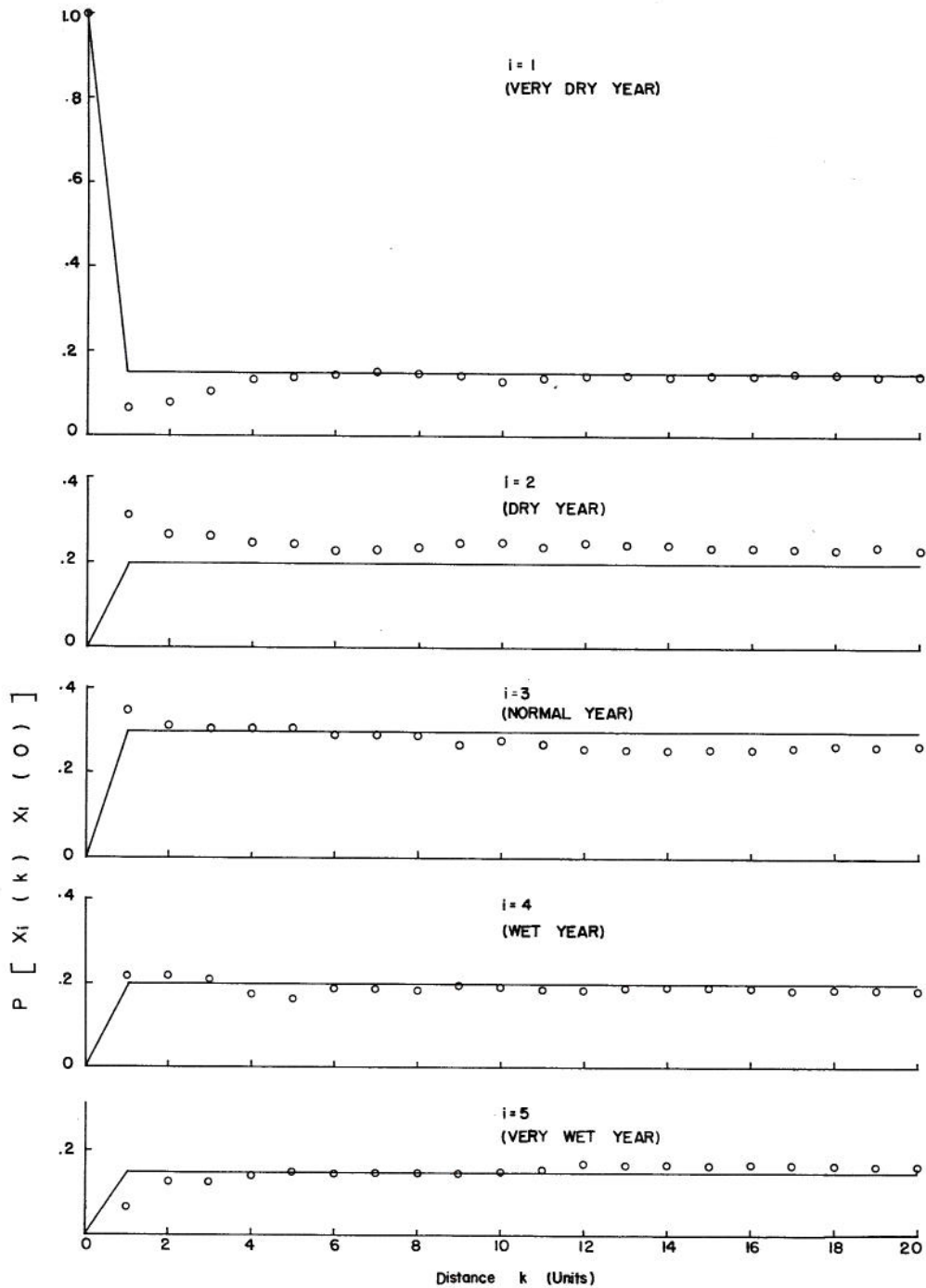
Fig. 19 Conditional probabilities of wet and dry years as a function of distance computed from the table of independent numbers
