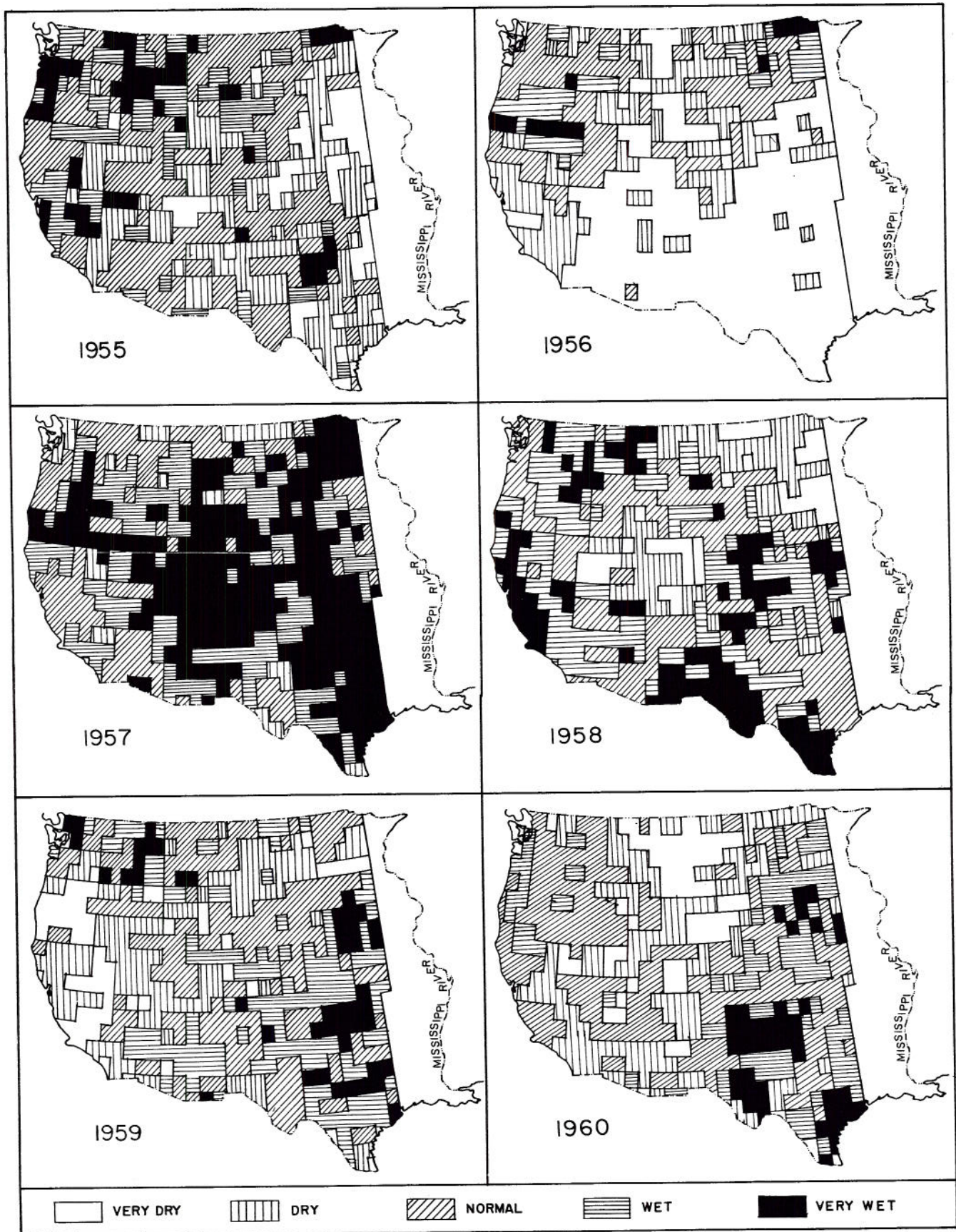
Fig. 8 Synoptic maps of wet and dry years in the Western United States for individual years during the period 1955 to 1960
