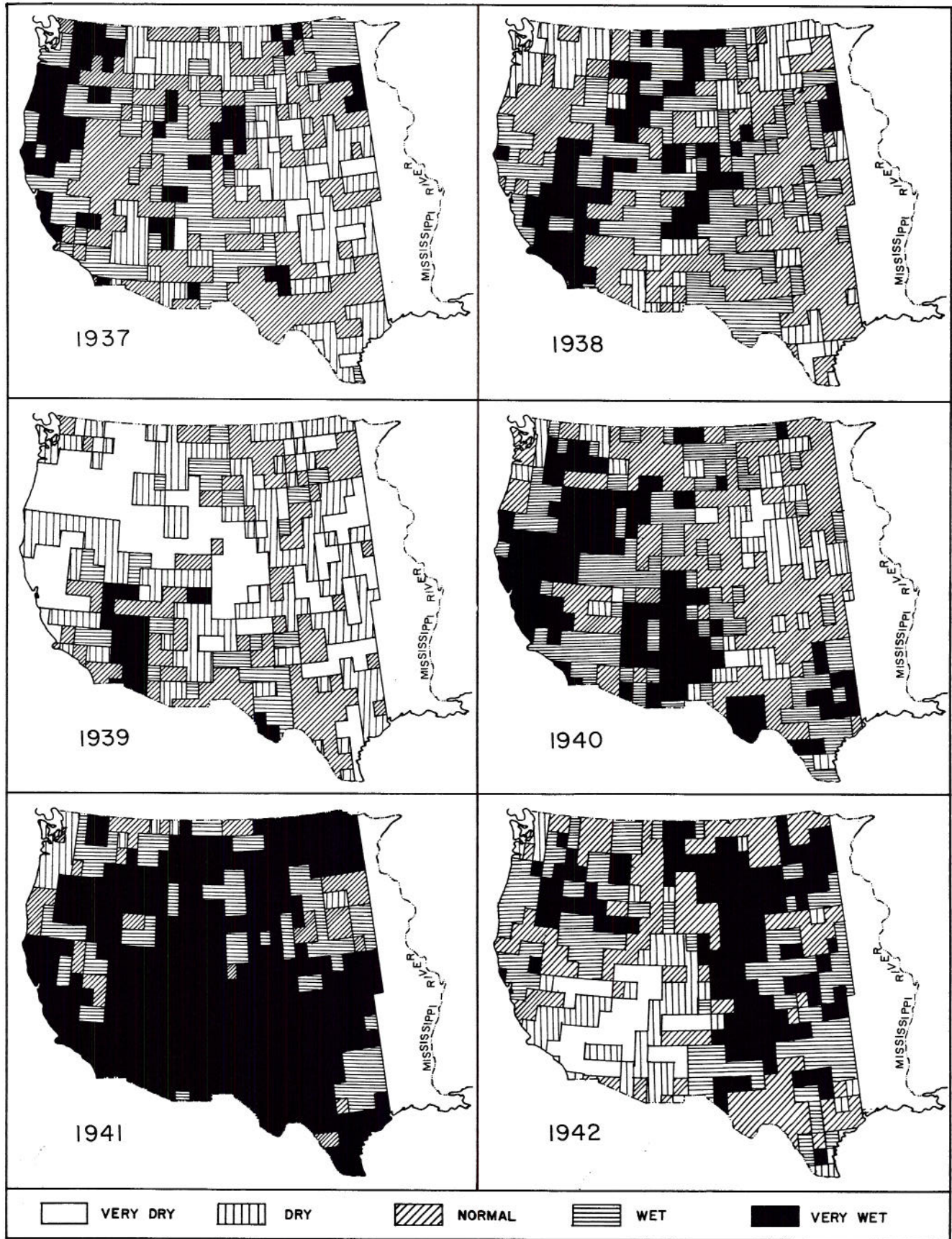
Fig. 5 Synoptic maps of wet and dry years in the Western United States for individual years during the period 1937 to 1942
