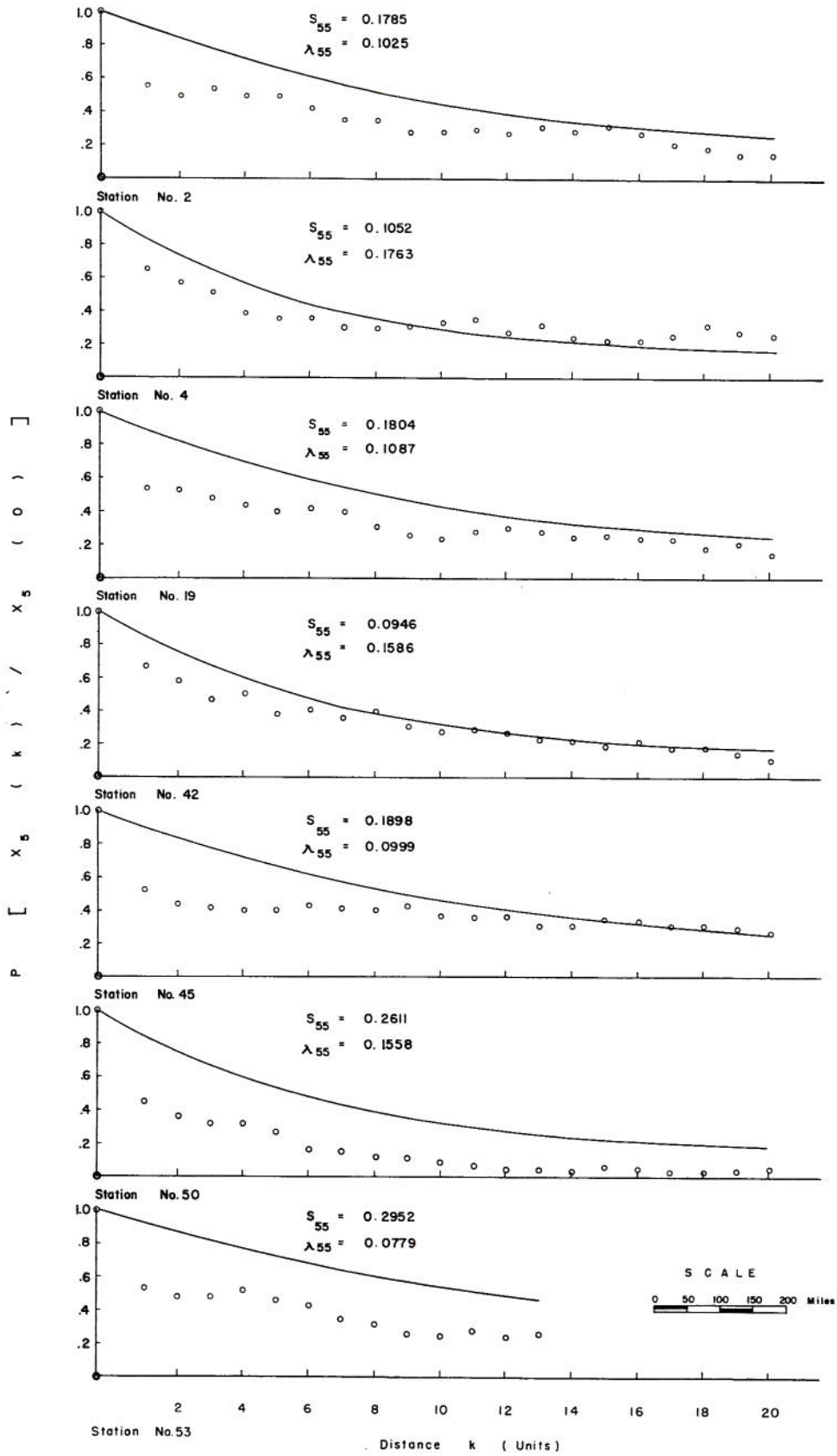
Fig. 15 Comparison of conditional probabilities of having a very wet year at the sub-areas at the distance k from the central sub-area, given a very wet year at the central sub-area, with those of Model II. Points are the computed conditional probabilities; the solid line represents Model II.
