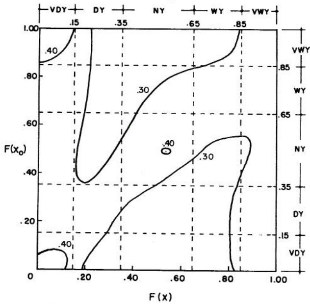
Fig. 23 Coefficient of variation, C_v , of the standard error of estimate, S_{ij} , as a function of F(x_0) and F(x) : (a) Model I; (b) Model II; (c) Model III; and (d) Model IV.
