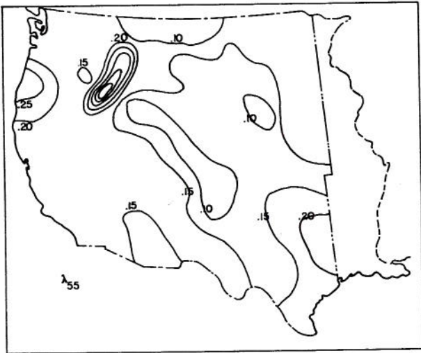
Fig. 24 Areal and frequency distributions of standard error of estimate, S_{55} , and of parameter \lambda_{55} for Model II.
