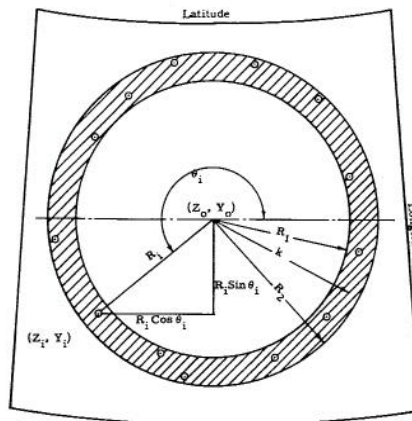
Fig. 41 Circular grid system used for computation of conditional probabilities of wet and dry years as a function of distance, by the use of the second method.
