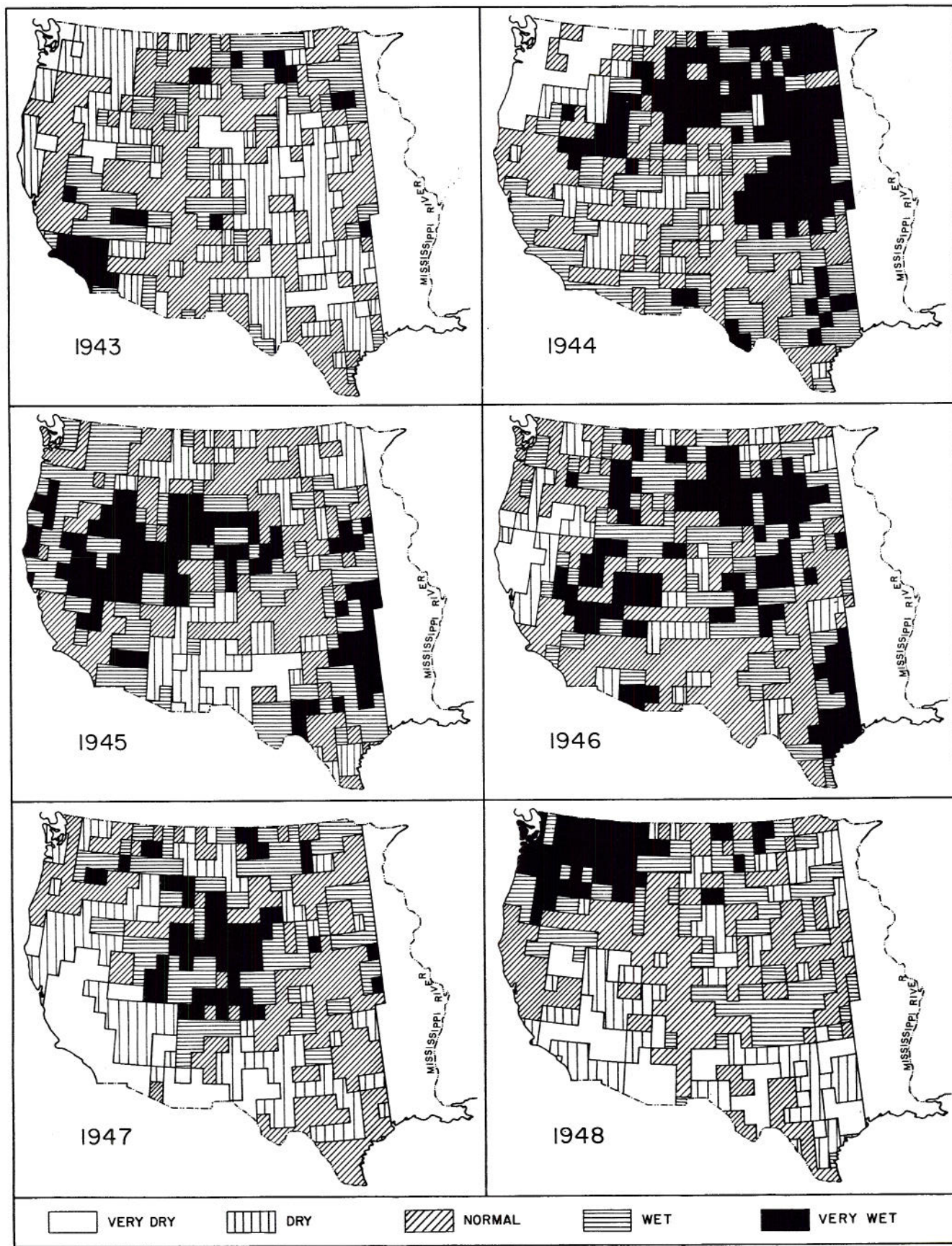
Fig. 6 Synoptic maps of wet and dry years in the Western United States for individual years during the period 1943 to 1948
