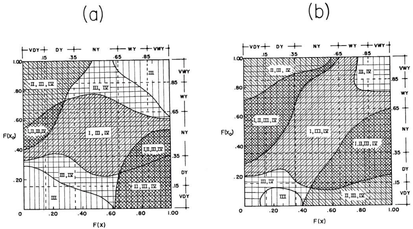
Fig. 32 Comparison of the goodness of fit of Models I, II, III and IV with various values of mean standard error of estimate being a function of F(x_0) and F(x) : (a) \bar{S}_{ij} \leq 0.06 ; (b) \bar{S}_{ij} \leq 0.08 .
