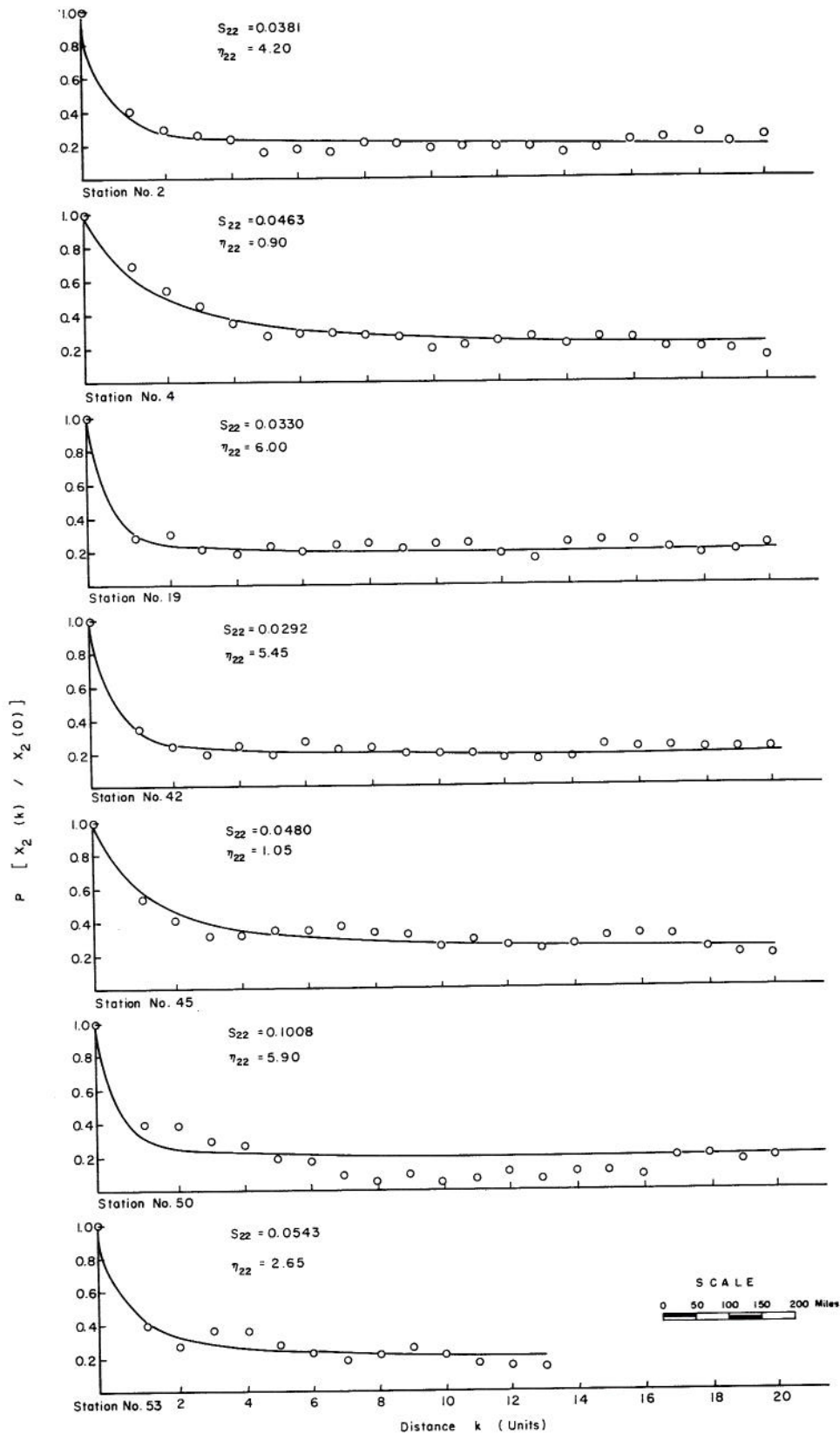
Fig. 29 Comparison of conditional probabilities of having a dry year at the sub-areas at the distance k from the central sub-area, given a dry year at the central sub-area, with those of Model IV. Points are the computed conditional probabilities: the solid line represents Model IV.
