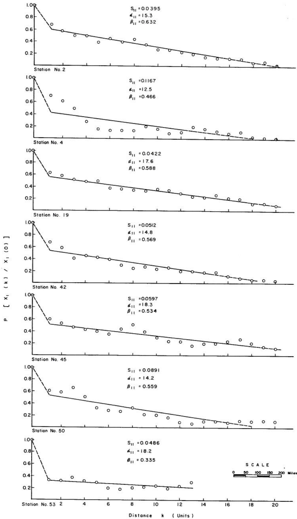
Fig. 27 Comparison of conditional probabilities of having a very dry year at the sub-areas at the distance k from the central sub-area, given a very dry year at the central sub-area, with those of Model III. Points are the computed conditional probabilities: the solid line represents Model III.
