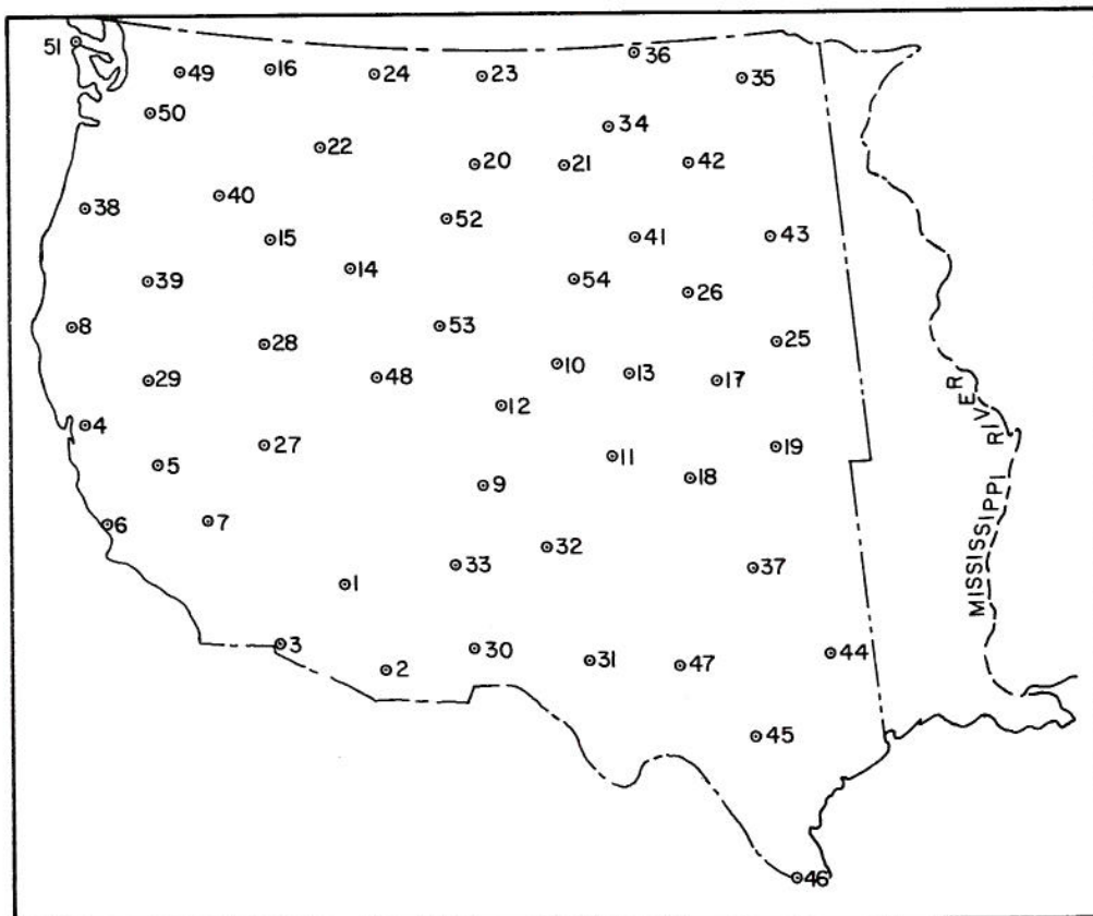
Fig. 12 Locations of central sub-area centers in the Western United States
