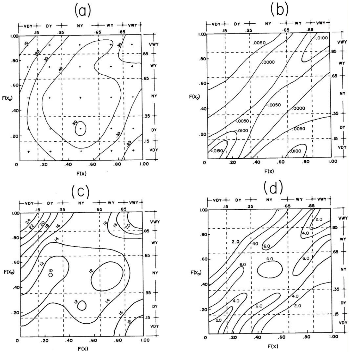
Fig. 26 Means or medians of parameters of mathematical models as functions of F(x_0) and F(x) : (a) Model II, \bar{\lambda}_{ij} ; (b) Model III, median of \nu_{ij} ; (c) Model III, median of \alpha_{ij} ; and (d) Model IV, \bar{\eta}_{ij} .
