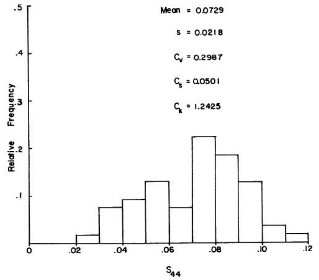
Fig. 20 Areal and frequency distributions of standard error of estimate S_{44} for Model I.
