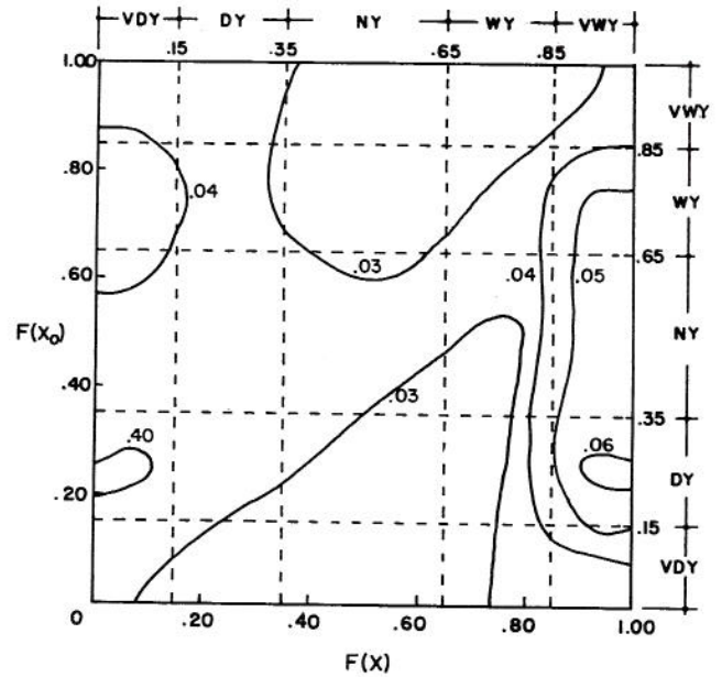
Fig. 23 Coefficient of variation, C_v , of the standard error of estimate, S_{ij} , as a function of F(x_0) and F(x) : (a) Model I; (b) Model II; (c) Model III; and (d) Model IV.
