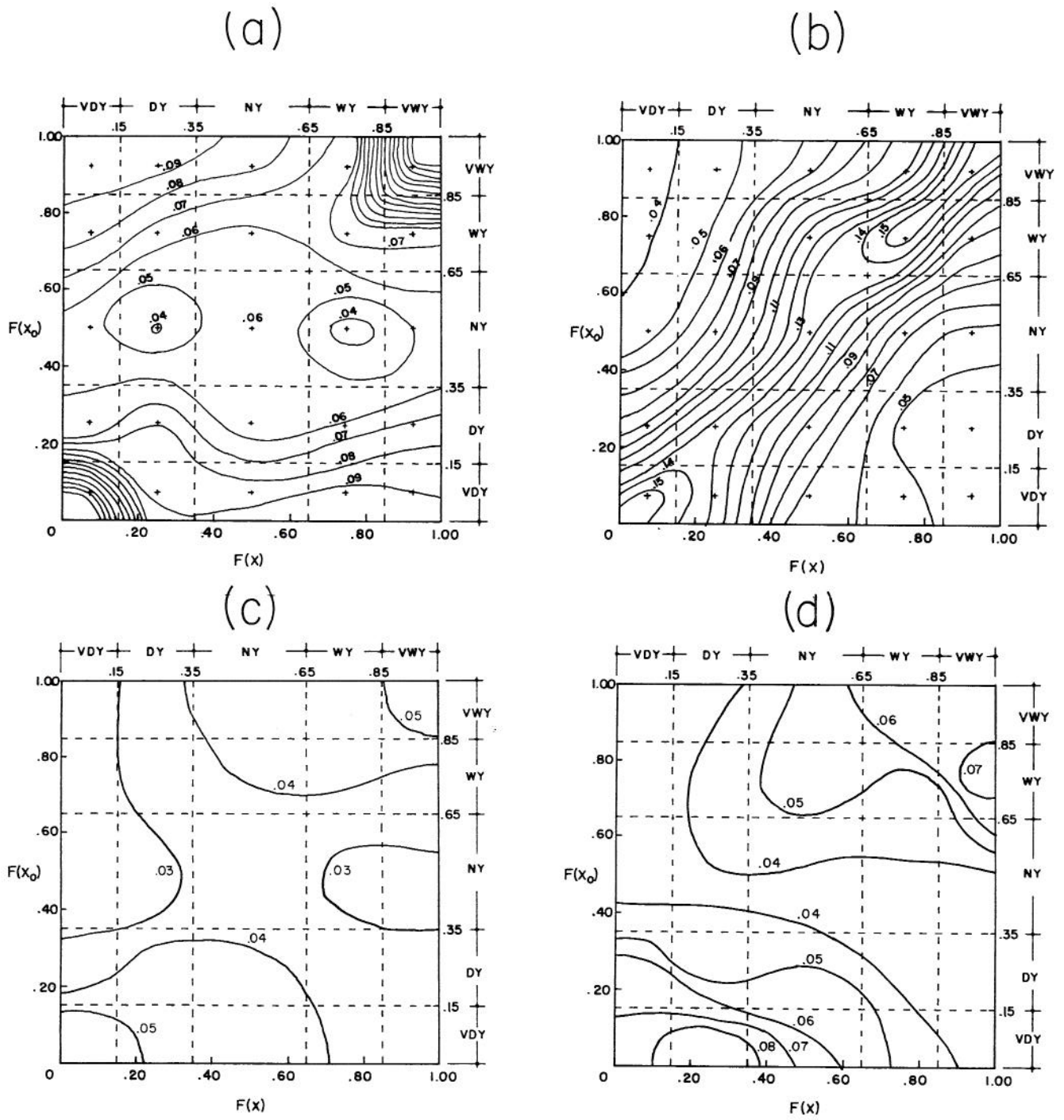
Fig. 22 Mean standard error of estimate, \bar{S}_{ij} , as a function of F(x_0) and F(x) : (a) Model I; (b) Model II; (c) Model III; and (d) Model IV
