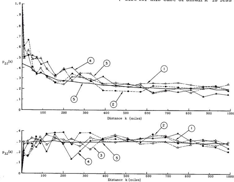
Fig. 33 Conditional probabilities of a dry year (upper graph) and a normal year (lower graph) at the distance k , given a dry year at a central station: (1) central station, Seward, Nebraska; (2) central station, Utica, Nebraska; (3) central station, Acton Escondido, California; (4) central station, Riverside Fire Station No. 3, California; and (5) Average conditional probabilities for all 1141 precipitation stations used in this study.
