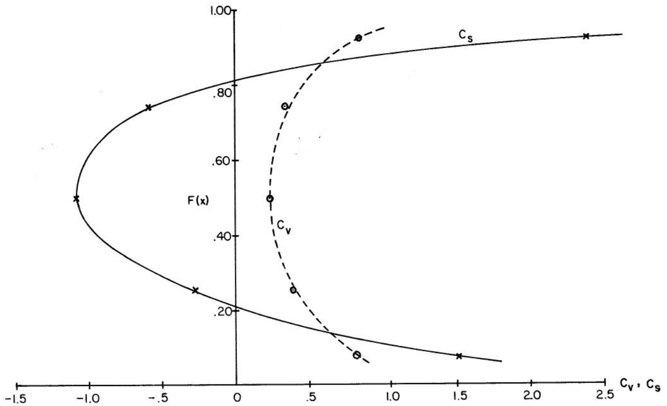
Fig. 11 Relationship among coefficients of variation, skewness coefficients and types of wet and dry years
