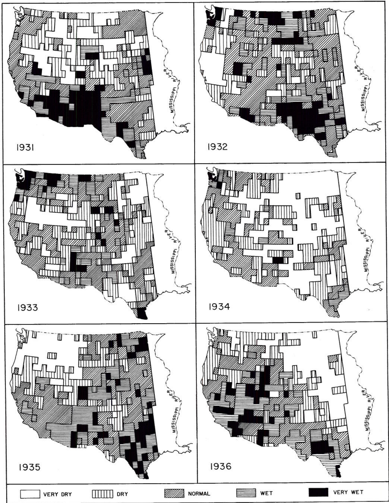
Fig. 4 Synoptic maps of wet and dry years in the Western United States for individual years during the period 1931 to 1960
