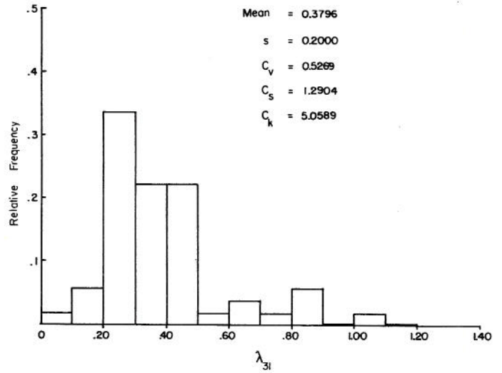
Fig. 25 Areal and frequency distributions of standard error of estimate, S_{31} , and of parameter \lambda_{31} for Model II.
