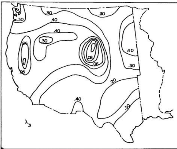
Fig. 25 Areal and frequency distributions of standard error of estimate, S_{31} , and of parameter \lambda_{31} for Model II.
