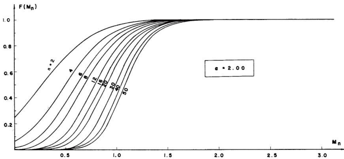
Fig. 3.18 Distribution functions of maximum surplus, F(M_n) , for \alpha = 2.00 and various values of n
