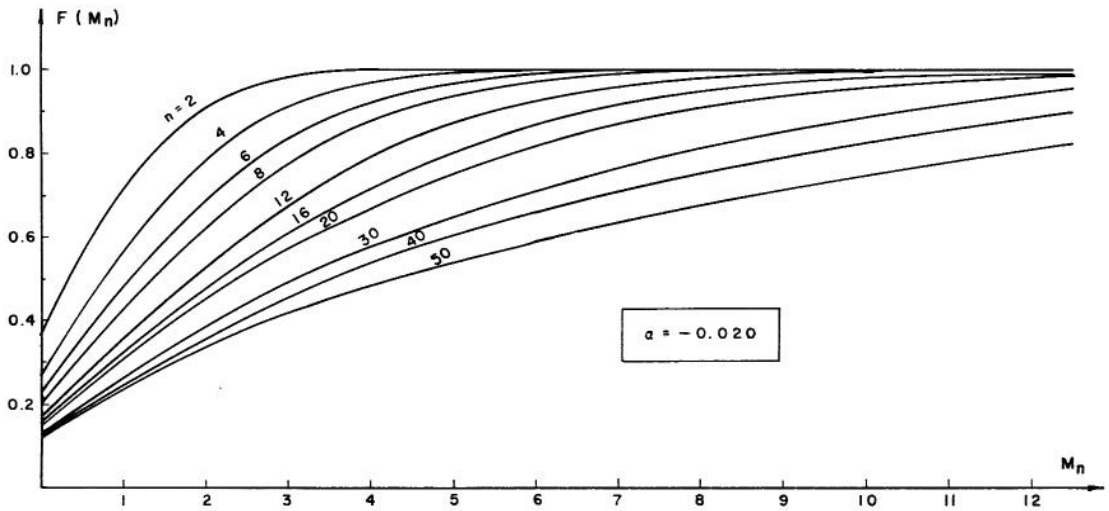
Fig. 3.11 Distribution functions of maximum surplus, F(M_n) , for \alpha = -0.020 and various values of n
