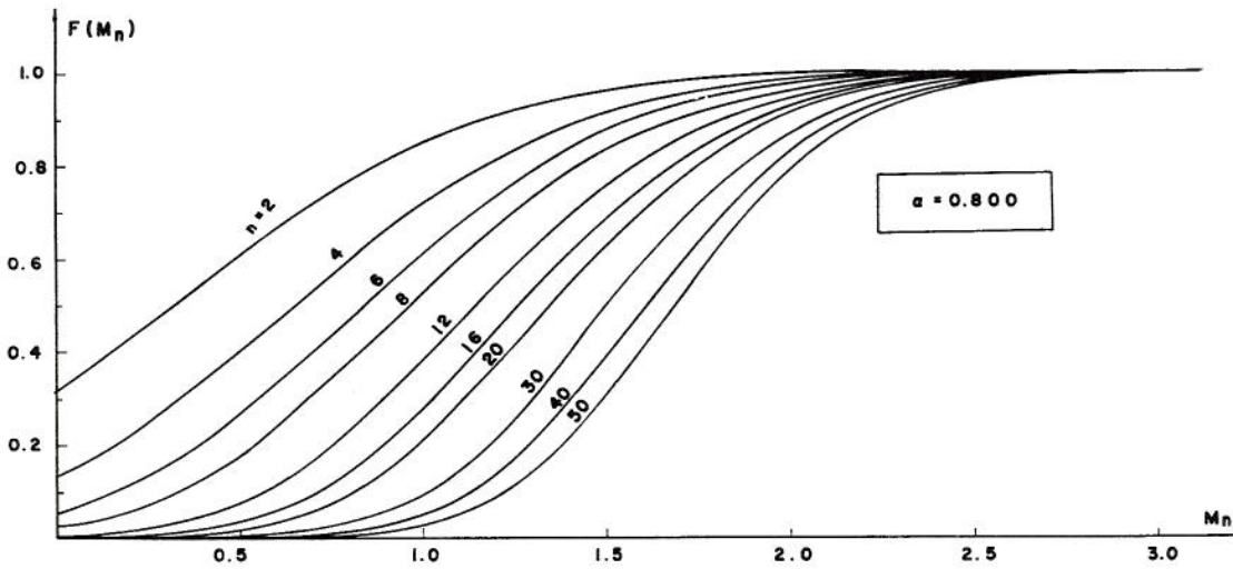
Fig. 3.17 Distribution functions of maximum surplus, F(M_n) , for \alpha = 0.800 and various values of n
