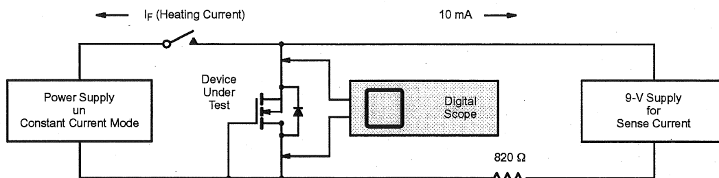
FIGURE 2. Connection Diagram
