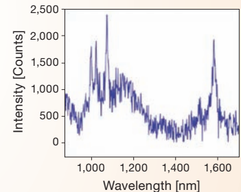
(Left) Configuration used to collect signal from the surface-enhanced Raman scattering (SERS) fiber probe. The spectrometer measures the SERS signal from analytes interacting with optical antennas transferred to a fiber facet (inset). (Right) Benzenethiol remotely detected through its SERS spectrum measured with the fiber sensor.
