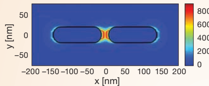
(Left) Numerical simulation of the optical intensity enhancement with respect to the incident intensity at \lambda_0=0.83\text{ }\mu\text{m} . (Right) Map of optical intensity enhancement for a bow-tie optical antenna designed for a vertical-cavity surface-emitting laser emitting at \lambda_0=0.85\text{ }\mu\text{m} .
