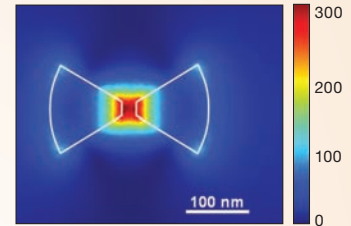
(Left) Numerical simulation of the optical intensity enhancement with respect to the incident intensity at \lambda_0=0.83\text{ }\mu\text{m} . (Right) Map of optical intensity enhancement for a bow-tie optical antenna designed for a vertical-cavity surface-emitting laser emitting at \lambda_0=0.85\text{ }\mu\text{m} .
